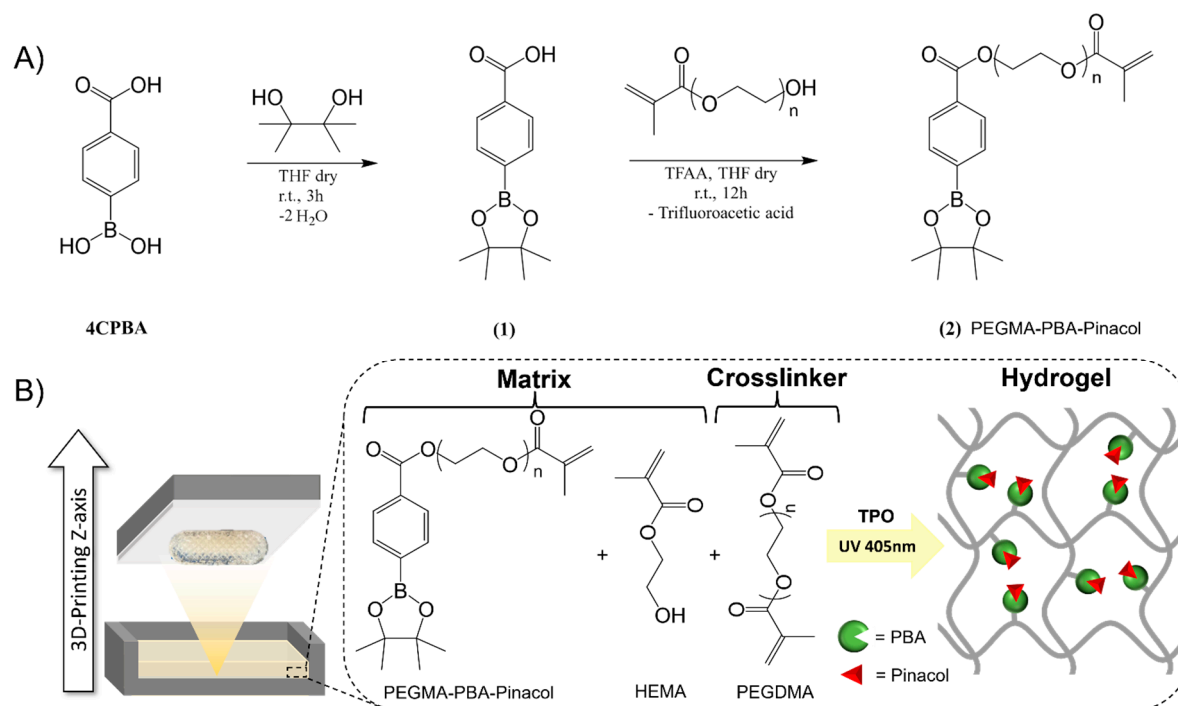
Figure 1. A) Synthetic route of \alpha -methacrylate \omega -pinacolyl boronic ester poly(ethylene glycol) (PEGMA-PBA-Pinacol, i.e. compound 2). B) Fast bottom-up fabrication of PBA-containing hydrogels via photopolymerization of HEMA and PEGMA-PBA-Pinacol using PEGDMA crosslinker and TPO photo-initiator.
