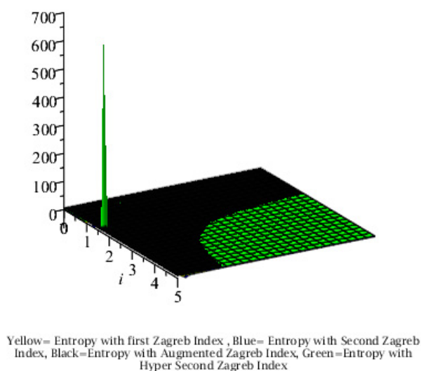
Figure 6. Comparison of Entropies for cu_2o[i, j, t] \geq 2 .
