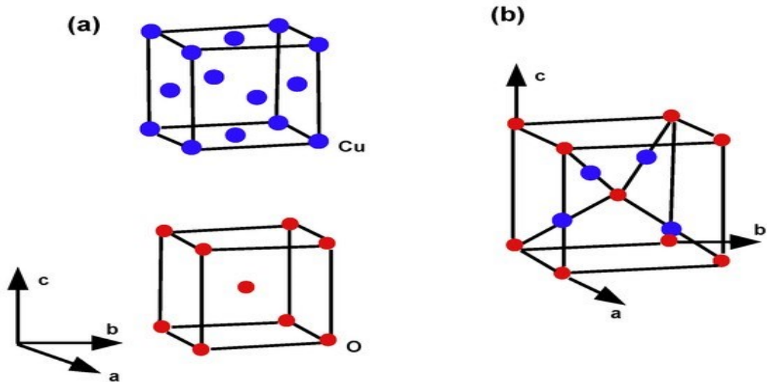
Structure of the crystallographic molecule Cu_2O (a) Cu and O structural features atoms in the lattice of Cu_2O . The lattice of Cu_2O is formed by interpenetrating the lattices of Cu and O with The other one. (b) Cu_2O Unit Cell. As small blue spheres, copper atoms are seen, and oxygen atoms they're seen as big red spheres. Each Cu atom is coordinated in the Cu_2O lattice with two O atoms and each atom of O is coordinated by four atoms of Cu.
