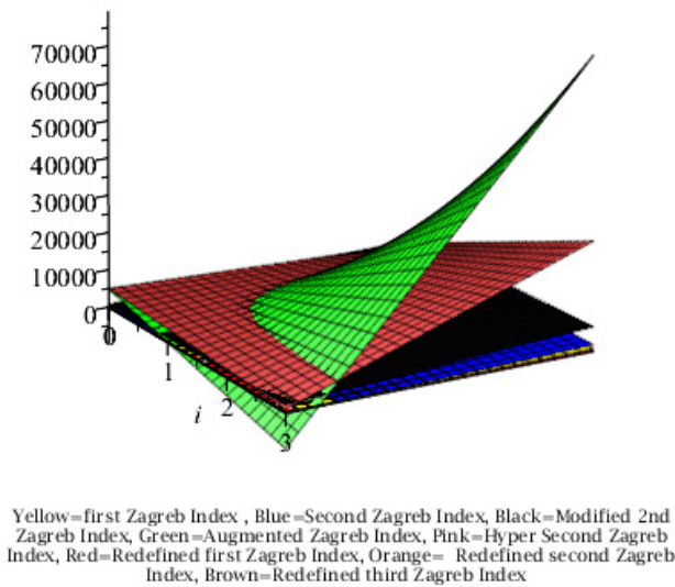
Figure 4. Comparison of Topological Indices for cu_2o[i, j, t] \geq 2 .
