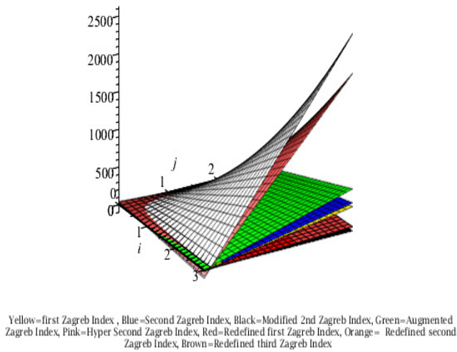
Figure 3. Comparison of Topological Indices for cu_2o[i, j, t] \geq 1 .
