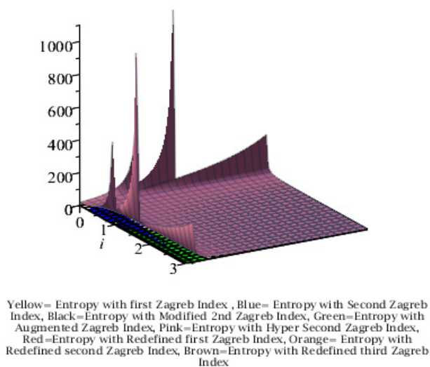
Figure 5. Comparison of Entropies for cu_2o[i, j, t] \geq 1 .
