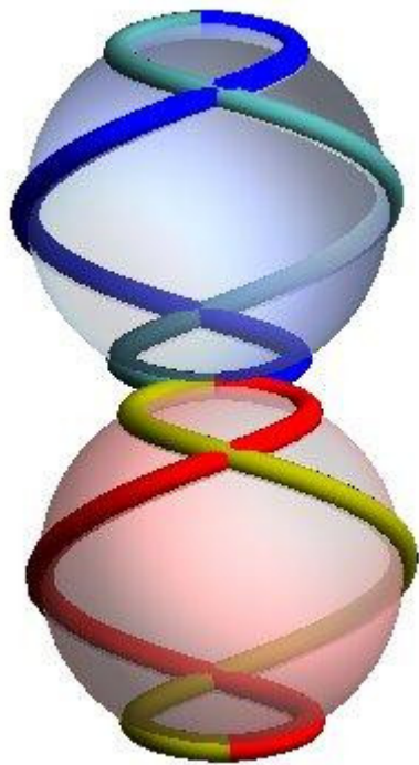
Figure 2. Aether Unit viewed in five dimensions of space resonance.
