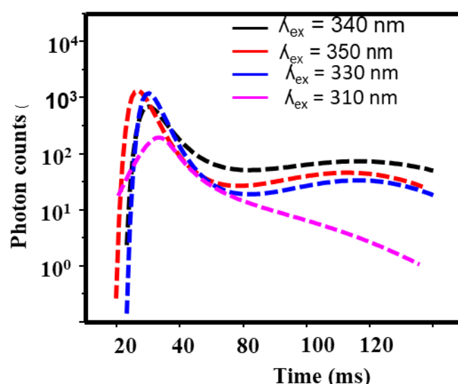
Figure 7. C-dot decay curves obtained at an excitation wavelength of each individual maximum intensity.
