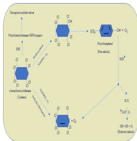
Figure 5: Pathway of organochlorine metabolism and free radicals generation.
