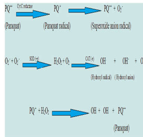
Figure 6: Reactions leading to the generation of herbicide (paraquat) radicals.
