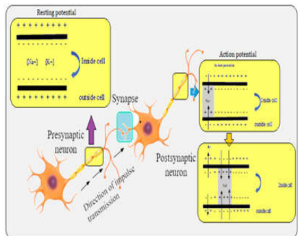
Figure 4: Mode of action of pyrethroid insecticides on sodium gated channel.
