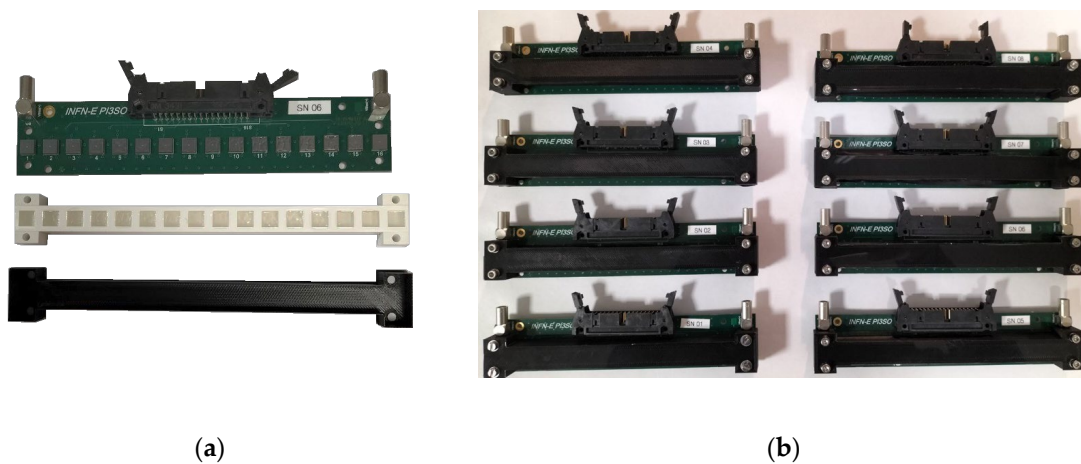
Figure 4. (a) Real view of the detector group components: the electronic board hosting 16 SiPMs, the 16 scintillators encased in white reflective resin, the black external light shield. (b) The 8 detector groups assembled and ready to be installed on the sliding bridge.
