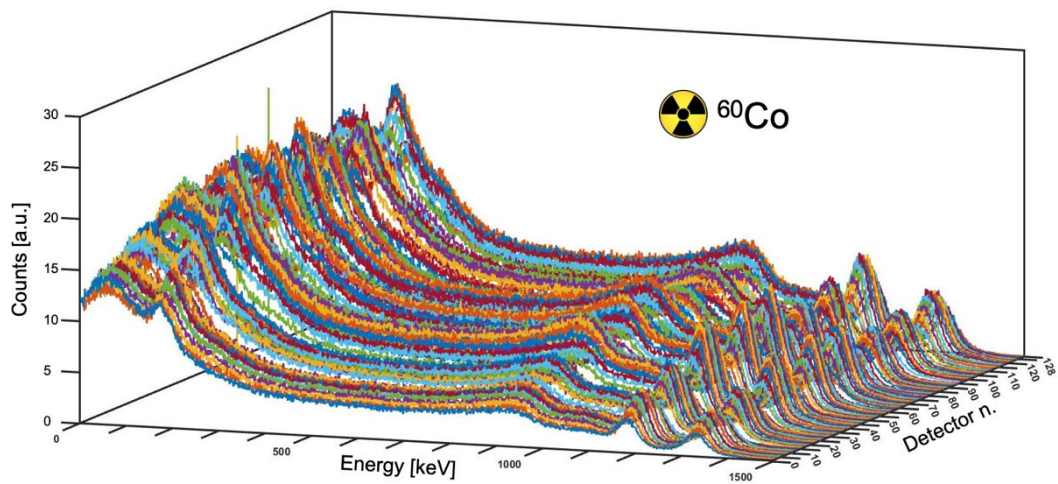
Figure 11. 128 calibrated spectra obtained with the ^{60}\text{Co} source in the arrangement of Figure 7.
