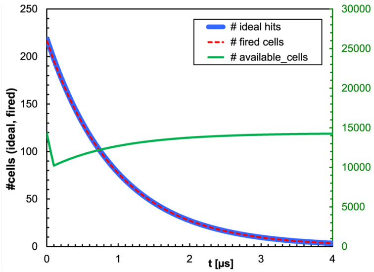
Figure 5. Calculation of the time evolution of the SiPM response under the assumption of 2 MeV deposited into the crystal and all the scintillation light conveyed onto the SiPM. See text for details.
