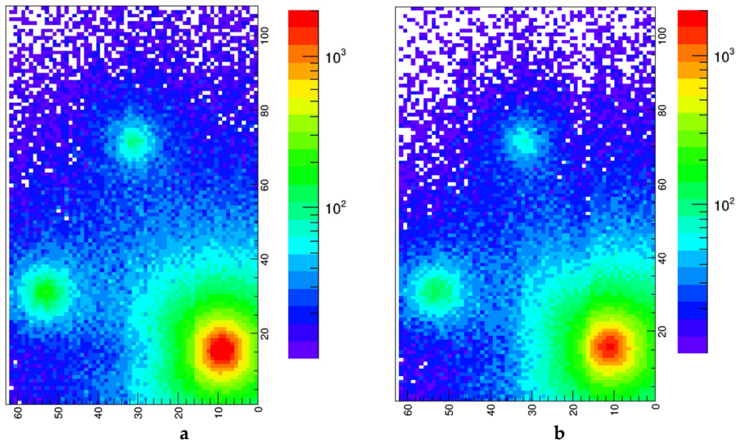
Figure 19. Result of the 1.5 minute gamma scan. (a) Top view. (b) Bottom view.
