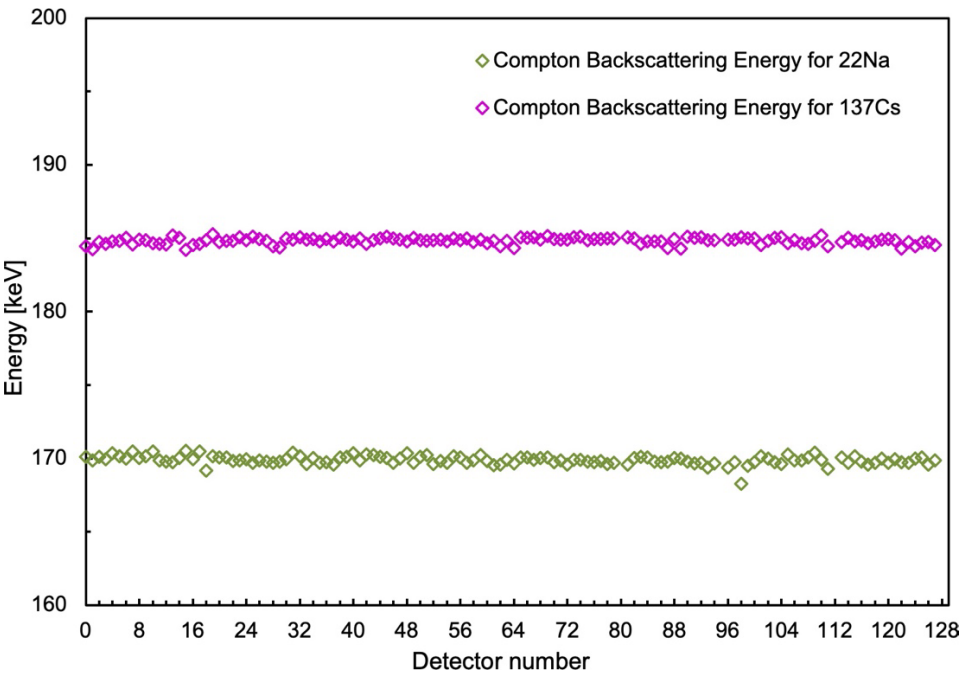
Figure 9. Energy calibration cross check for the 128 detectors: the resulting centroid energy of the Compton backscattering peak for the 511 and 662 keV gamma rays, expected at 170 and 184 keV respectively, as a function of the detector number.
