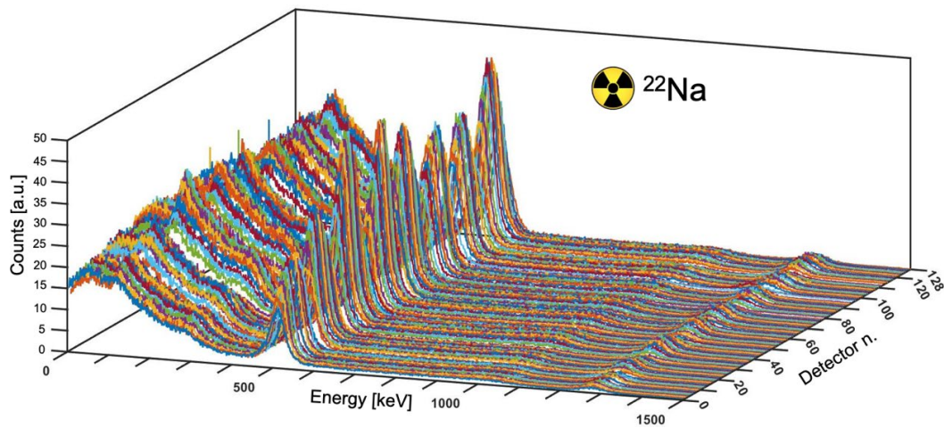
Figure 10. 128 calibrated spectra obtained with the ^{22}\text{Na} source in the arrangement of Figure 7.
