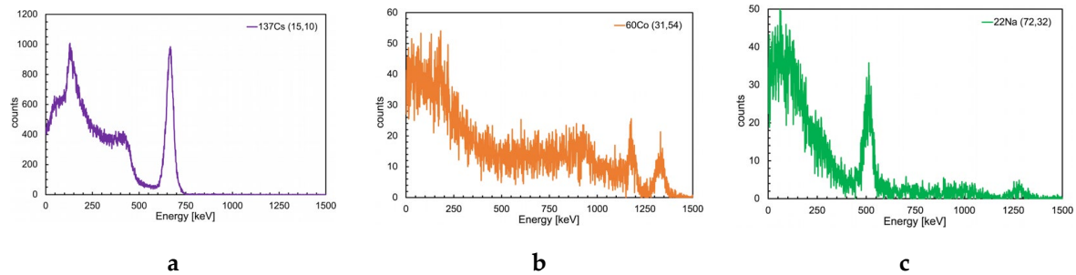
Figure 15. Spectra from three dedicated one-minute data acquisitions on the three detected hot spots. (a) ^{137}\text{Cs} . (b) ^{60}\text{Co} . (c) ^{22}\text{Na} .
