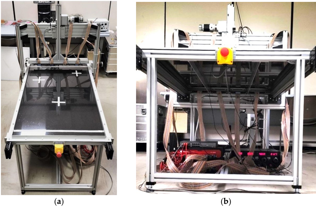
Figure 1. (a) Top and (b) bottom views of the PI3SO gamma-ray scanner table. 4+4 ribbon cables for the signals from the 128 detectors are visible, along with the data acquisition and power supply electronics installed under the table.
