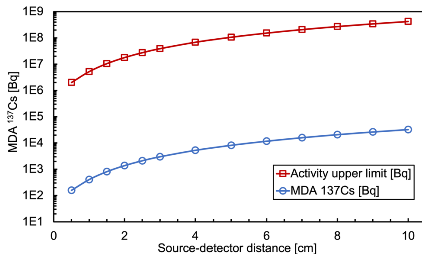
Figure 24. Operational range of a 1 cm 3 CsI(Tl) detector, between Minimum Detectable Activity and activity upper limit, as a function of its distance from a pointlike 137 Cs source.
