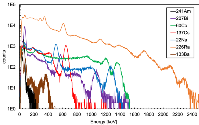
Figure 6. Calibrated spectra of seven different gamma sources obtained with a single detector [17].
