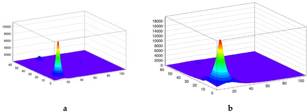
Figure 17. (a) Top view plot for the scan with the lead plate, in linear scale in a fancy 3D representation. (b) Bottom view plot for the same scan, obviously unaffected by the lead plate.
