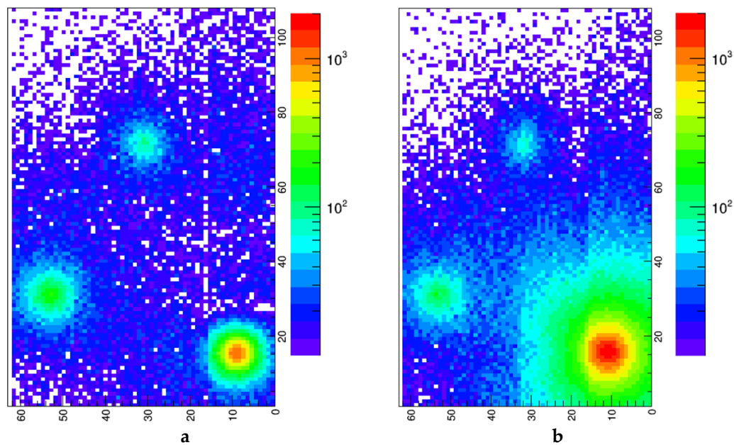
Figure 20. Result of the 1.5 minute gamma scan with the lead plate on the ^{137}\text{Cs} source. (a) Top view. (b) Bottom view.
