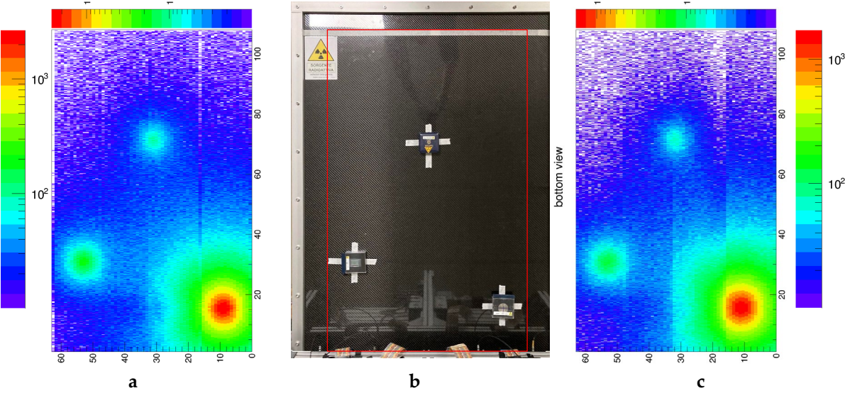
Figure 14. (a) Result of the gamma scan with the three sources, top view. (b) The three sources placed on the table. (c) Result of the gamma scan with the three sources, bottom view.
