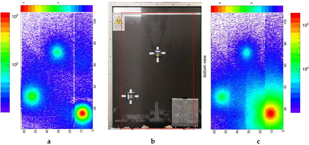
Figure 16. Result of the gamma scan with the three sources and a lead plate (a) Top view. (b) The three sources placed on the table, the lead plate onto the ^{137}\text{Cs} source. (c) Bottom view.
