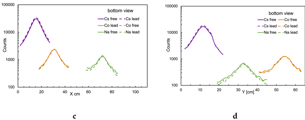
Figure 21. Plots of 1 cm wide slices cut on the maximum of each hot spot for the two scans with and without the lead plate on the ^{137}\text{Cs} source. (a) On the X direction, top view. (b) On the Y direction, top view. (c) On the X direction, bottom view. (d) On the Y direction, bottom view.
