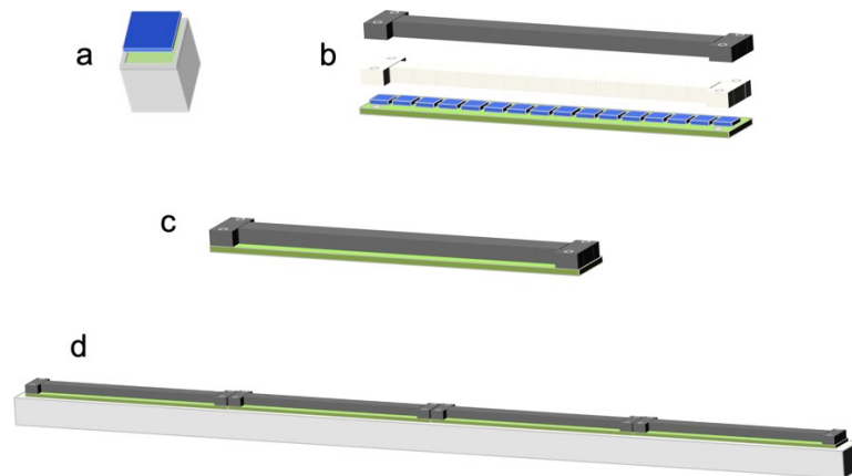
Figure 3. (a) Coupling of a SiPM (blue) with the CsI(Tl) crystal (green) surrounded by the reflective resin case (grey). (b) Exploded view of the electronic board hosting 16 SiPMs, the group of 16 scintillators, and the external light shield. (c) Assembled view of one group. (d) Sketch of one linear array made of four groups fixed on a support rod.
