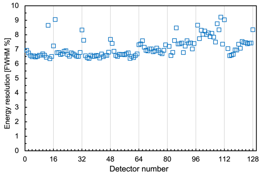
Figure 13. Energy resolution as a function of the detector number, determined as FWHM of the 662 keV peak of 137 Cs.
