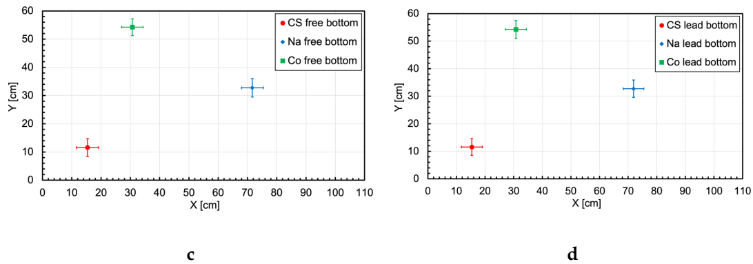
Figure 23. Positions of the detected hot spots with their error bars (data from Table 4). (a) Top view, no lead plate. (b) Top view, lead plate. (c) Bottom view, no lead plate. (d) Bottom view, lead plate.
