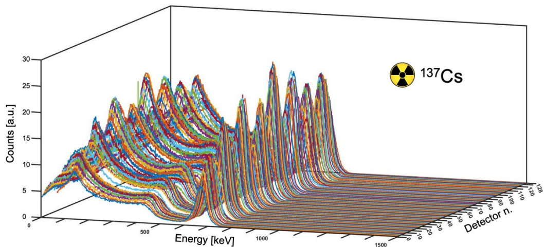
Figure 12. 128 calibrated spectra obtained with the ^{137}\text{Cs} source in the arrangement of Figure 7.
