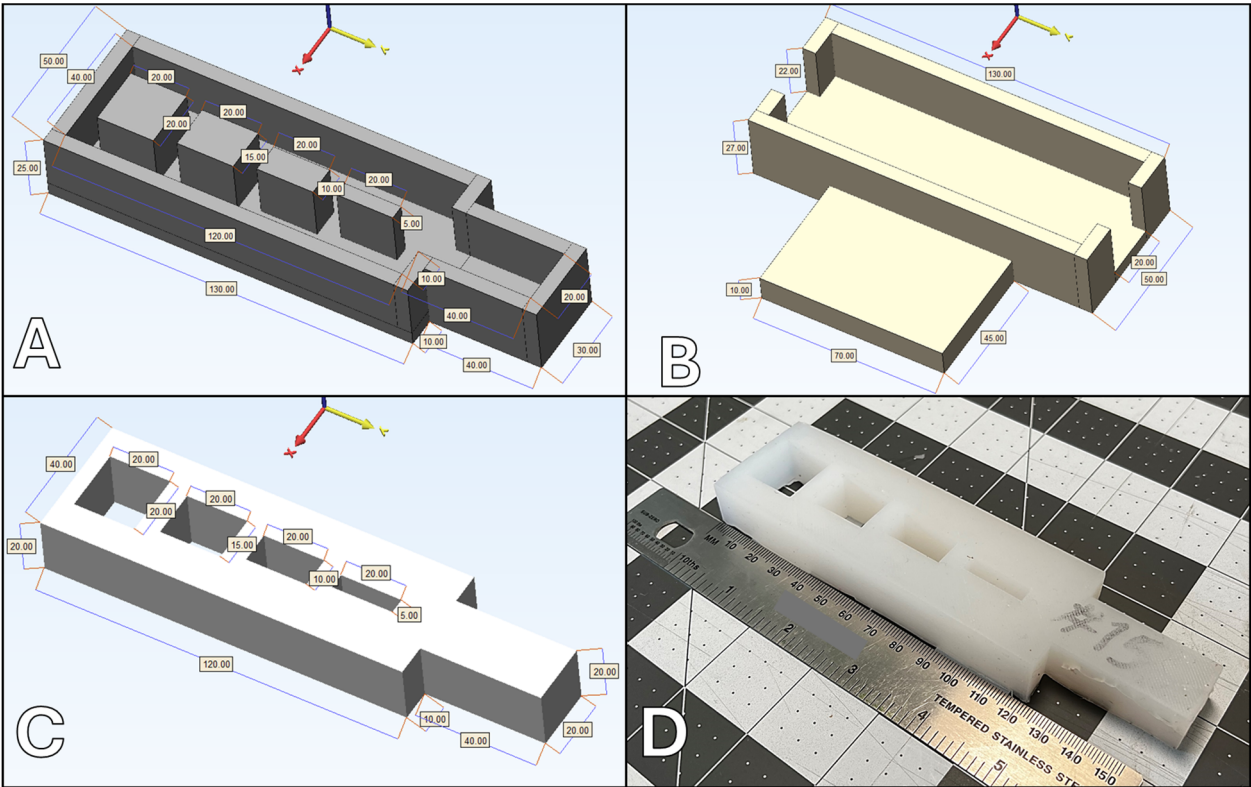
Figure 1. Silicone surrogate testing components. Surrogate mold (A), surrogate testing stand (B), and resultant surrogate sample (C/D). All measurement citations in millimeters.
