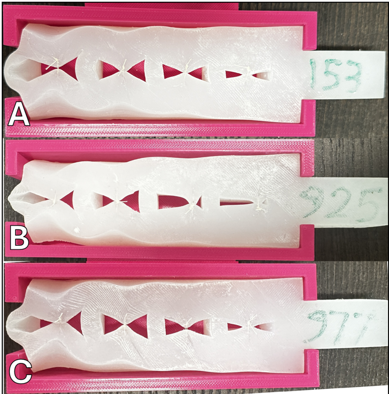
Figure 2. Top-performing surrogate samples following simulated surgical evaluation by expert surgeons. Sample 153 (A), Sample 925 (B), Sample 977 ©.
