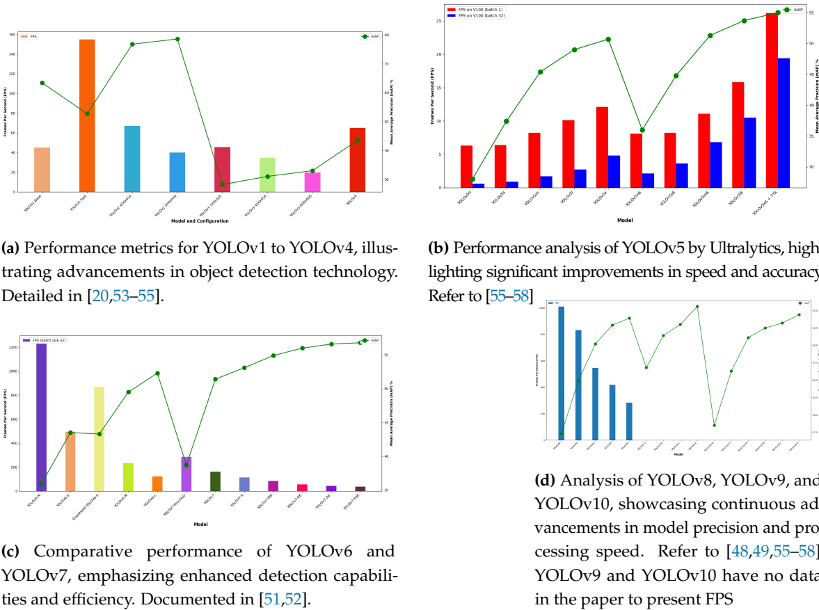
Figure 3. Comprehensive analysis of the performance metrics for YOLO versions. Subfigure (a) covers YOLOv1 to YOLOv4, (b) details YOLOv5, (c) compares YOLOv6 and YOLOv7, and (d) showcases YOLOv8, YOLOv9, and YOLOv10.
