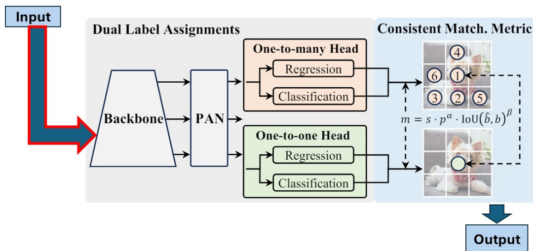
Figure 5. YOLOv10 architecture, which employs a dual label assignment strategy to improve detection accuracy. A backbone processes the input image, while PAN (Path Aggregation Network) enhances feature representation. Employed heads are (1) one-to-many head for regression and classification tasks, and (2) one-to-one head for precise localization [48]
