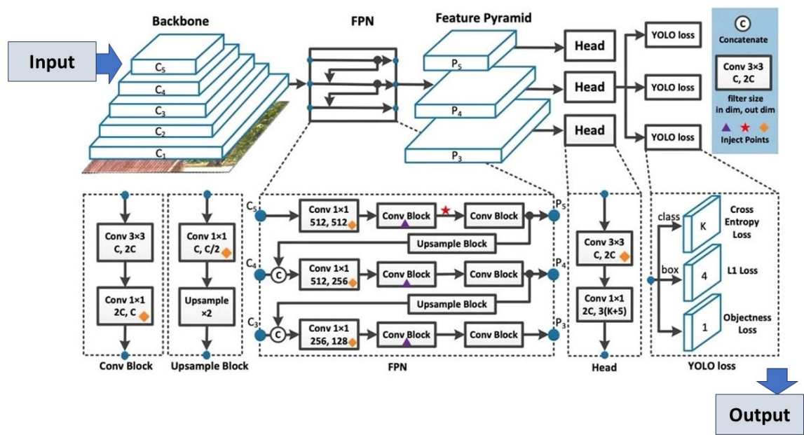
Figure 7. YOLOv8 architecture [79]: showcasing the key components and their connections. The backbone network processes the input image through multiple convolutional layers (C1 to C5), extracting hierarchical features. These features are then passed through the Feature Pyramid Network (FPN) to create a feature pyramid (P3, P4, P5), which enhances detection at different scales. The network heads perform final predictions, incorporating convolutional blocks and upsample blocks to refine features.
