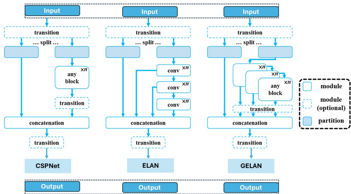
Figure 6. YOLOv9 architecture [49] with CSPNet, ELAN, and GELAN modules. CSPNet enhances gradient flow and reduces computational load through feature map partitioning. ELAN focuses on linear aggregation of features for improved learning efficiency, while GELAN generalizes this approach to combine features from multiple depths and pathways, providing greater flexibility and accuracy in feature extraction.
