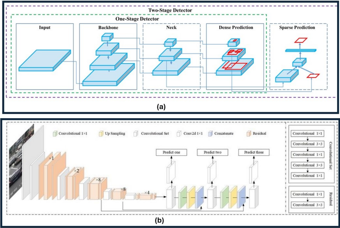
Figure 9. Comparison of YOLOv4 [55] and YOLOv3 [54] architectures. (a) YOLOv4 architecture showing a two-stage detector with backbone, neck, dense prediction, and sparse prediction modules. (b) YOLOv3 architecture featuring convolutional and upsampling layers leading to multi-scale predictions. This highlights the structural advancements in object detection between the two versions.
