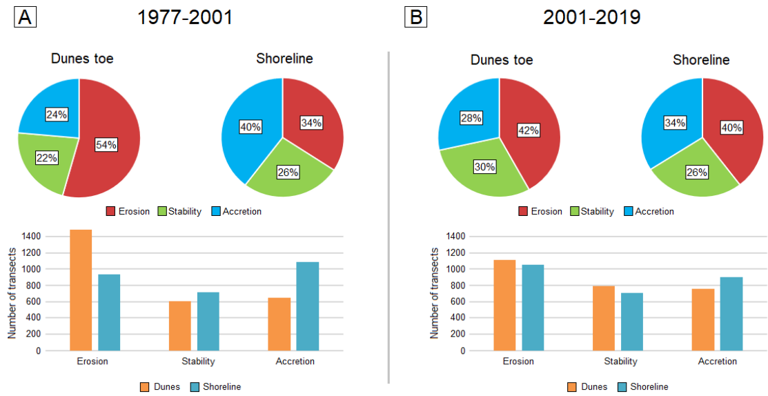
Figure 3. Rates of change of beach and foredune proxies for the 1977-2001 (A) and 2001-2019 (B) periods. Pie charts (upper figures) represent the percentages of change rates for foredunes and shorelines. Bar graph (lower figures) present the number of transects recording erosion, stability and accretion per each studied proxies, i.e. dune toe in the case of foredunes and the wet-dry line for the shoreline.
