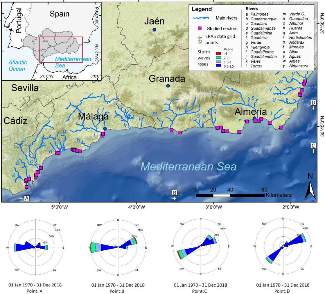
Figure 1. Location of the study area with storm waves roses obtained in previous works in four points of the ERA5 re-analysis data grid [65].
