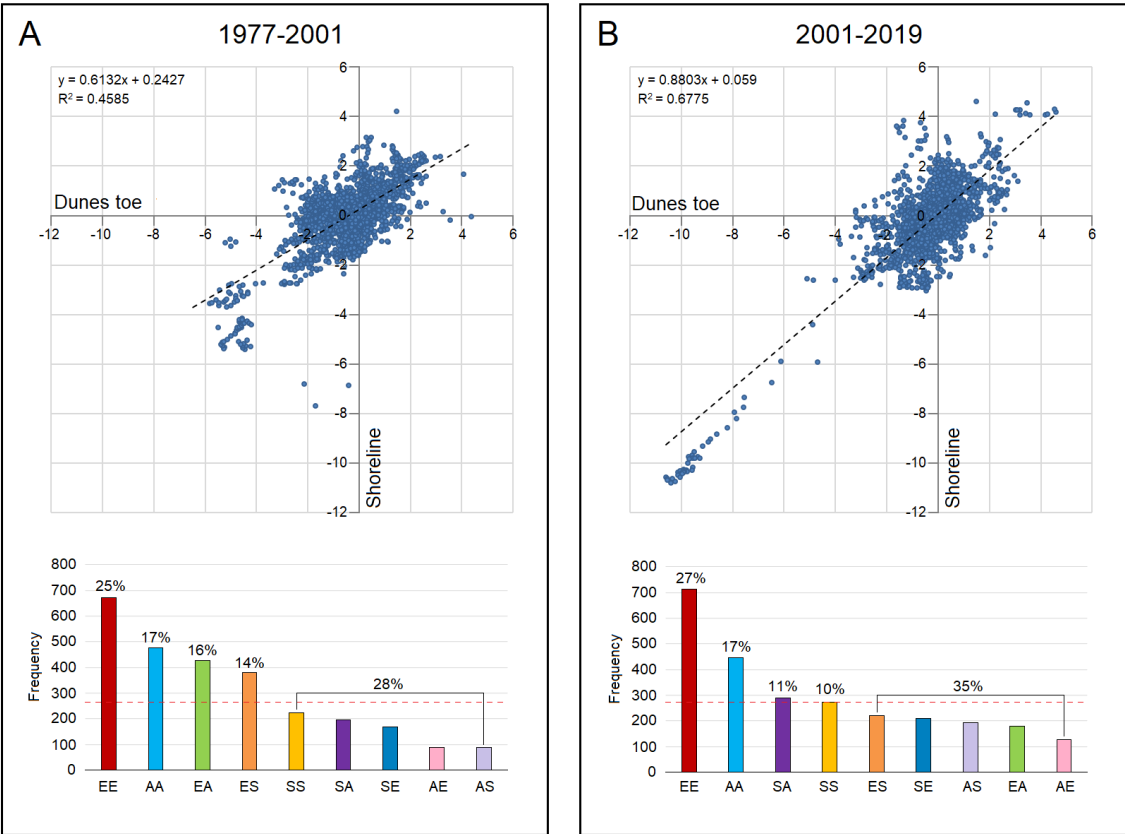
Figure 4. Foredune evolution classes vs. shoreline evolution classes for the 1977-2001 (A) and 2001-2019 (B) periods. Scatter charts (upper figures) present evolution classes at each studied period and the dotted line represents the linear regression line. Bar graphs (lower figures) show the frequency of each combination of classes: the first letter indicates the class of evolution for the dunes and the second letter the class of the shoreline evolution. E: Erosion, A: Accretion, and S: Stability. Red dotted line represents 10% of the data, only combinations of classes over this threshold were considered to describe most common observed cases.
