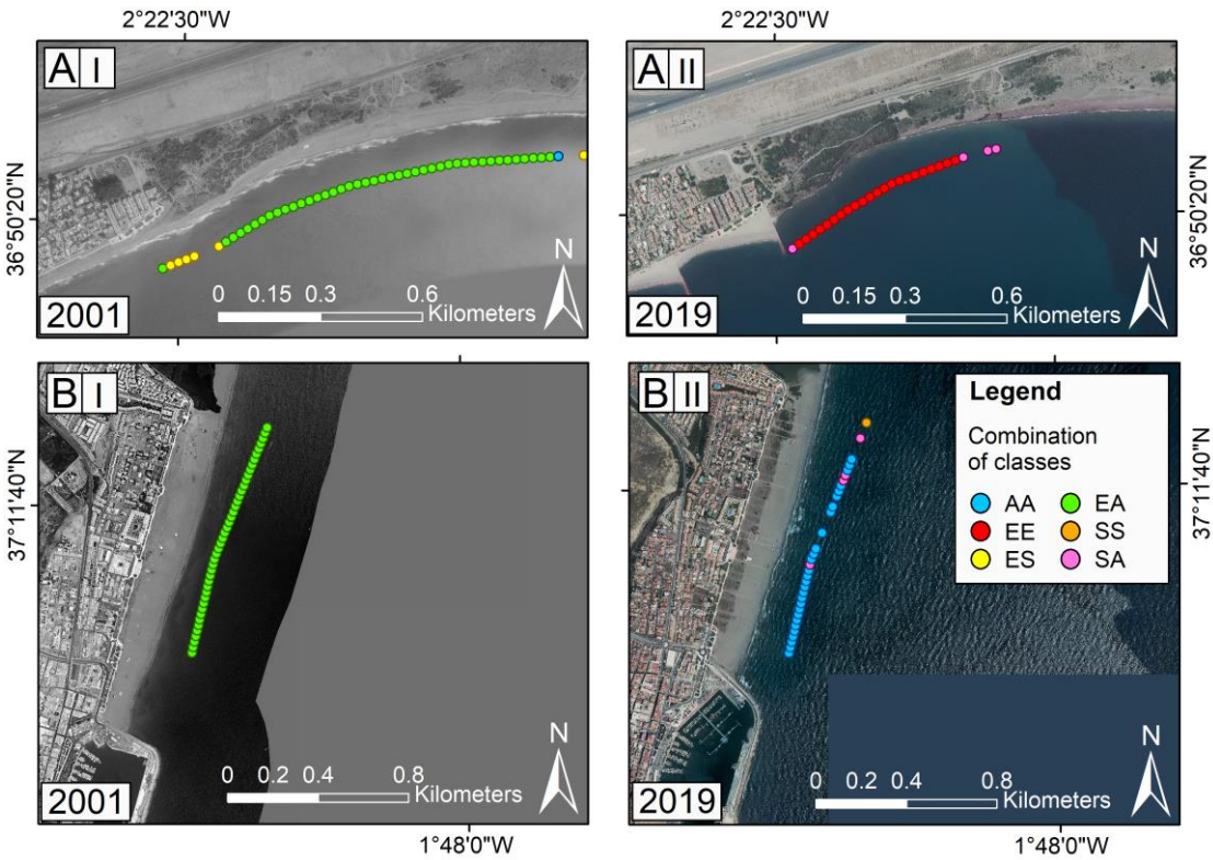
Figure 8. Changes of beach-dunes systems trends recorded at specific places and linked to the effect of coastal structures. A) Playa del Perdigal; B) Garrucha.
