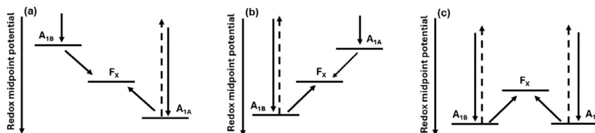
Scheme 1. Schematic presentation of relative redox potential of acceptors A_{1A} and A_{1B} in respect to F_x . Note, that lower redox midpoint potential means a more reducing potential. Dashed arrow indicates recombination reaction to P_{700}^+ . Left: cyclic electron transfer in the A branch. Middle: cyclic electron transfer in the B branch. Right: cyclic electron transfer in both A and B branches.
