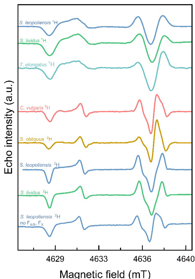
Figure 3. High-frequency D-band (130 GHz) pulsed EPR spectra of the SCRP recorded in PSI from different biological species. T=100 K, DAF = 1 \mu s.
