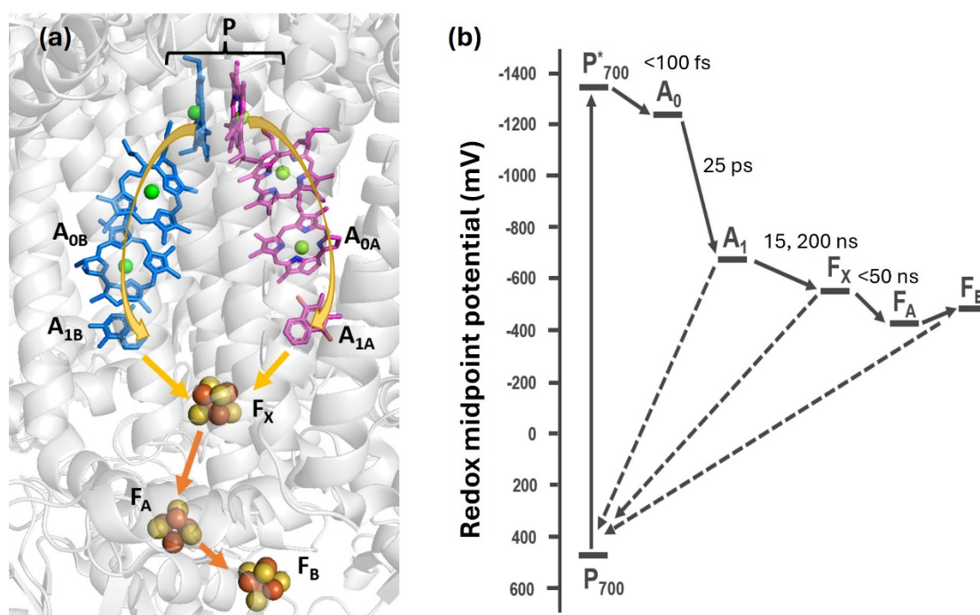
Figure 1. (a) Schematic structure and ET pathways in cyanobacterial Photosystem I. Following photoexcitation, the primary donor P becomes oxidized, transferring one electron to one of two almost identical chains of electron transfer cofactors: chlorophyll A 0 , phyloquinone A 1 , and converging at the three [4Fe-4S] clusters, F X , F A , and F B . Photoinduced ET in PSI is bidirectional at ambient temperature, proceeding through both the A and B branches of cofactors as indicated by arrows. (b) Energy diagram and time constants of forward electron transfer reactions in PSI. Information was taken from refs. 9,10. .
