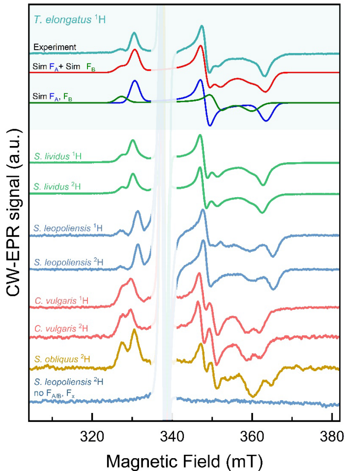
Figure 4. Continuous wave (cw) X-band (9.5 GHz) EPR spectra of various PSI samples. Samples were frozen in the dark, cooled down to 10 K in the cavity of the EPR spectrometer and subsequently illuminated with a white light LED. Microwave power 3 mW, modulation amplitude 1.2 mT.
