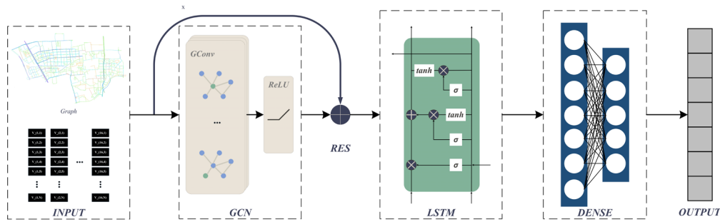
Figure 2. GraphResLSTM network architecture diagram.
