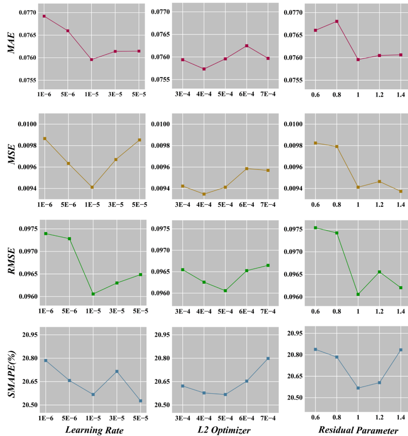
Figure 4. sensitivity analysis on crucial hyperparameters within the GraphResLSTM.
