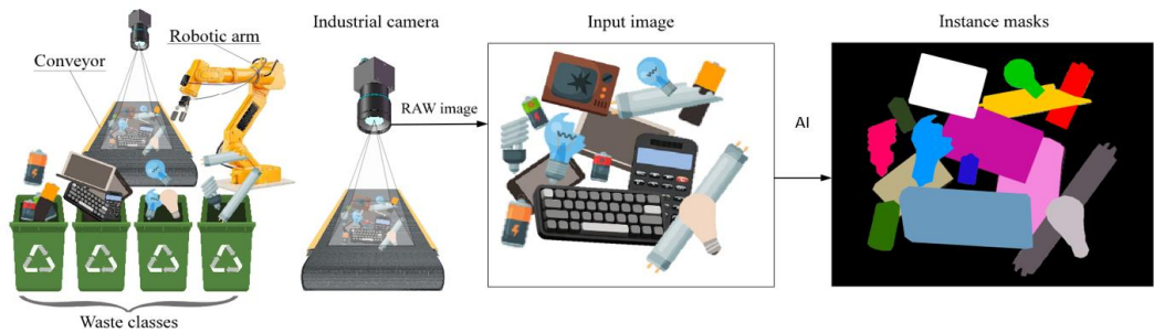
Figure 5. A typical robotic waste separation setup.
