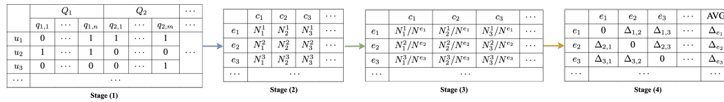
Figure 3. The process of the proposed approach for quantifying cross-sectoral discrepancies within different groups.
