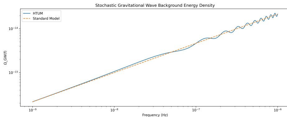
Figure 7. Stochastic Gravitational-Wave Background Energy Density: HTUM vs Standard Model.
