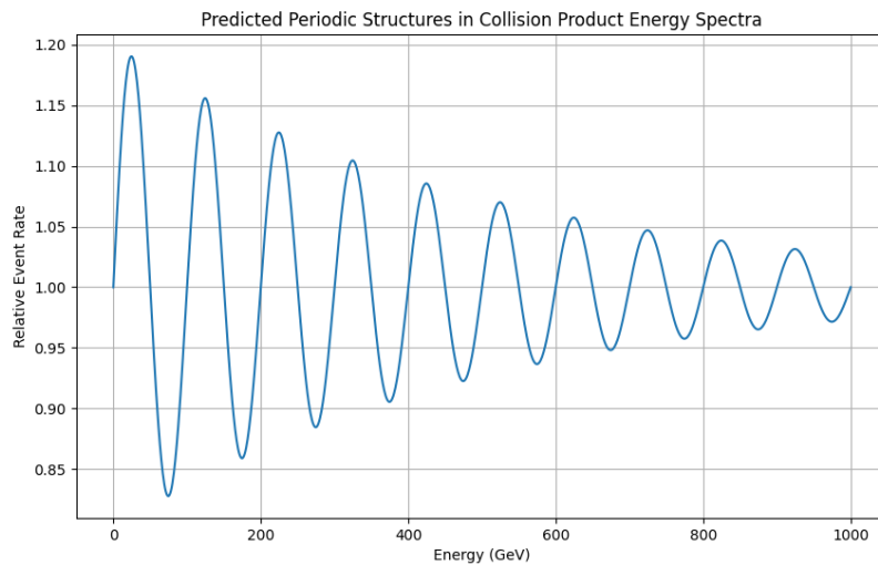
Figure 6. Predicted periodic structures in collision product energy spectra according to HTUM.
