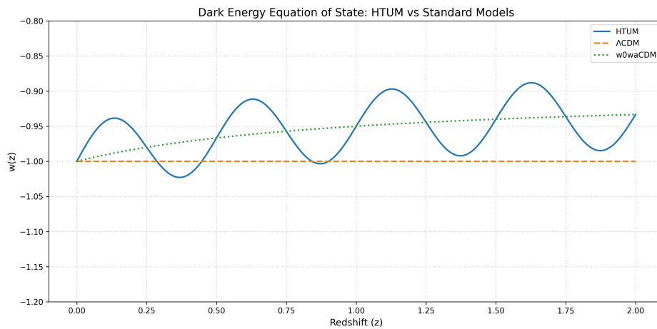
Figure 13. Dark energy Equation of State: HTUM vs Standard Models.
