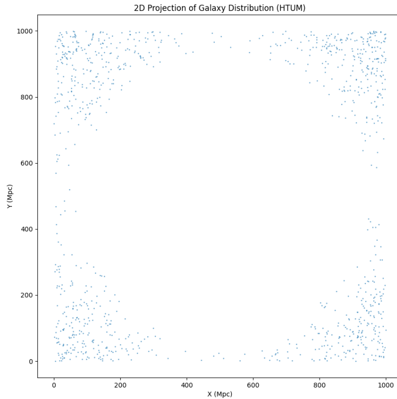
Figure 10. Galaxy distribution simulation.
