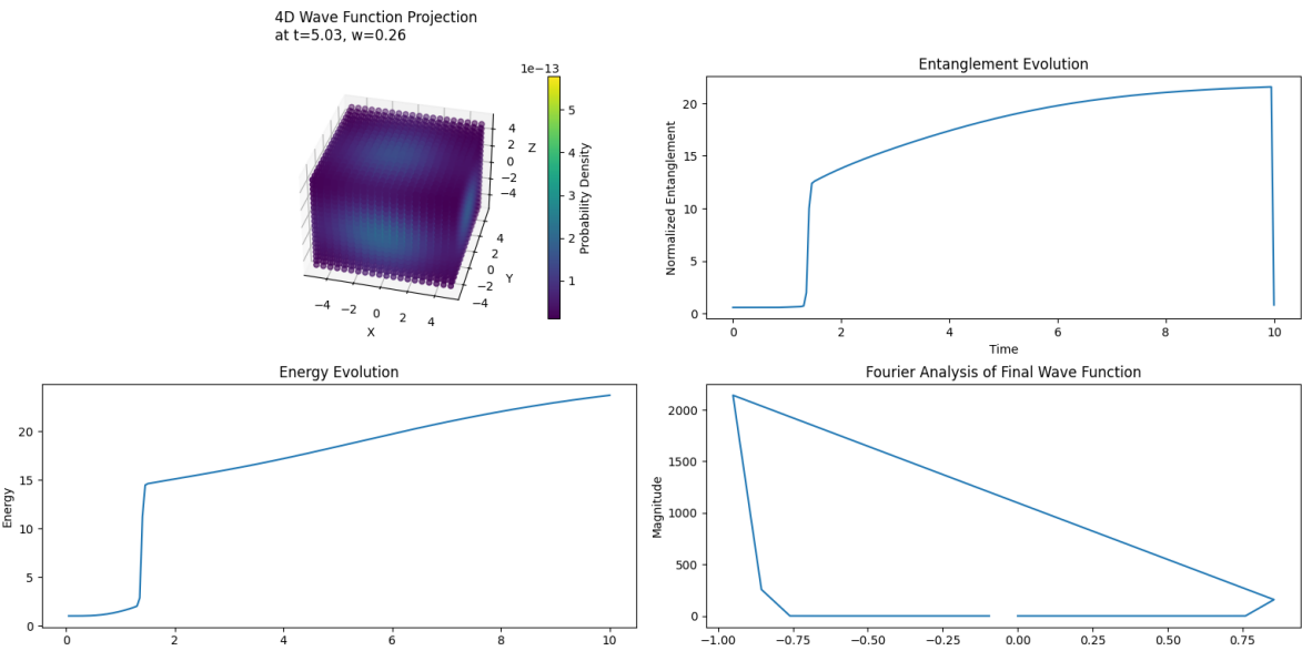
Figure 5. Simulation results of the latest HTUM simulation. (a) 4D Wave Function Projection, (b) Entanglement Evolution, (c) Energy Evolution, (d) Fourier Analysis of Final Wave Function.
