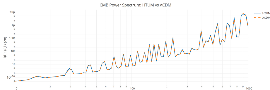
Figure 11. Comparison of CMB power spectra predicted by HTUM and \Lambda CDM models.
