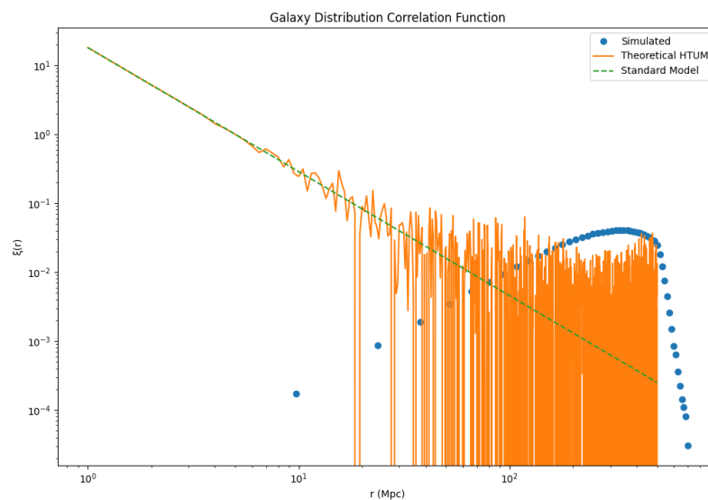
Figure 9. Galaxy distribution correlation function.
