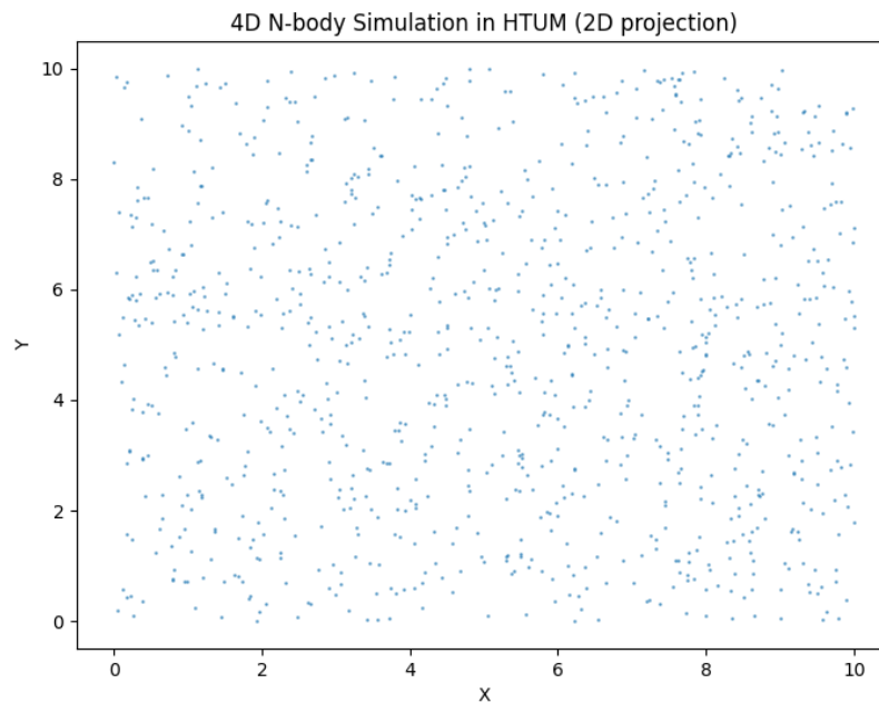
Figure 14. 4D N-body Simulation in HTUM (2D projection).
