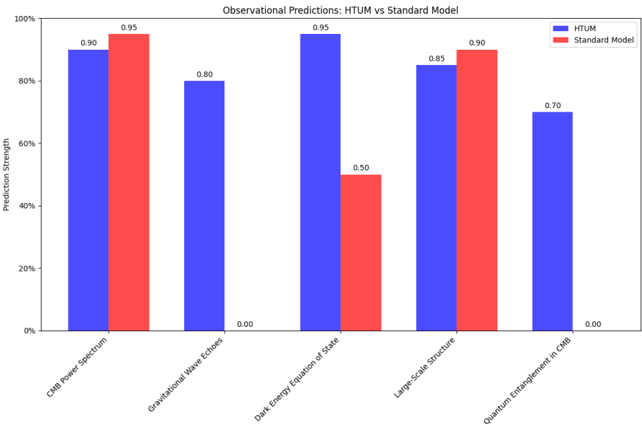
Figure 16. Comparison of observational predictions between HTUM and the Standard Model.
