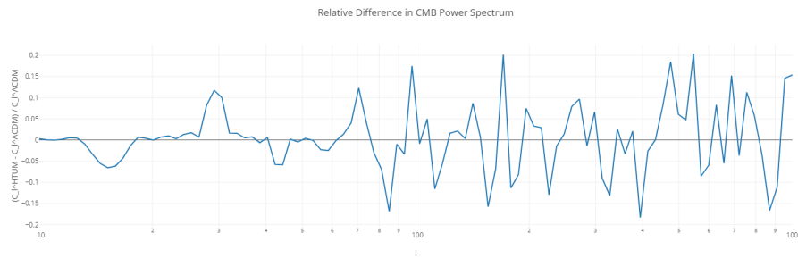
Figure 12. Relative difference in the CMB power spectrum between HTUM and \Lambda CDM models. The graph shows the fractional difference (C_l^{\text{HTUM}} - C_l^{\Lambda\text{CDM}}) / C_l^{\Lambda\text{CDM}} as a function of multipole moment l . Positive values indicate where HTUM predicts higher power than \Lambda CDM, and negative values indicate lower power.
