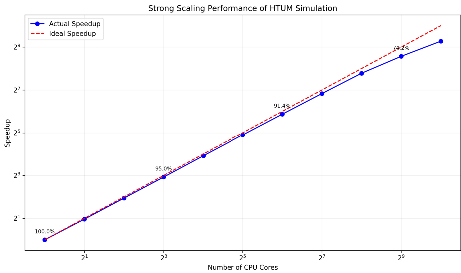
Figure A2. Strong scaling performance of HTUM simulation.
