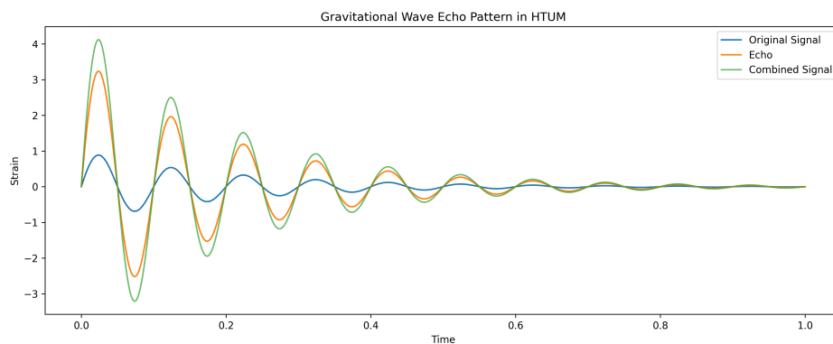
Figure 8. Gravitational Wave Echo Pattern predicted by HTUM.
