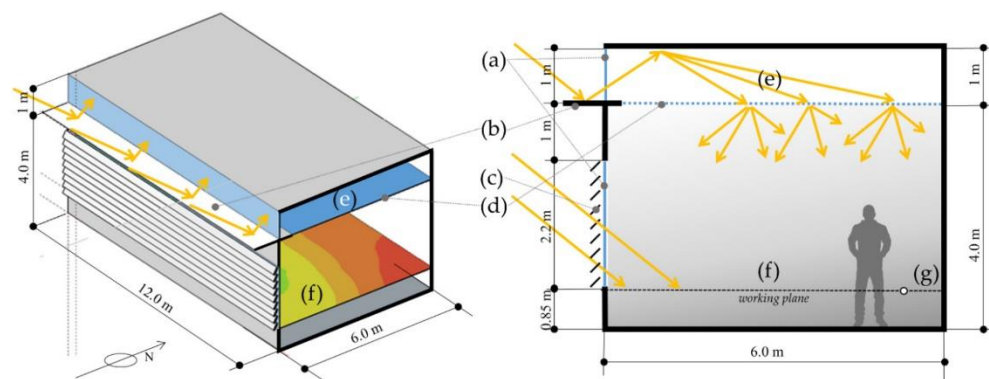
Figure 15. Combining a semi-transparent surface in line with the light shelf [16].
