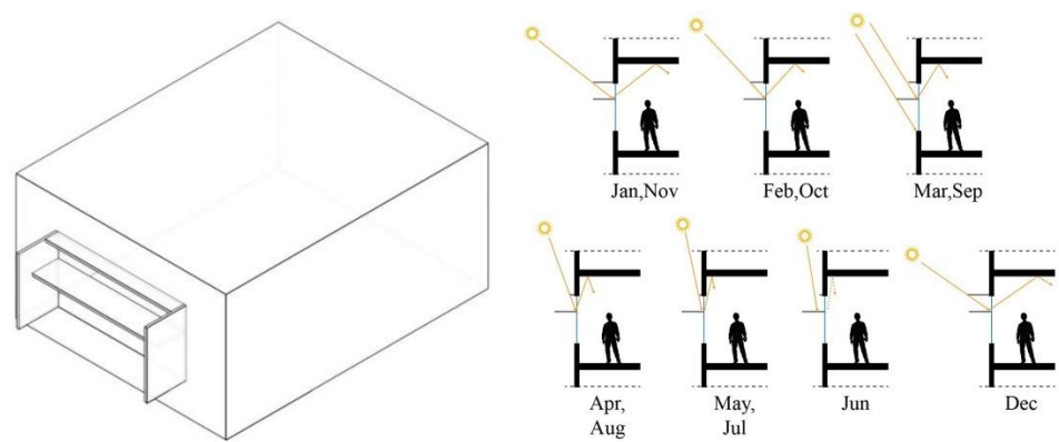
Figure 11. The optimal combination of shades and light shelf [2].
