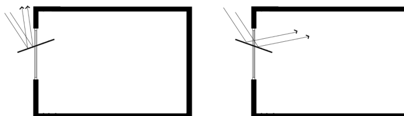
Figure 8. The role of light shelf slope in light penetration [44].
