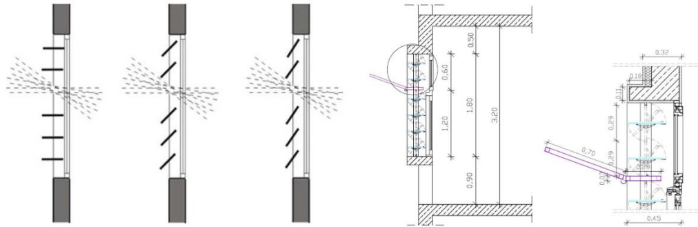
Figure 13. Combination of light shelves with louvers [15].
