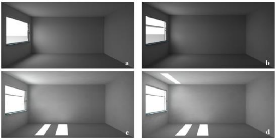
Figure 5. Various interior radiance renderings of a south-oriented room with dimensions 4 \times 6 \times 3 m and a window-to-floor ratio equal to 20% equipped with (a) No light shelf under overcast sky; (b) Perfectly diffuse external horizontal light shelf with 0.5 m depth (reflectance 0.8), under overcast sky; (c) Perfectly diffuse external horizontal light shelf with 0.5 m depth, under clear sky conditions, sun's elevation 37.8^\circ ; (d) Like; (c) but with mirror external horizontal light shelf [6].
