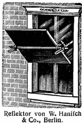
Figure 3. Daylight reflector by W. Hanifch and Co. [7].
