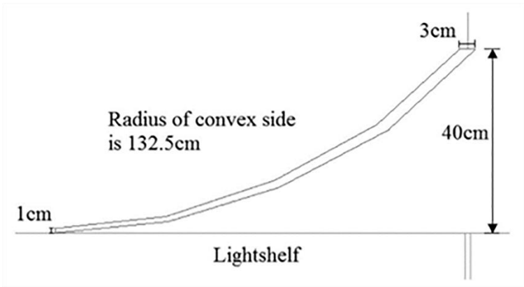
Figure 6. Selected mode for the glass above the light shelf [26].
