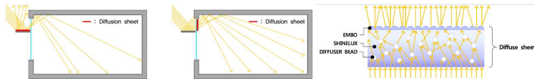
Figure 14. Combination of light shelf with diffusion sheet [17].
