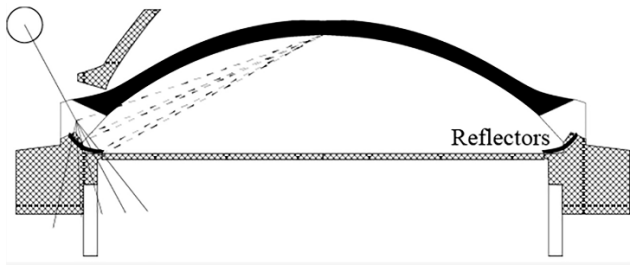
Figure 2. Schematic representation of the parapet of Hagia Sophia based on Anthemius’s reflector superimposed over the cross-section of the original dome [6].
