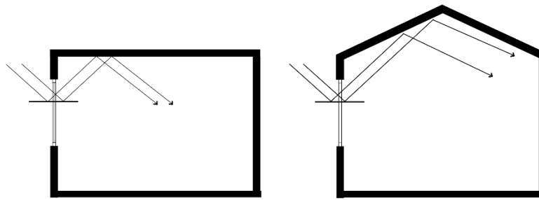
Figure 9. Increasing the penetration depth of light in sloping roofs [44].
