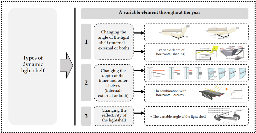
Figure 17. Classification of dynamic light shelves [24,25,33,49].
