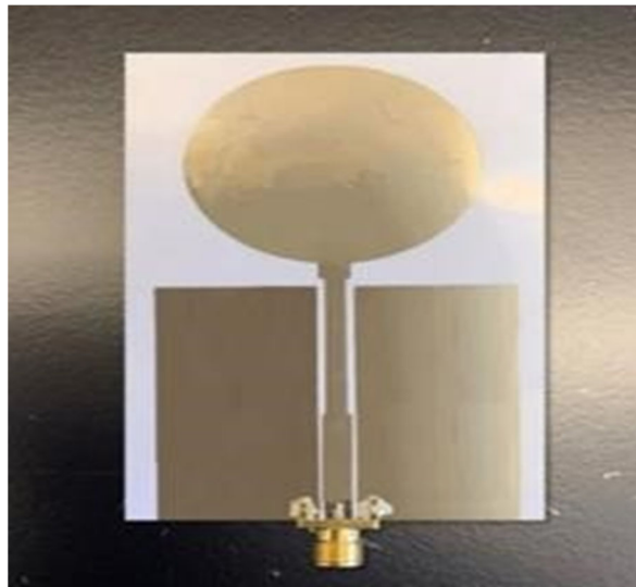
Figure 2. Chen et al. Inkjet-printed UWB antenna.
