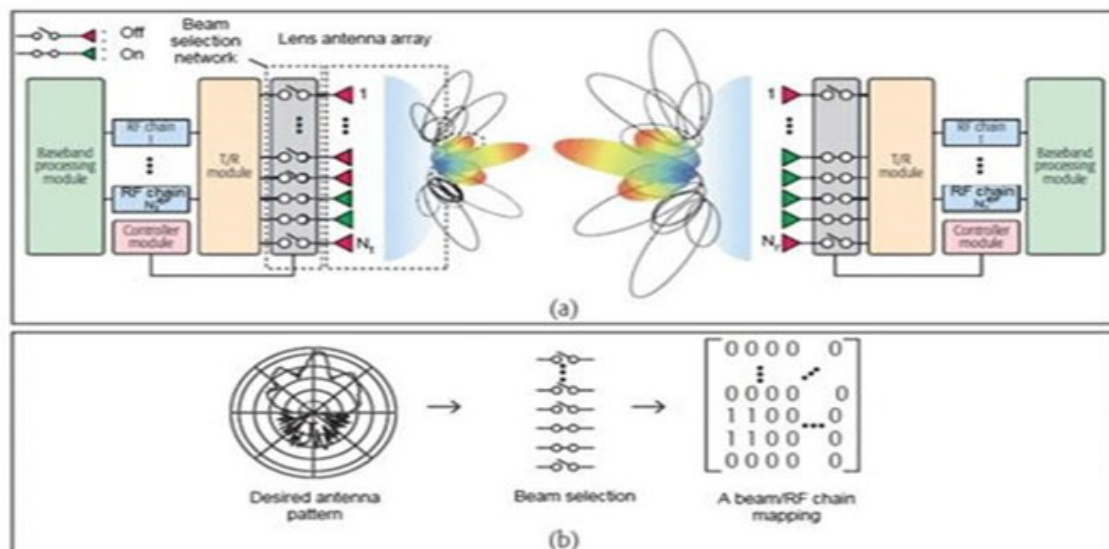
Figure 6. Zarini et al. Schematic of beamspace technology: (a) architectural components; (b) analog beam selection.
