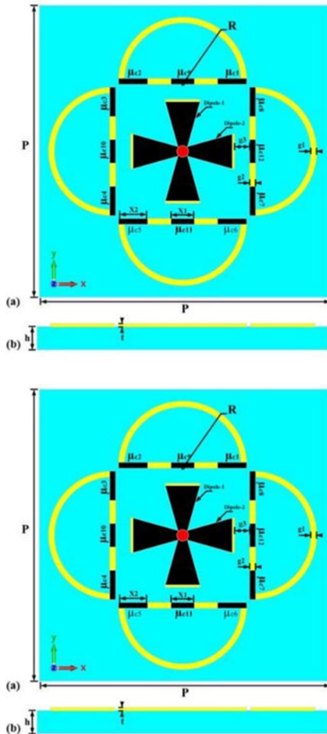
Figure 4. Jin et al. Structure of the CRTA. a) Top view. b) Side view.
