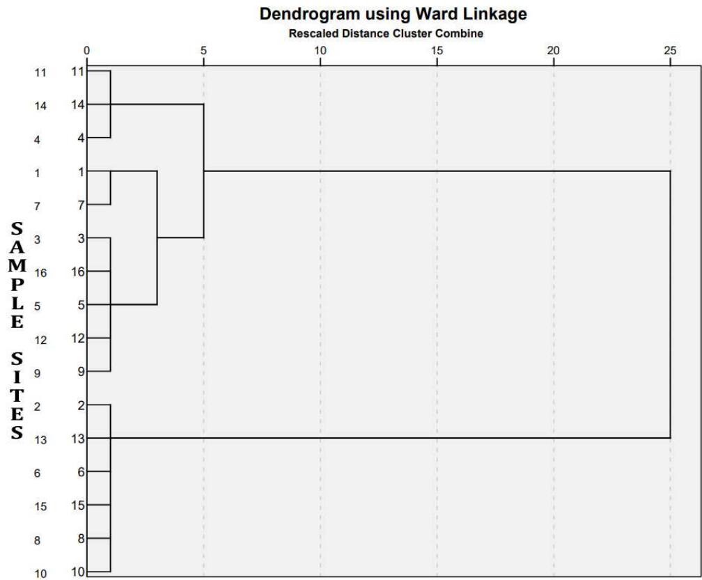
Figure 6. Dendrogram from HCA of sampling sites.
