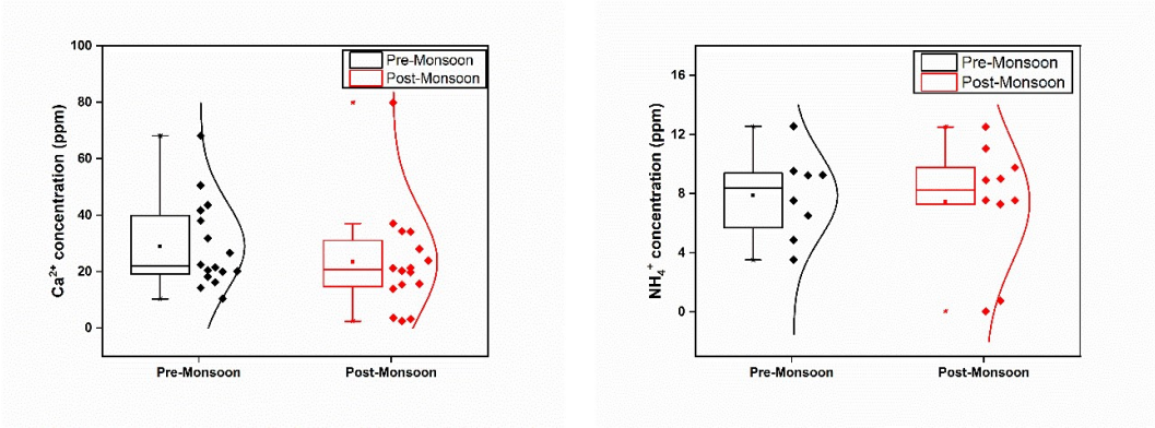
Figure 3. Spatial and temporal variations in the ionic concentration of the study area.
