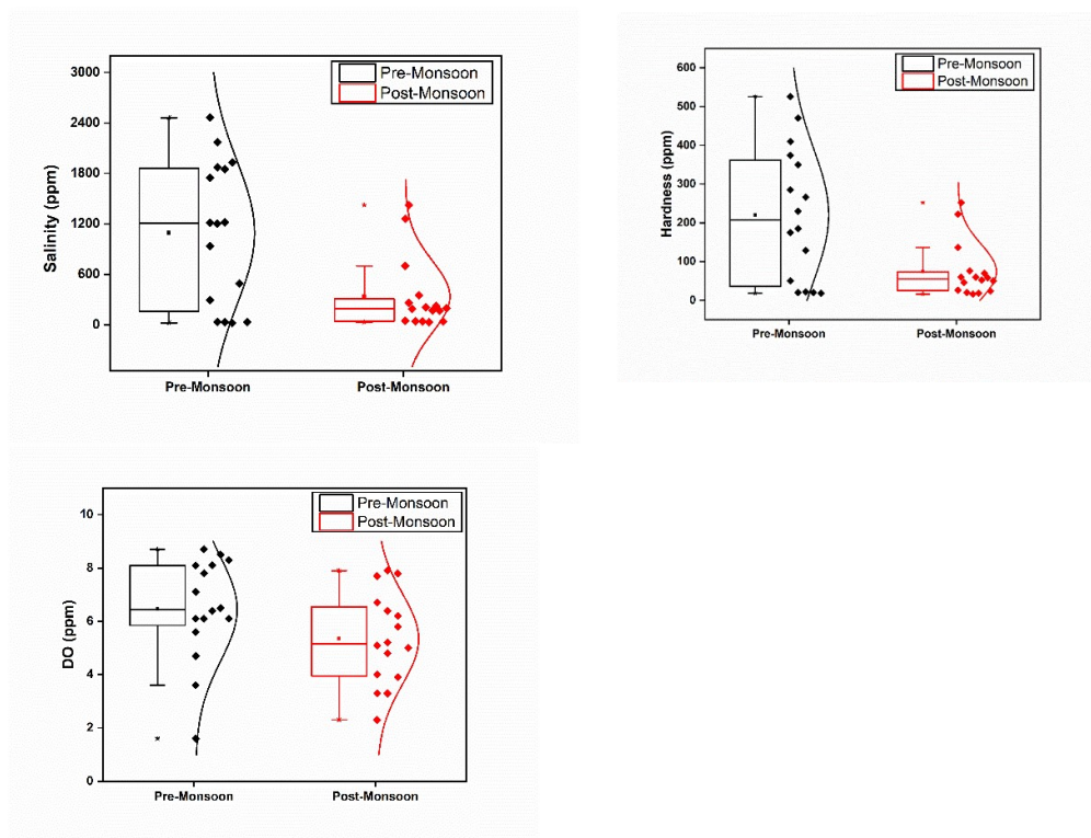
Figure 2. Spatial and temporal variations in physico-chemical parameters in the study area.
