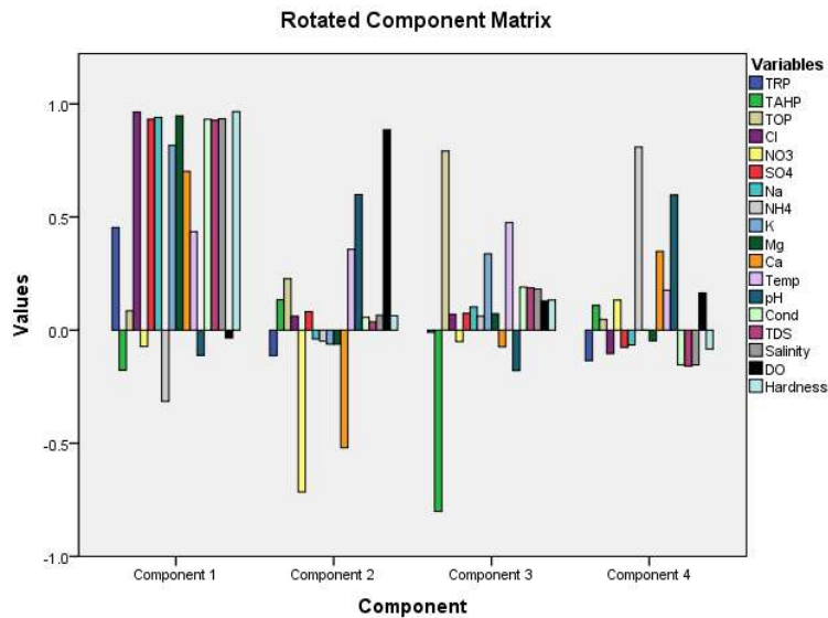
Figure 5. Principal component analysis-factor loadings for the variables.
