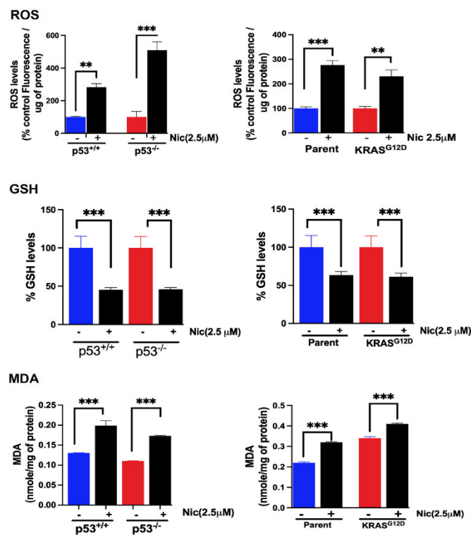
Figure 13. Effects of niclosamide on cellular levels of ROS, GSH, and MDA. The cells were treated with niclosamide (2.5 \mu M) for 24 h. Data are given as mean \pm S.E. **, p < 0.01 ; ***, p < 0.001 .
