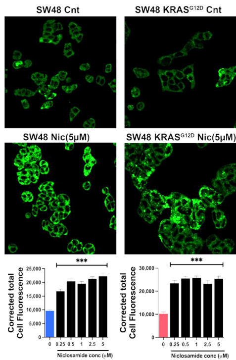
Figure 11. Induction of ferroptosis by niclosamide (5 \mu M) in SW48 cells with and without G12D mutation in KRAS. Quantification of the fluorescence signals (mean \pm S.E.) are given. ***, p < 0.001 .
