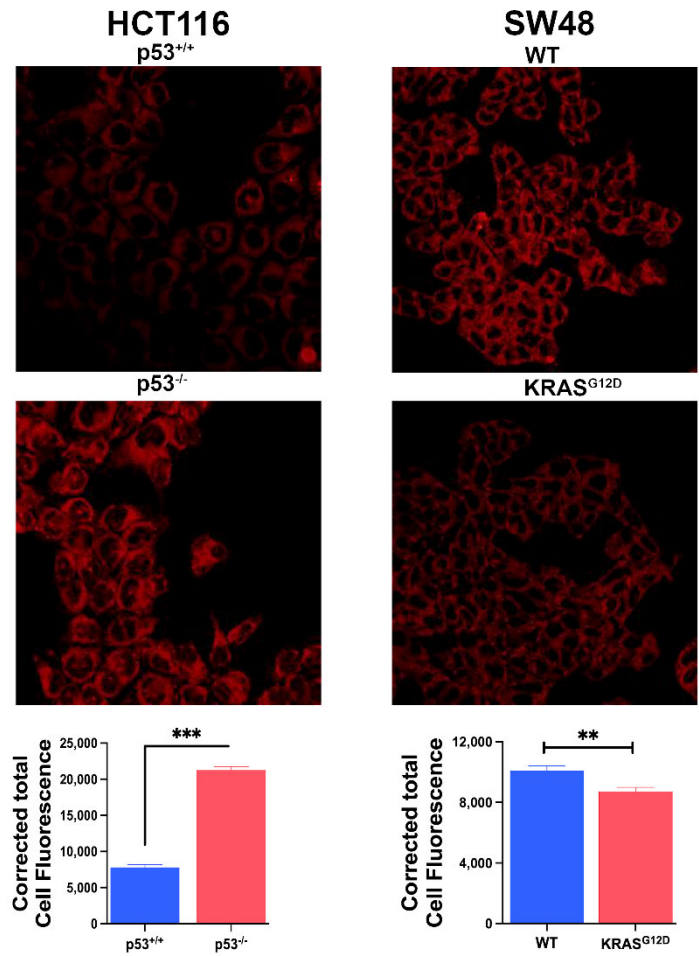
Figure 6. Iron levels in the two isogenic cell lines with and without p53 (HCT-116) and with and without G12D mutation in KRAS (SW48). The fluorescence signals were also quantified (data given as mean ± S.E.). **, p < 0.01 ; ***, p < 0.001 .
