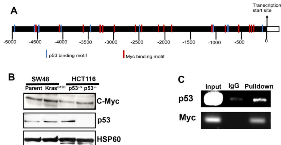
Figure 2. Evidence for SLC38A5 as a transcriptional target for p53 and Myc. Locations for theoretical binding sites in human SLC38A5 gene promoter for p53 and Myc ( A ). Protein levels for p53 and Myc in the isogenic cell lines SW48 with and without KRAS-G12D mutation and HCT-116 with and without p53 ( B ). SW48 parent cells were used for ChIP assay to provide evidence for the binding of p53 and Myc to the SLC38A5 gene promoter ( C ).
