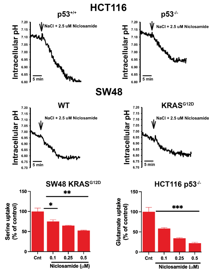
Figure 8. Effects of niclosamide on intracellular pH in all four cell lines and on the transport activity of SLC38A5 in SW48 cells with G12D mutation in KRAS and on the transport activity of SLC7A11 in p53 -null HCT-116 cells. Data are given as mean \pm S.E. *, p < 0.05 ; **, p < 0.01 ; ***, p < 0.001 .
