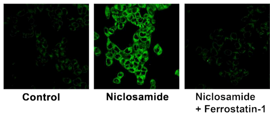
Figure 12. Blockade of niclosamide (5 \mu M)-induced ferroptosis by ferrostatin (10 \mu M) in p53 -null HCT116 cells.
