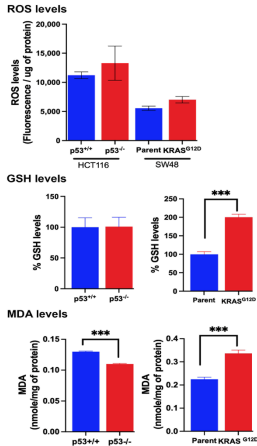
Figure 7. Basal levels of ROS, GSH and MDA. Data (mean \pm S.E.) are from three independent experiments. ***, p < 0.001 . When not specified, the differences were not statistically significant.
