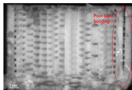
(b) Optical microscopy image for experimental run 3 (LH: 0.1 mm, I: 100%, NT: 215 °C)
