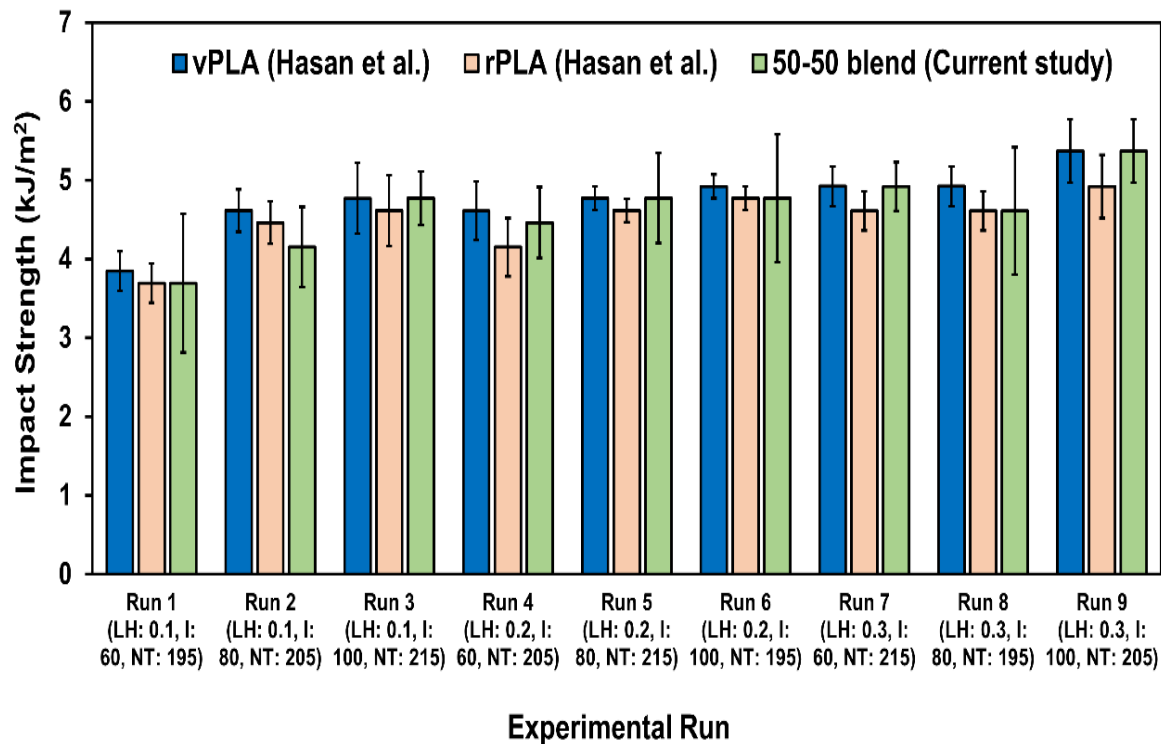
Figure 15. Comparison of the impact strengths of vPLA, rPLA, and vPLA:PC-PLA (50:50) blended filament specimens (where LH is the layer height, I is the infill percentage, and NT is the nozzle temperature).
