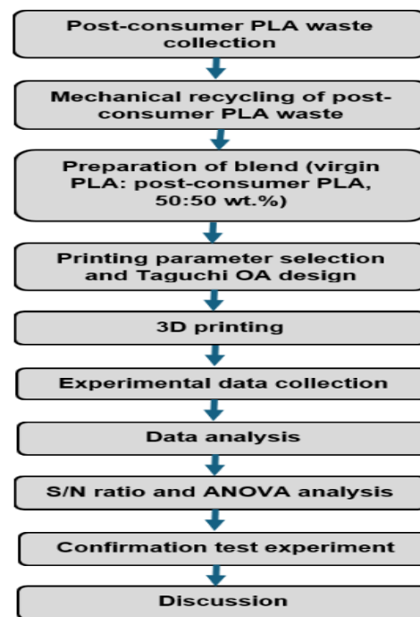
Figure 1. Flow chart of the research methodology.
