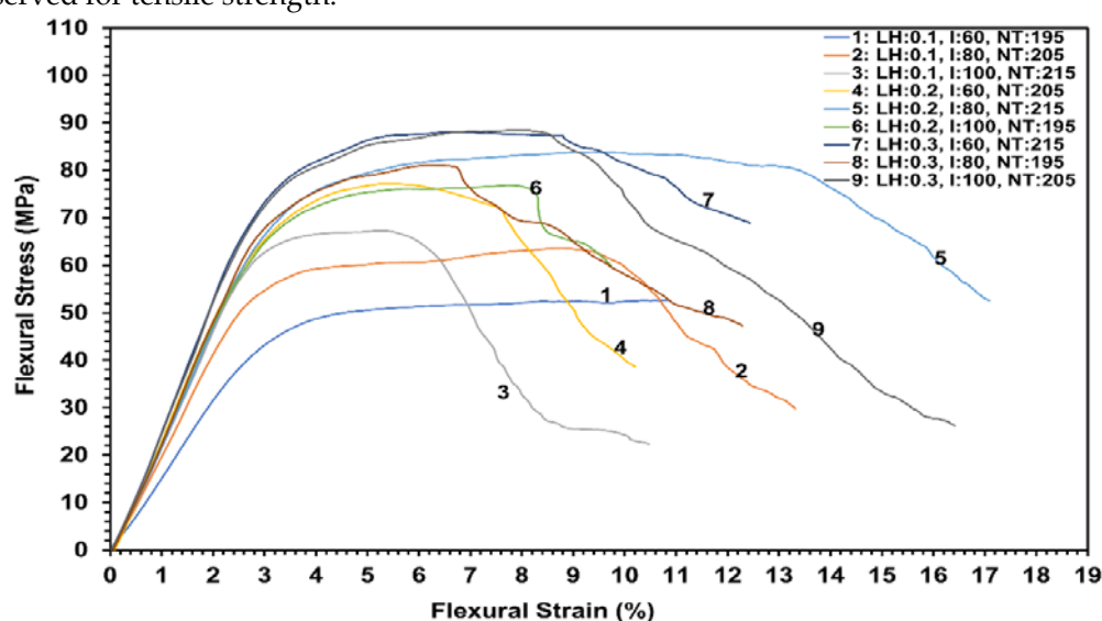
Figure 12. Flexural stress–strain curves for vPLA: PC-PLA (50:50) blended filament-printed specimens (where LH is the layer height, I is the infill percentage, and NT is the nozzle temperature).
