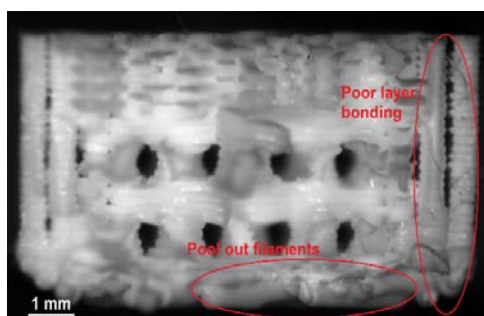
(a) Optical microscopy image for experimental run 1 (LH: 0.1 mm, I: 60%, NT: 195 °C)
