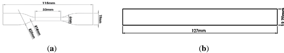
Figure 5. Schematic of (a) tensile and (b) flexural test specimens [46].
