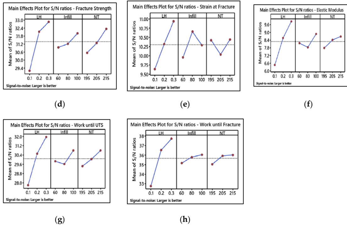
Figure 17. Main effects plots illustrating S/N ratios for the tensile properties of blended specimens: (a) yield strength, (b) ultimate tensile strength (UTS), (c) strain at UTS, (d) fracture strength, (e) strain at fracture, (f) elastic modulus, (g) work until UTS, and (h) work until fracture.
