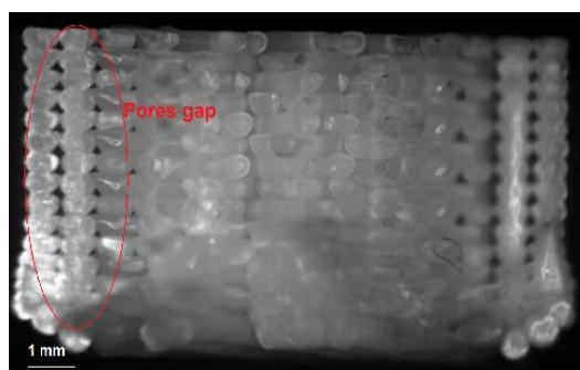
(c) Optical microscopy image for experimental run 6 (LH: 0.2 mm, I: 100%, NT: 195 °C)
