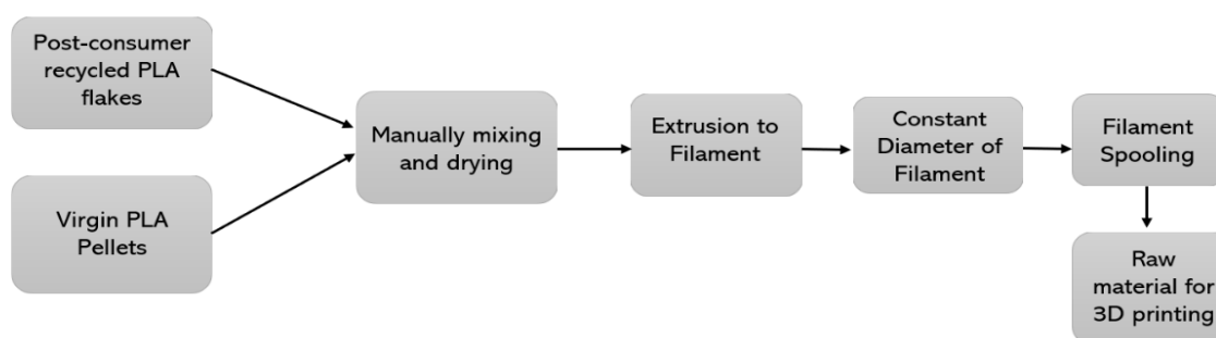
Figure 3. Flowchart of post-consumer PLA filament production.
