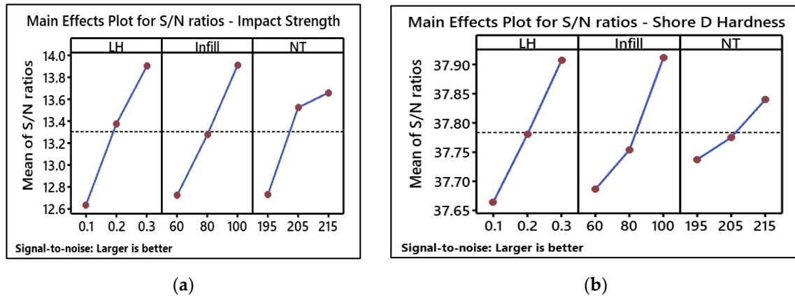
Figure 19. Main effect plots of S/N ratios for (a) impact strength and (b) hardness of blended specimens.
