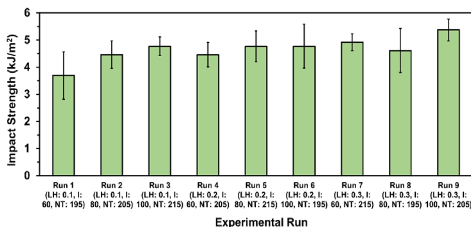
Figure 14. Charpy impact strength of vPLA:PC-PLA (50:50) blended 3D printed specimens (where LH is the layer height, I is the infill percentage, and NT is the nozzle temperature).
