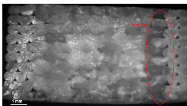
(e) Optical microscopy image for experimental run 9 (LH: 0.3 mm, I: 100%, NT: 205 °C)
