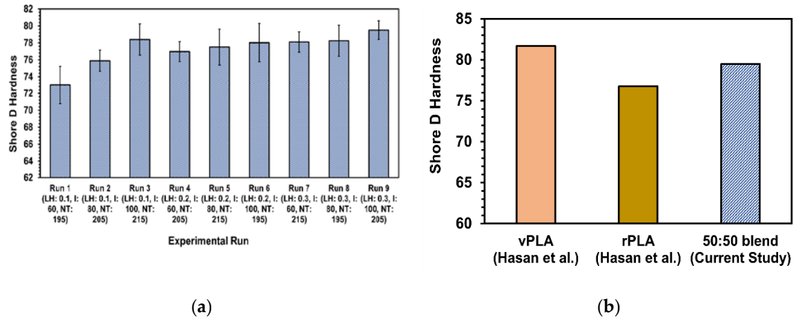
Figure 9. (a) Shore D hardness of the vPLA:PC-PLA (50:50) blended specimens, and (b) comparison of hardness for vPLA, rPLA and vPLA:PC-PLA (50:50) blended specimens (where LH is the layer height, I is the infill percentage, and NT is the nozzle temperature).
