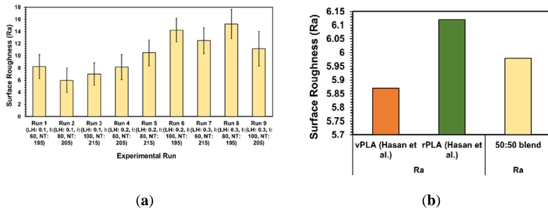
Figure 8. (a) Surface roughness of vPLA:PC-PLA (50:50) blended filament specimens and (b) comparison of surface roughness of vPLA, rPLA, and vPLA:PC-PLA (50:50) blended specimens (where LH is the layer height, I is the infill percentage, and NT is the nozzle temperature).
