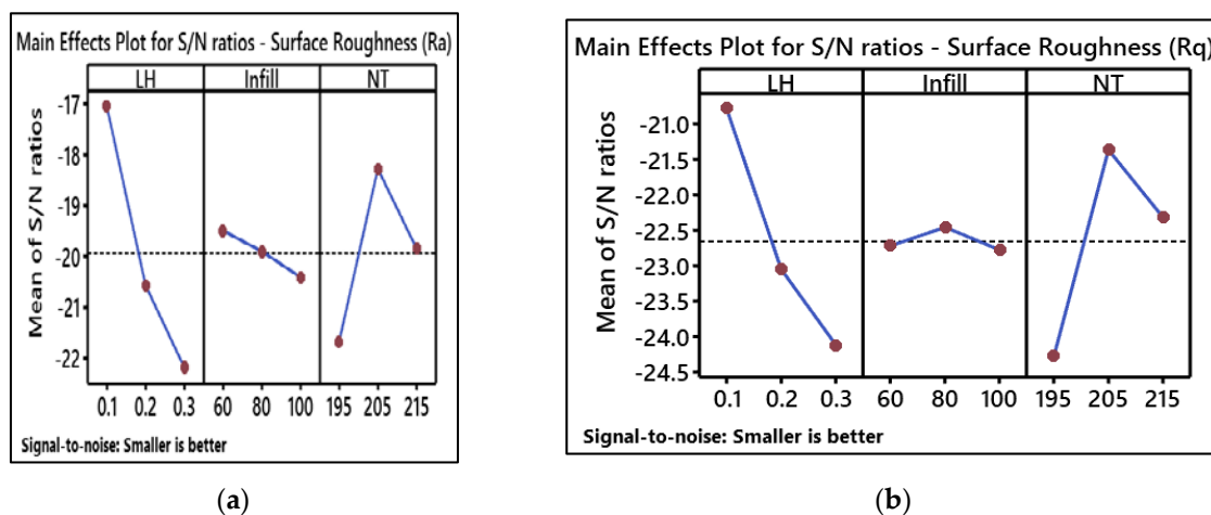
Figure 20. Main effects plot of S/N ratios for surface roughness of blended specimen (a) R_a , (b) R_q .
