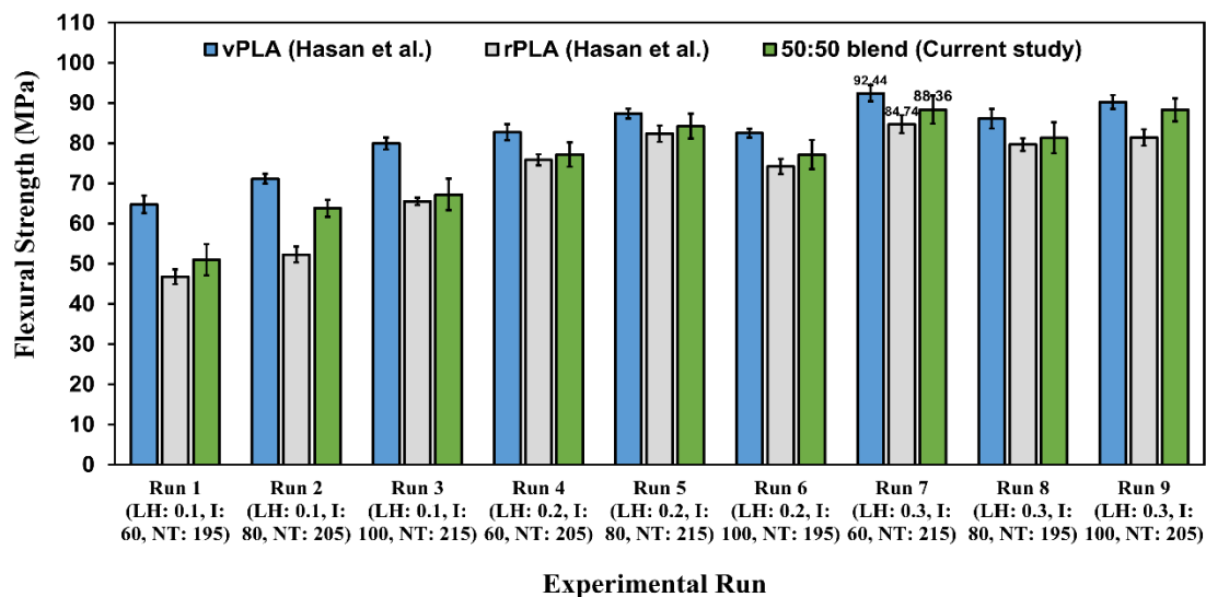
Figure 13. Comparison of flexural strength for vPLA, rPLA, and vPLA:PC-PLA (50:50) blended filament specimens (where LH is the layer height, I is the infill percentage, and NT is the nozzle temperature).
