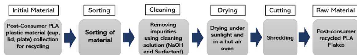
Figure 2. Processing of household post-consumer PLA waste.
