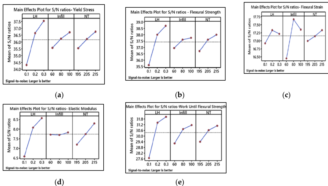
Figure 18. Main effects plots illustrating S/N ratios for the flexural properties of blended specimens: (a) yield strength, (b) flexural strength, (c) flexural strain, (d) elastic modulus, and (e) work until flexural strength.
