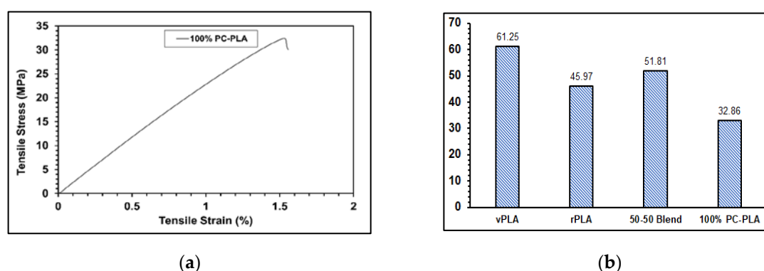
Figure 21. (a) Stress-strain diagram of 100% PC-PLA 3D printed tensile sample, and (b) comparison of UTS for vPLA, rPLA, vPLA:PC-PLA (50:50) blended specimens, and 100% PC-PLA tensile samples.
