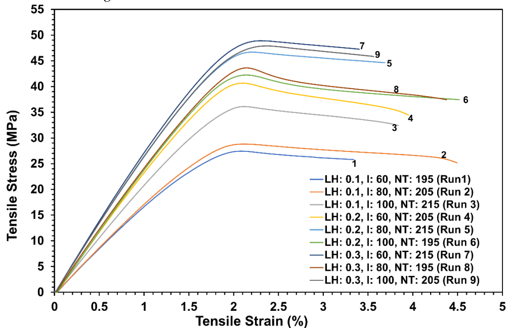
Figure 10. Tensile stress vs. tensile strain curves for vPLA:PC-PLA (50:50) blended filament printed specimens (where LH is the layer height, I is the infill percentage, and NT is the nozzle temperature).
