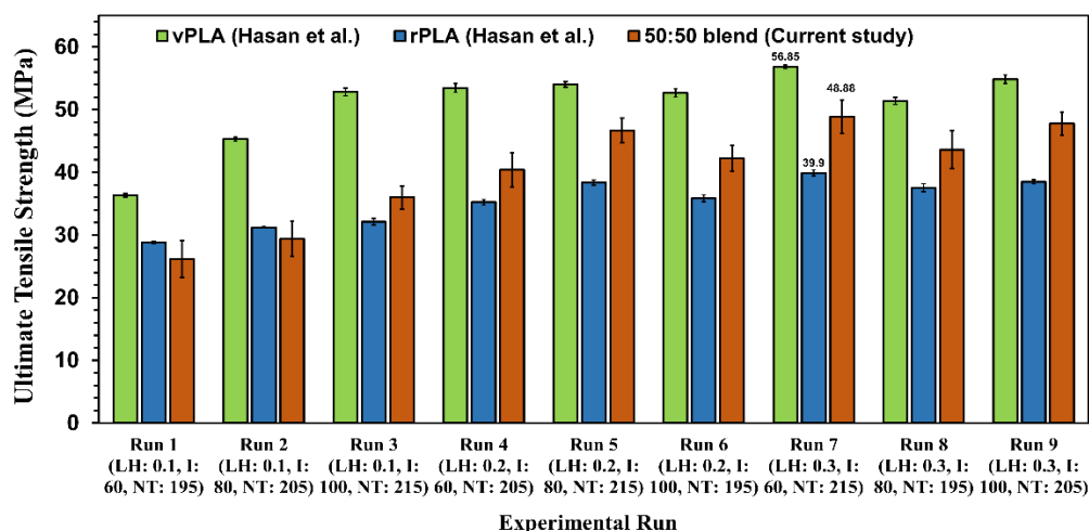
Figure 11. Comparison of UTS for vPLA, rPLA, and vPLA:PC-PLA (50:50) blended filament 3D printed specimens (where LH is the layer height, I is the infill percentage, and NT is the nozzle temperature).
