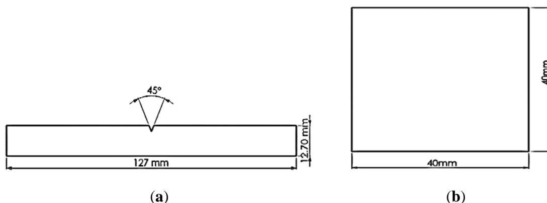
Figure 6. Schematic of (a) impact and (b) hardness test specimens [46].
