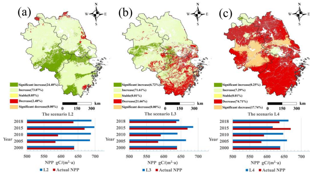
Figure 8. Changes of NPP in different scenarios: (a) L2, (b) L3, (c) L4.
