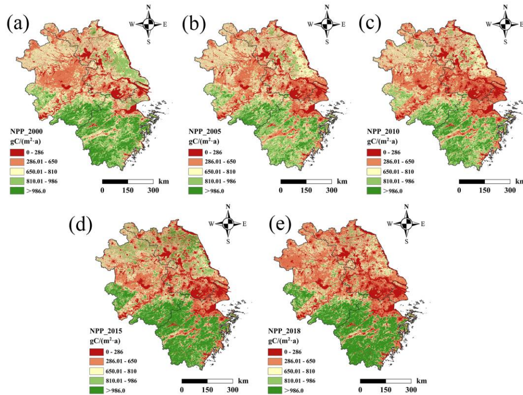
Figure 2. Spatial distribution of NPP in the YRD region from 2000 to 2018: (a) 2000, (b) 2005, (c) 2010, (d) 2015, (e) 2018.
