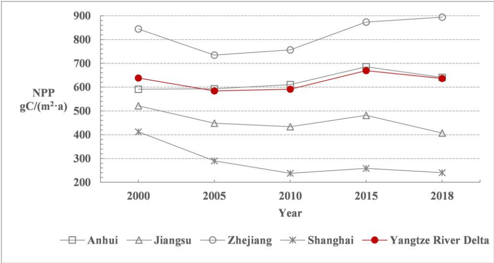
Figure 3. Changes in the average NPP value of the YRD region between 2000 and 2018.
