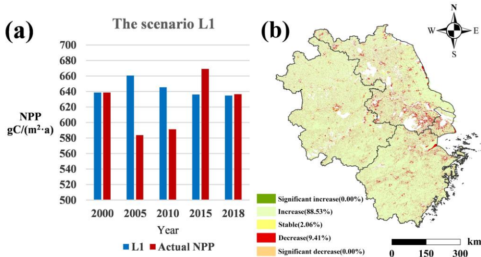
Figure 6. Changes of NPP in the scenario L1: (a) Comparison of L1 with the realistic scenario, (b) Trends of NPP in L1.
