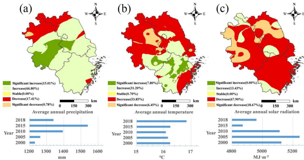
Figure 7. Changes of climatic factors in the YRD region from 2000-2018: (a) average annual precipitation, (b) average annual temperature, (c) average annual solar radiation.
