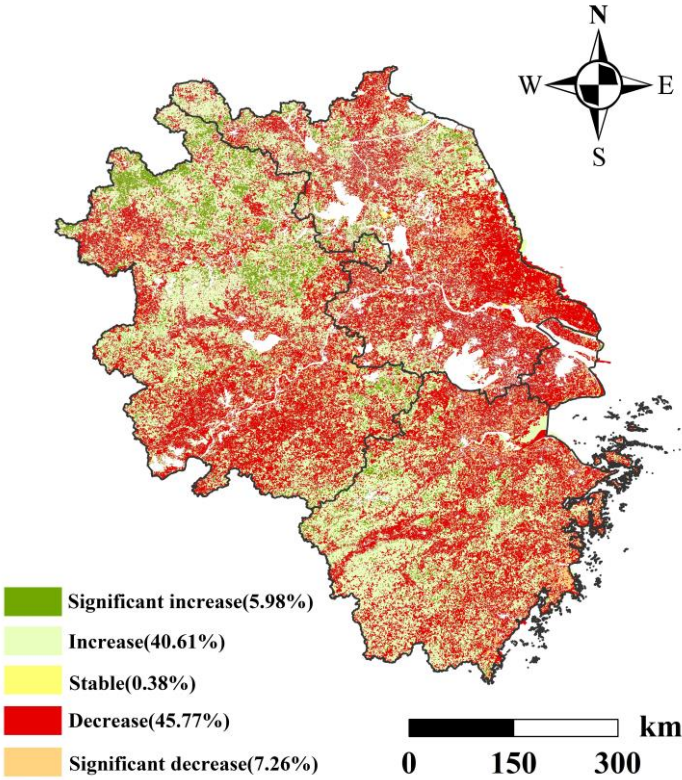
Figure 4. Trends in NPP of the YRD Region between 2000 and 2018.
