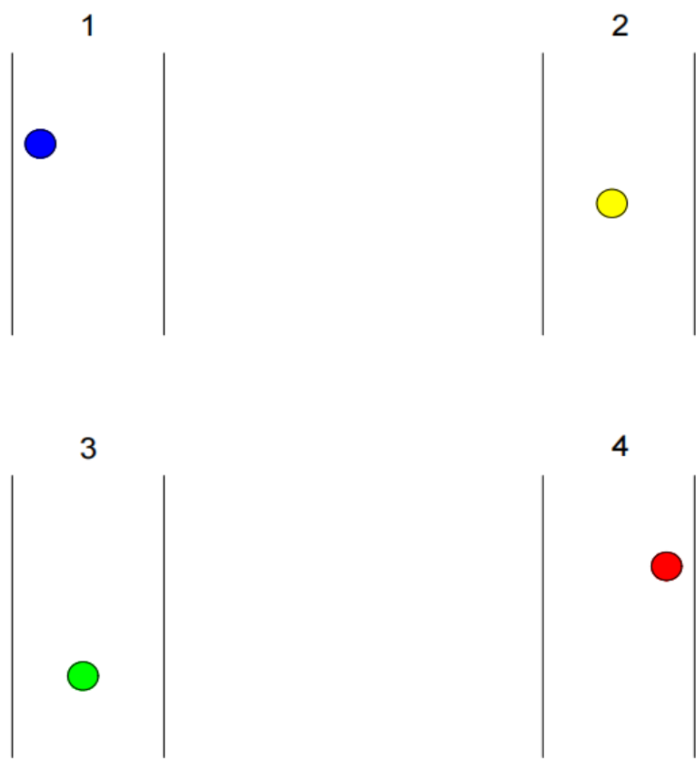
Figure 5. Two-slit interference experiment.
