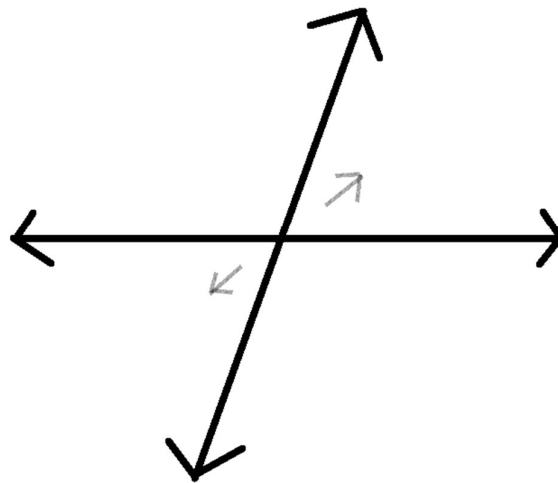
Figure 9. A two-dimensional substance.
