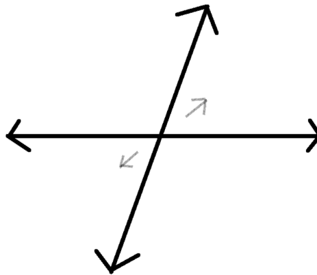
Figure 9. A two-dimensional substance.
