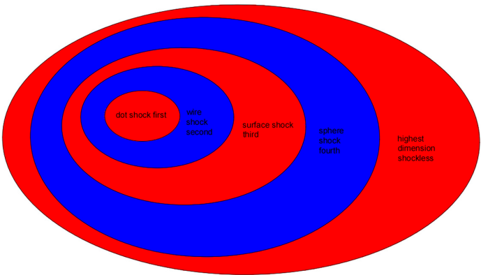
Figure 8. The relationship between dimensions is that the higher dimensions have a larger range but infinitely small energy, the lower dimensions are faster, and the lower dimensions produce more dimensions.
