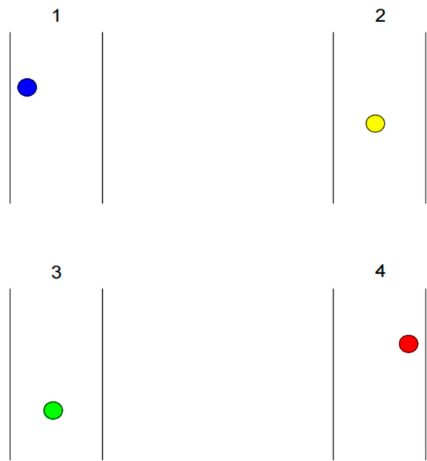
Figure 5. Two-slit interference experiment.
