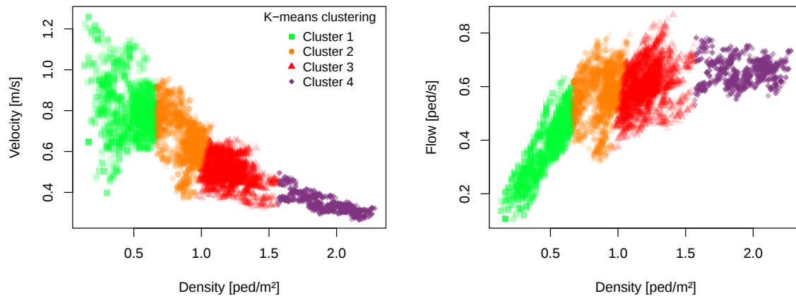
Figure 2. Results of the K-Means clustering. Trajectory scenes are clustered as shown by the different colors of the points.
