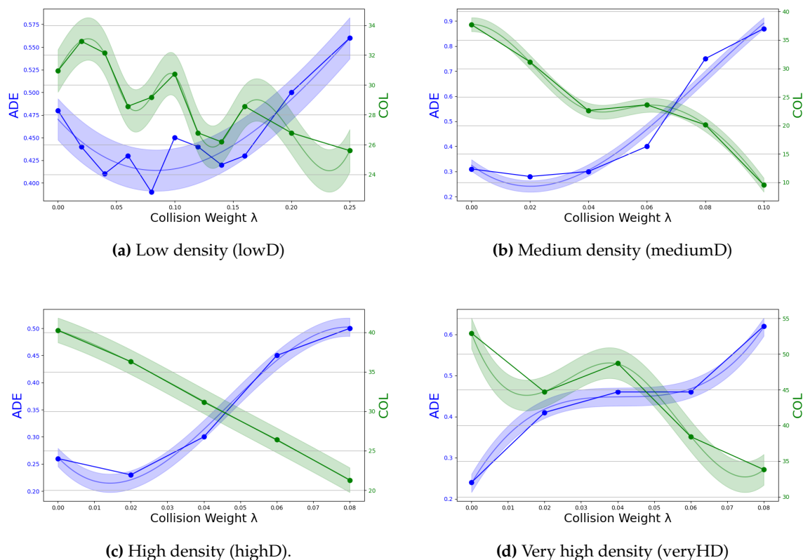
Figure 5. ADE and COL metrics for the two-stage SLSTM algorithm according to the collision weight \lambda for the four density levels.
