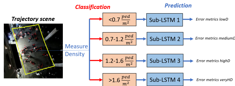
Figure 3. Schemata of our two-stage prediction approach
