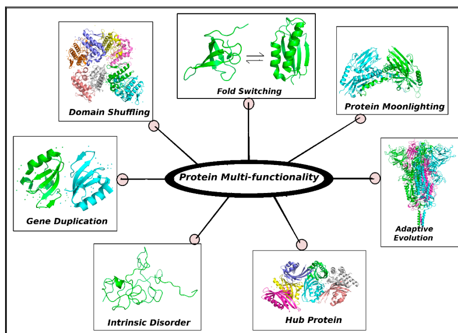
Figure 1. The composite figure portrays different evolutionary tools to express protein multi-functionality. The represented repertoire includes (i) Gene Duplication: Rck (PDB ID: 4YS2), (ii) Domain Shuffling: RV4/RV7 complex (1OQS), (iii) Fold Switching: RfaH C-terminal domain (6TF4, 7MN1), (iv) Protein Moonlighting: a Metazoan Small Heat shock Protein (2BOL), (v) Adaptive Evolution: Spike Protein with highly mutable FLC Spike from SARS-CoV-2 (6XR8), (vi) Hub Proteins: CaMKII alpha hub (7REC) and (iii) Intrinsic Disorder: alpha synuclein (a random template from a loop-modelled, MD-simulated trajectory [23]).
