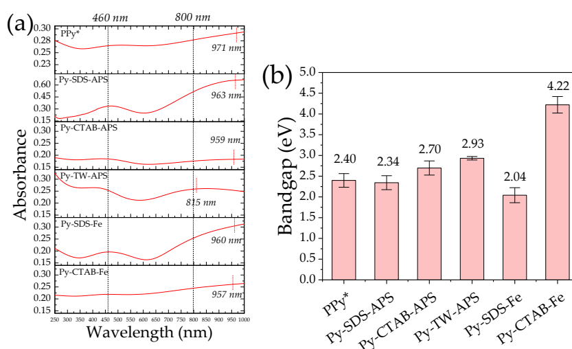
Figure 5. (a) UV-Vis-NIR absorption ranged between 250 and 1000 nm, (b) bandgap calculated from UV-Vis-NIR absorbance.
