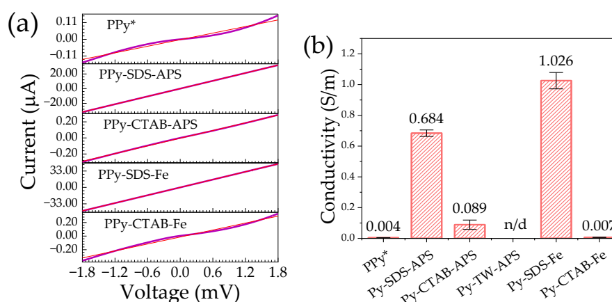
Figure 3. (a) I/V graph data determined from the autopolarization machine using the LSV mode, dash line refer to slope fitted from Origin software, and (b) conductivity calculated from resistance based on of each sample.
