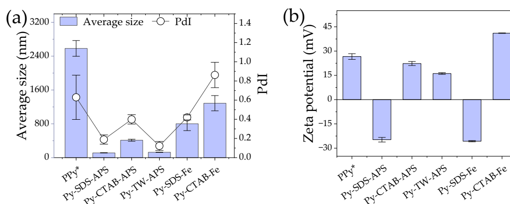
Figure 1. Average size, PDI, and zeta potential determined from zetasizer: (a) average size and PDI, (b) zeta potential.
