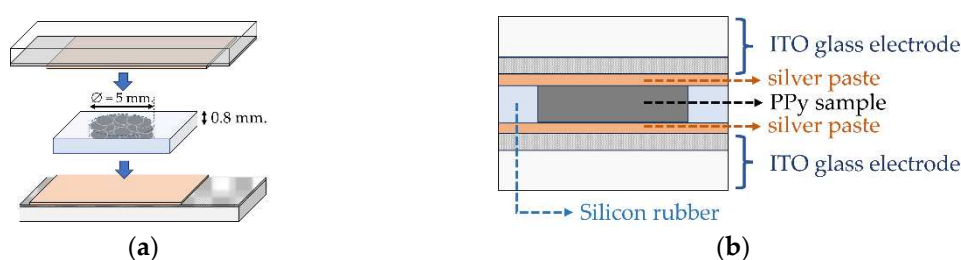
Scheme 3. (a) Two-electrode cell construction for resistance measurement and (b) half-side view of the cells.
