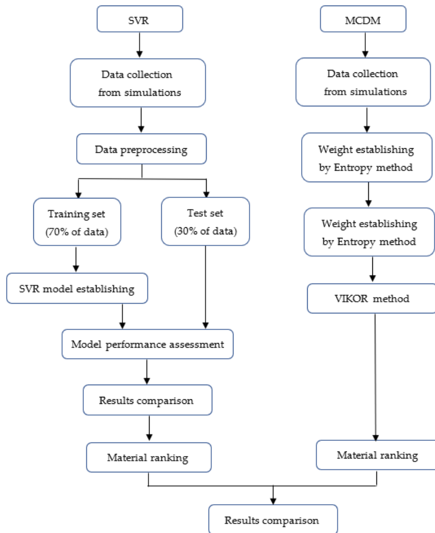
Figure 3. Methodology flowchart.
