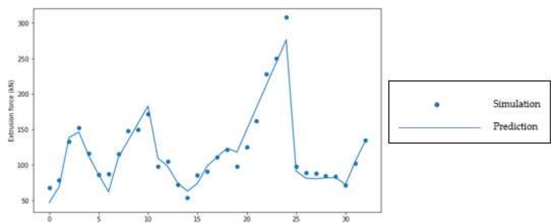
Figure 5. H13 extrusion force prediction comparison.
