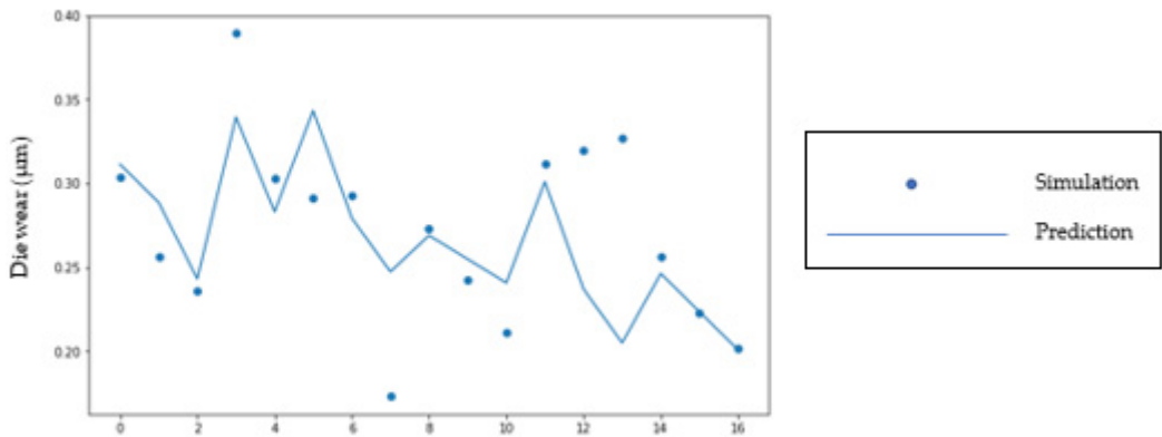
Figure 13. AISI3310 die wear prediction comparison.
