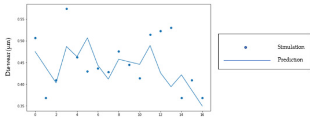
Figure 11. 25CrMo4 die wear prediction comparison.
