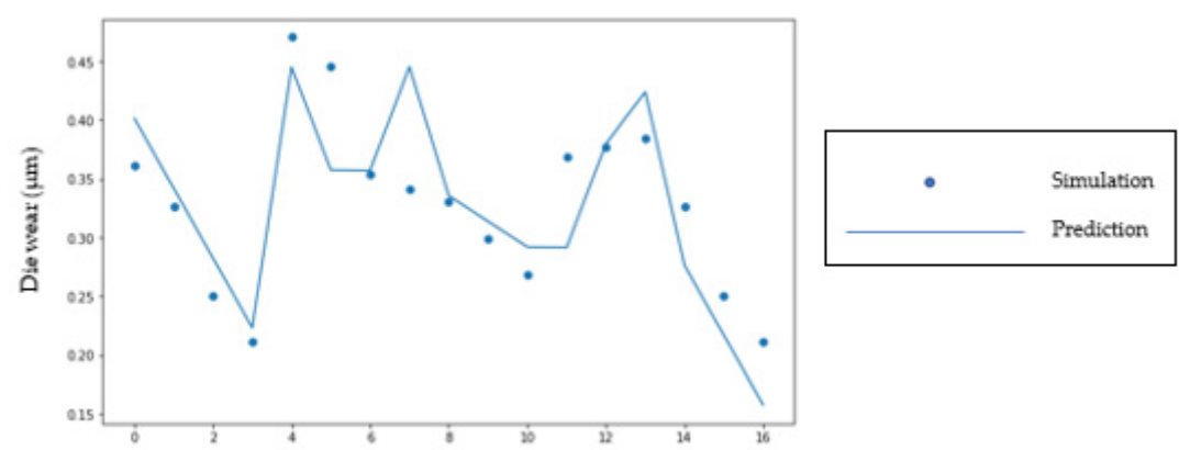
Figure 12. AISI52100 die wear prediction comparison.
