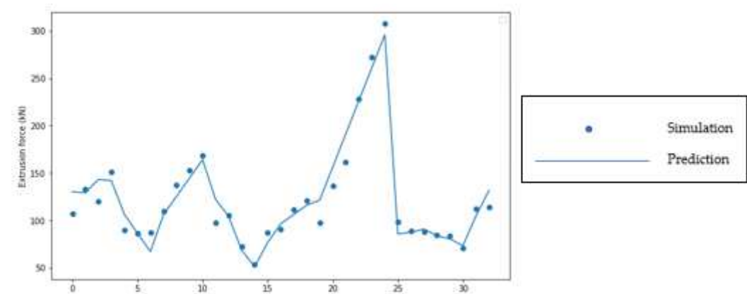
Figure 4. AISI316 extrusion force prediction comparison.
