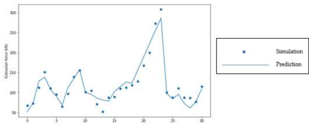
Figure 7. AISI52100 extrusion force prediction comparison.
