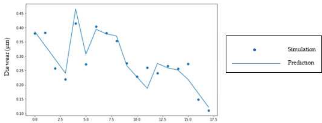
Figure 10. H13 die wear prediction comparison.
