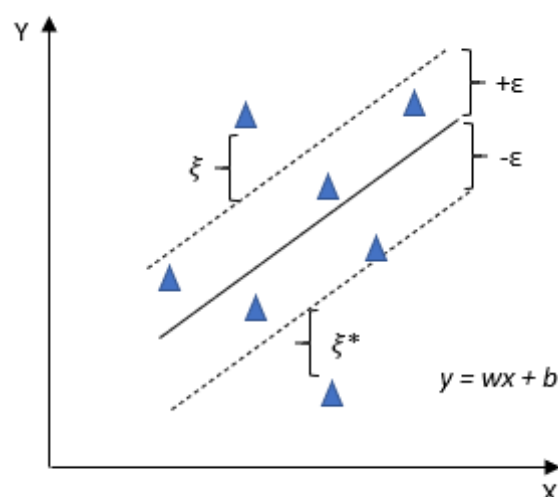
Figure 2. 2D hyperplane representation.
