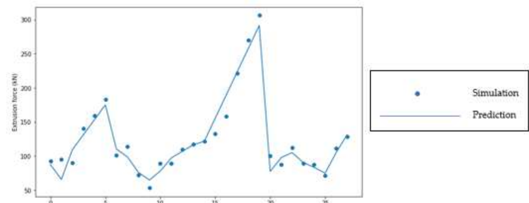
Figure 8. AISI3310 extrusion force prediction comparison.
