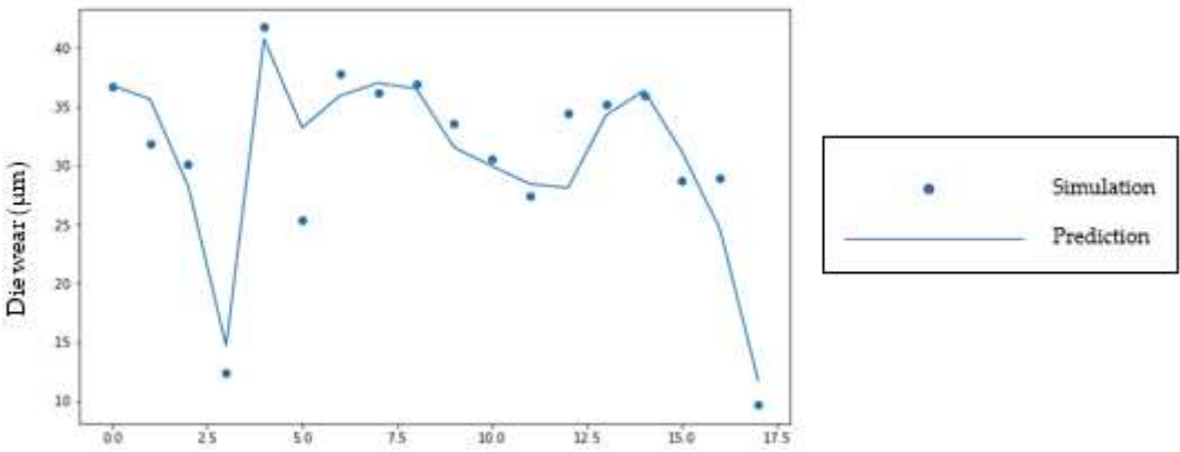
Figure 9. AISI316 die wear prediction comparison.
