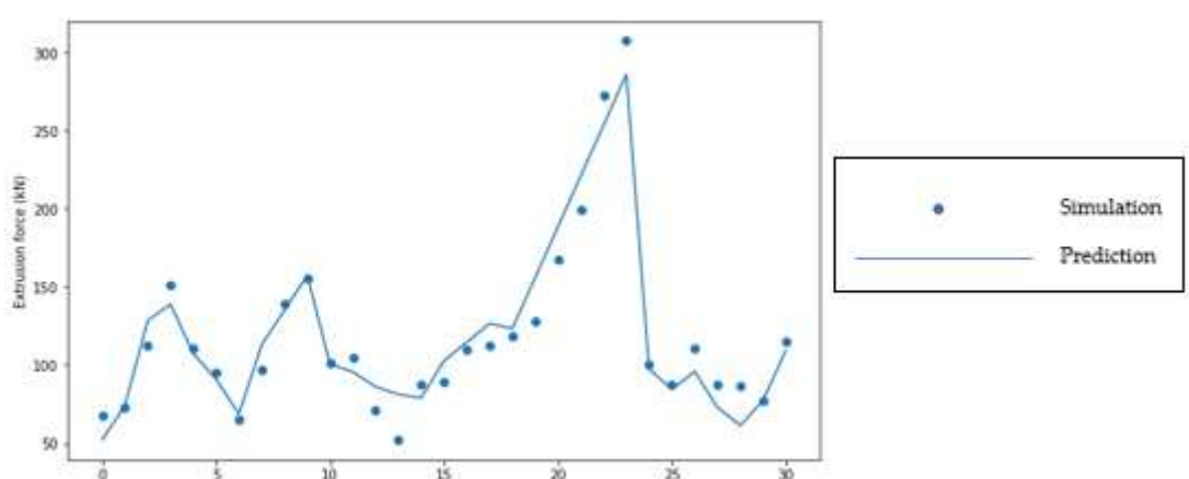
Figure 6. 25CrMo4 extrusion force prediction comparison.
