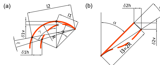
Figure A6. Deformed (a) part 1 or 3 and (b) part 2 of RUCe: continuous line represents undeformed situation and dashed line represents deformed situation
