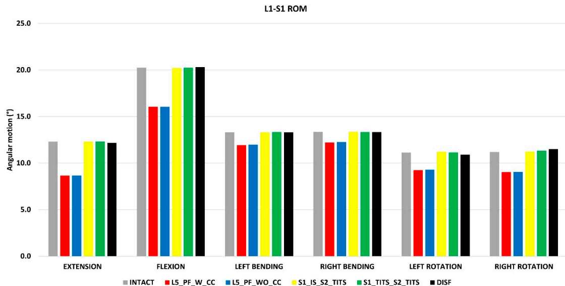
Figure 10. Comparison of L1-S1 ROM at 7.5Nm moment with 400N follower load under two leg stance condition for five different pelvic ring fracture stabilization configurations. The vertical axis is the angle in degrees and the horizontal axis indicates the motions simulated.
