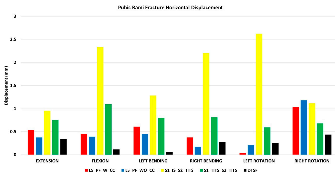
Figure 6. Comparison of Pubic Rami fracture horizontal displacement at 7.5Nm moment with 400N follower load under two leg stance condition for five different pelvic ring fracture stabilization configurations. The vertical axis is the displacement in mm and the horizontal axis indicates the motions simulated.
