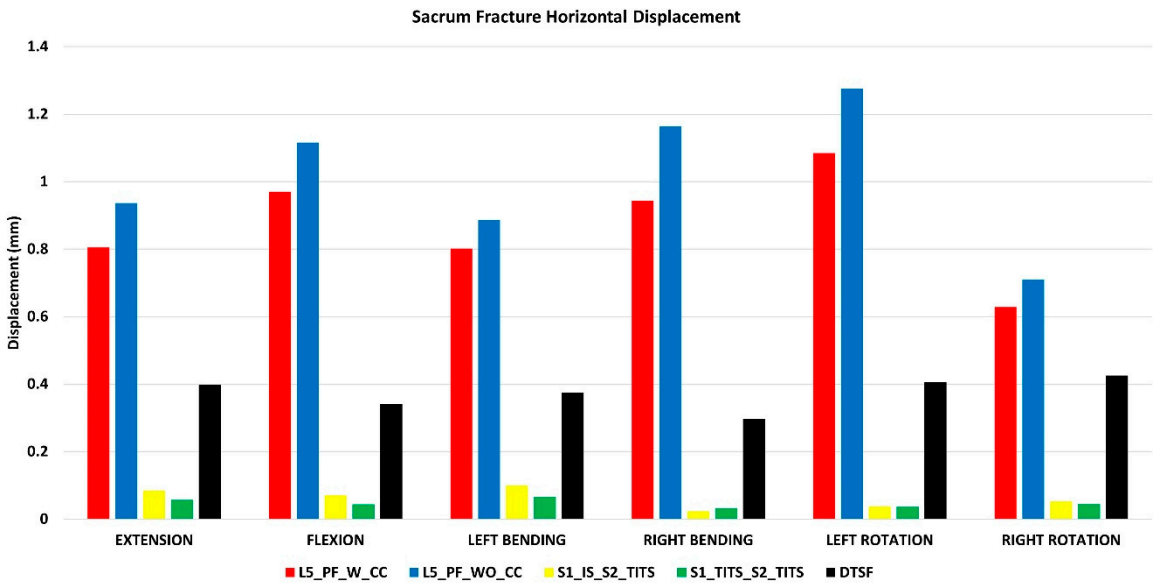
Figure 4. Comparison of sacrum fracture horizontal displacement at 7.5Nm moment with 400N follower load under two leg stance condition for five different pelvic ring fracture stabilization configurations. The vertical axis is the displacement in mm and the horizontal axis indicates the motions simulated.
