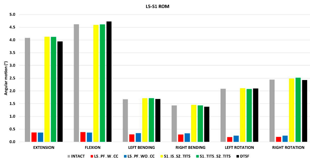
Figure 9. Comparison of L5-S1 ROM at 7.5Nm moment with 400N follower load under two leg stance condition for five different pelvic ring fracture stabilization configurations. The vertical axis is the angle in degrees and the horizontal axis indicates the motions simulated.
