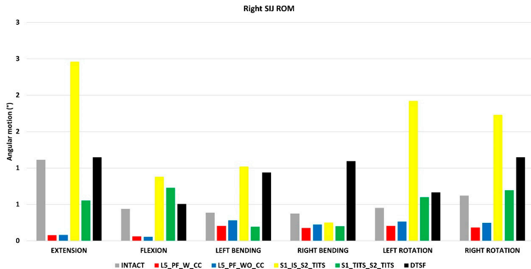
Figure 8. Comparison of right (contralateral to fracture site) SIJ ROM at 7.5Nm moment with 400N follower load under two leg stance condition for five different pelvic ring fracture stabilization configurations. The vertical axis is the angle in degrees and the horizontal axis indicates the motions simulated.
