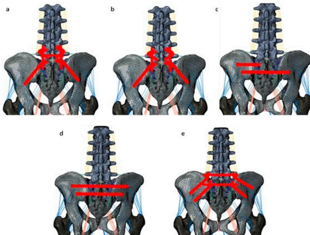
Figure 3. Stabilization of the pelvic ring fracture with various fracture fixation techniques. 3a indicates the L5-ilium fixation with cross connector (L5_PF_W_CC). 3b indicates the L5-ilium fixation without cross connector (L5_PF_WO_CC). 3c indicates the iliosacral screws at S1 and the trans-iliac-trans-sacral screw at S2 (S1_IS_S2_TITS). 3d indicates the trans-iliac-trans-sacral screw at both S1 and S2 (S1_TITS_S2_TITS). 3e indicates the double transiliac rod and screw fixation (DTSF).
