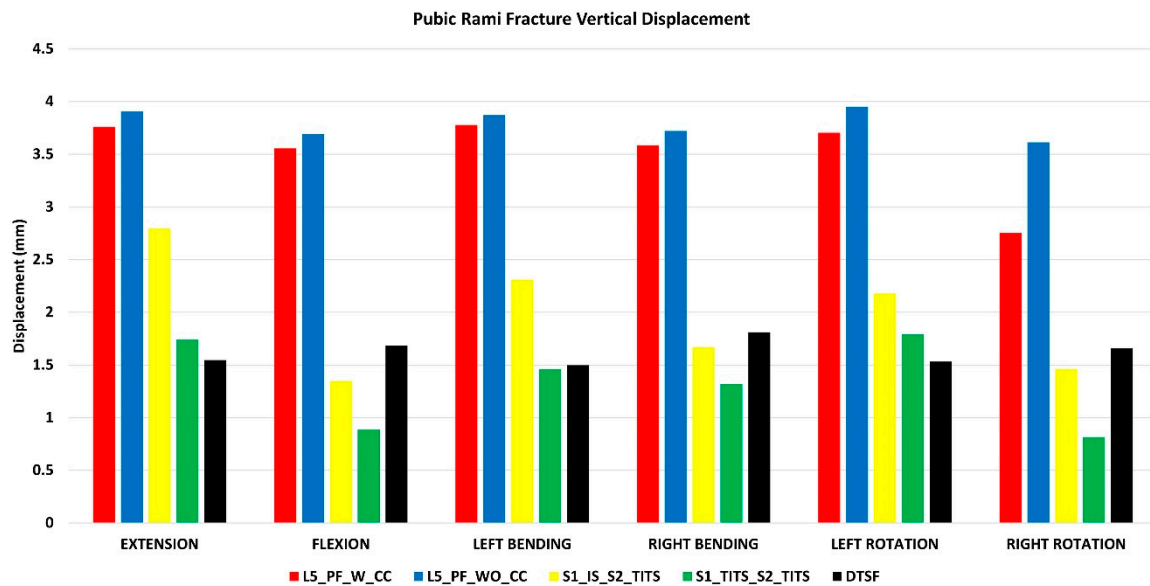
Figure 7. Comparison of Pubic Rami fracture vertical displacement at 7.5Nm moment with 400N follower load under two leg stance condition for five different pelvic ring fracture stabilization configurations. The vertical axis is the displacement in mm and the horizontal axis indicates the motions simulated.
