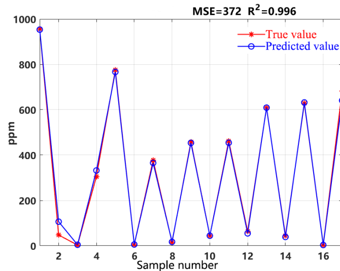
Figure 2. VOCs concentration regression by SVR after PCA of PID signal features.
