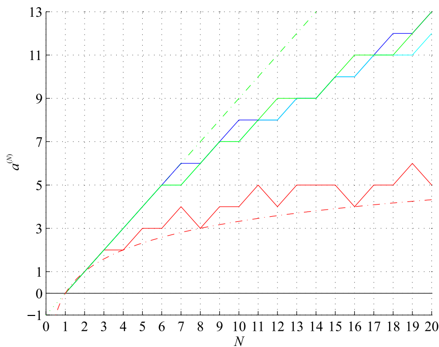
Figure 3. Lower bound on the binary string assembly index 2 (red) and \log_2(N) (red, dash-dot), conjectured upper bound on the binary string assembly index 1 (green), factual values of the string assembly index (blue) and the ringed string assembly index (cyan) and N - 1 (green, dash-dot), for the string length 0 \leq N \leq 20 .
