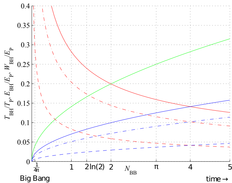
Figure 10. Black body object energy E_{BB} (green); temperature T_{BH} (red), \text{Re}[T_{BB}(k_{eq})] (red, dash-dot), \text{Re}[T_{BB}(k_{max})] (red, dash); and work W_{BH} (blue), \text{Re}[W_{BB}(k_{eq})] (blue, dash-dot), \text{Re}[W_{BB}(k_{max})] (blue, dash), as a function of its information capacity N_{BB} in terms of Planck units, for 0 \leq N_{BB} \leq 5 .
