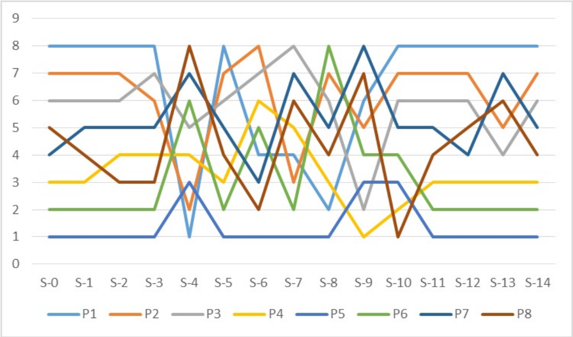
Figure 2. Changes in ranked projects with changes in the value of criteria weights
