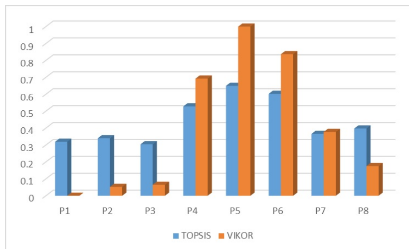
Figure 3. Ranked projects by VIKOR and TOPSIS methods
