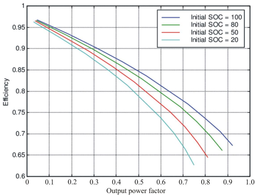
Figure 2. Discharge efficiency of lithium batteries as a function of the state of charge.
