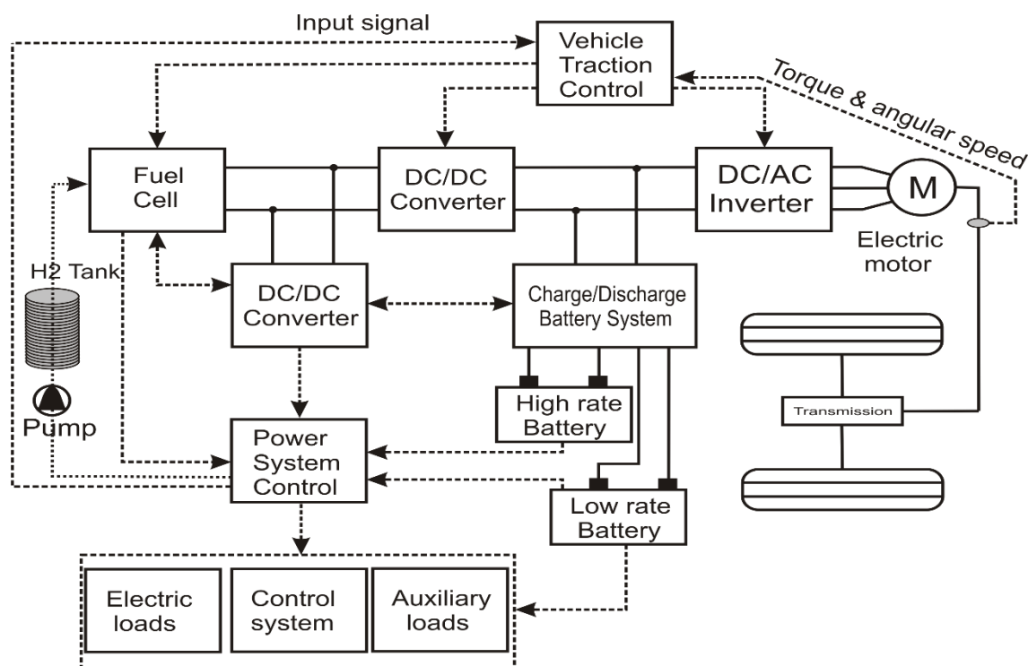
Figure 4. Schematic view of a Hybrid Fuel Cell-Lithium Battery Power System for Electric Vehicles.
