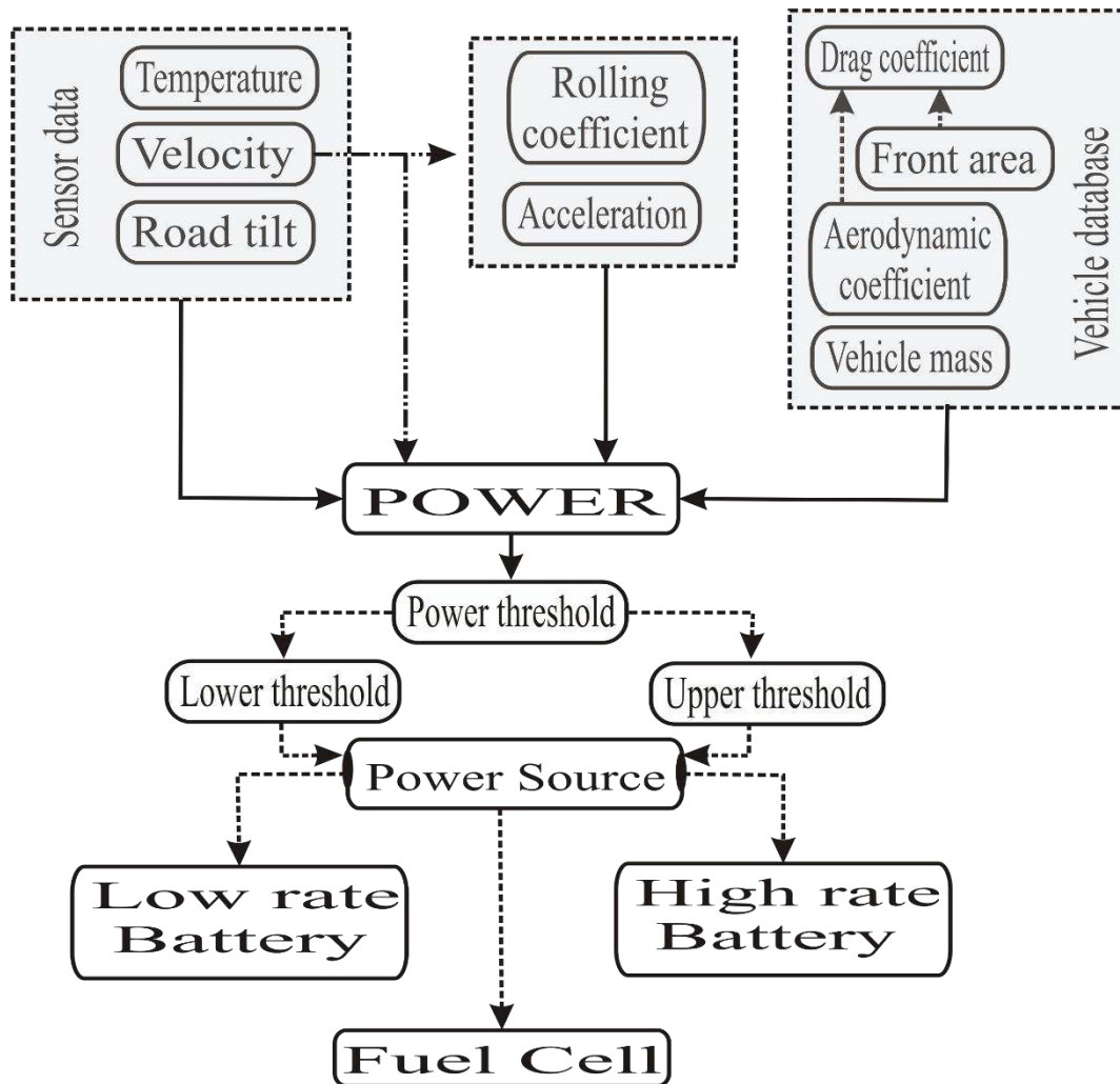
Figure 3. Control System Flowchart.
