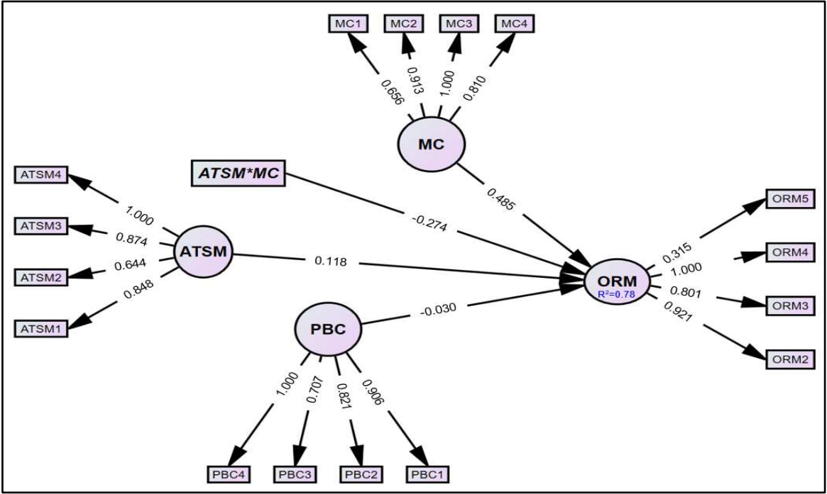
Figure 2. Modified SEM Structural model with unstandardized path coefficients and regression weights.
