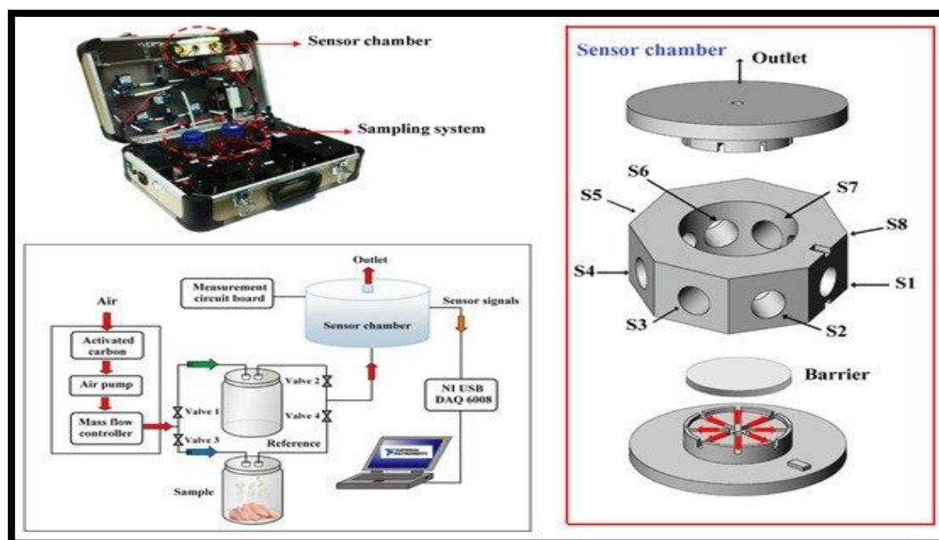
Figure 1. Image and schematic diagram of a portable E-nose system prototype.
