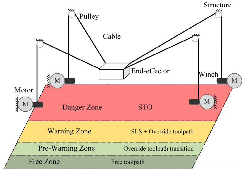
Figure 10. Proposed zones for a Collaborative CDPR prototype implementation.
