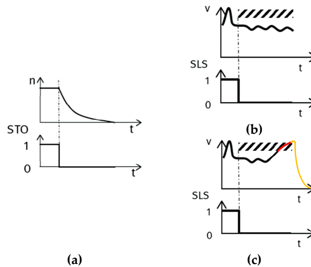
Figure 3. Safe motion monitoring functionalities examples: (a) STO; (b) SLS with activation of the speed limit; (c) SLS with activation and speed limit exceedance.
