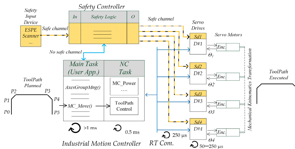
Figure 1. Reference architecture for safe servo-driven industrial systems.
