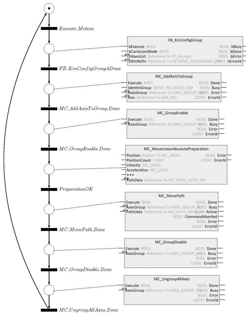
Figure 4. Sequence process control for executing toolpaths in a suspended 4-cable CDPR configuration in TwinCAT 3 with legacy Beckhoff resources.
