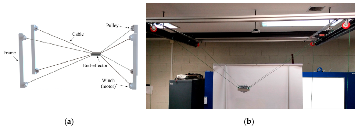
Figure 2. Example of CDPR configurations: (a) 8-cables fully-constrained (position cannot change without changing the length of the cables); (b) Photo of the developed 4-cables suspended (position can be different even subject to the same cable lengths).
