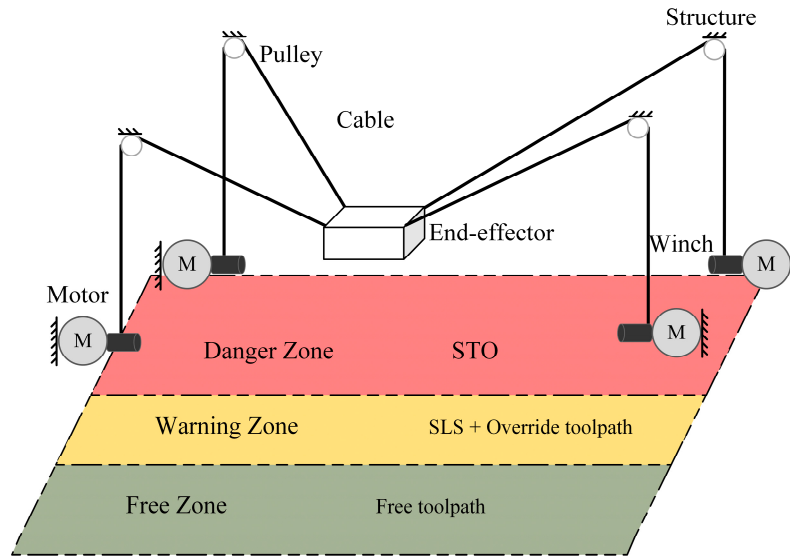
Figure 6. Zones definitions for a Collaborative CDPR prototype implementation.
