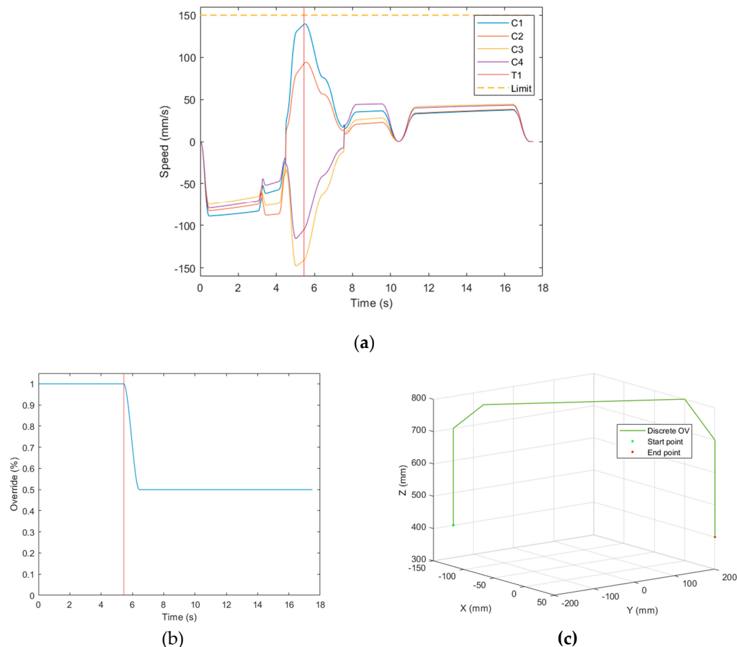
Figure 8. Result of performing the trajectory when a person entered the Warning Zone, triggering the activation of the SLS safety function and a speed override of the axes group. The vertical red line ("T1") indicates when an operator entered the Warning Zone. (a) Time evolution of the speed on each axis (cable); (b) Time series of the discrete speed override (level 50%); (c) 3D view of the toolpath.
