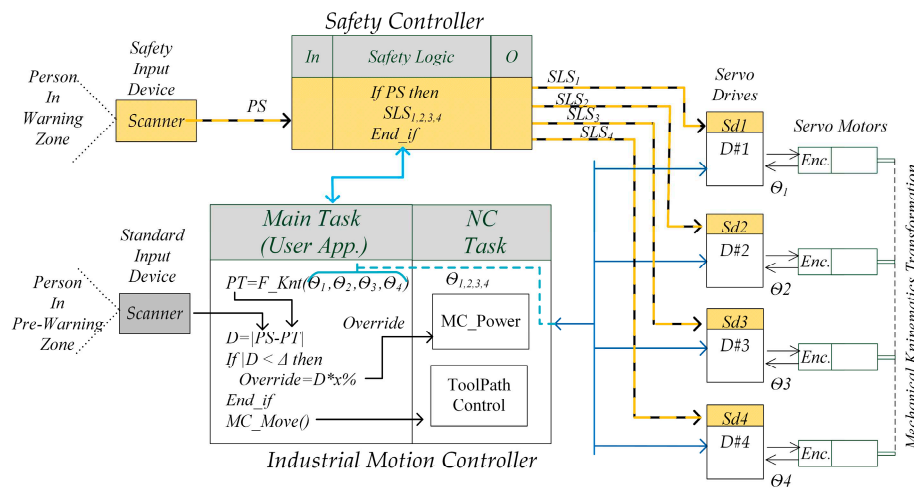
Figure 5. Proposed reference architecture for the experiment.
