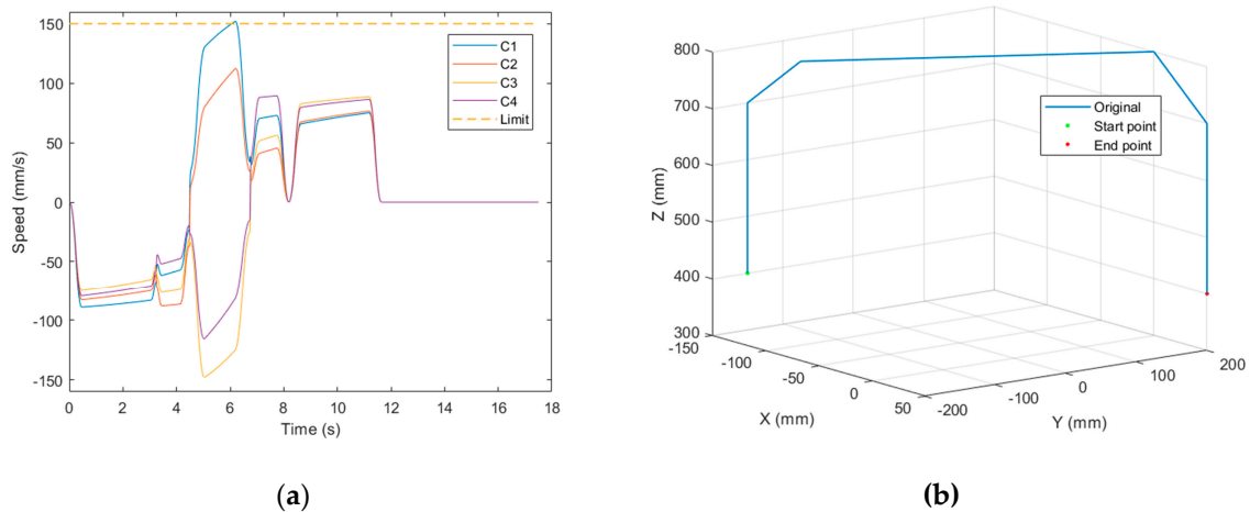
Figure 7. Result of performing the trajectory under normal conditions (with the operator standing in the "Free Zone"): (a) Time series of the velocity on each axis (cable); (b) 3D view of the toolpath.
