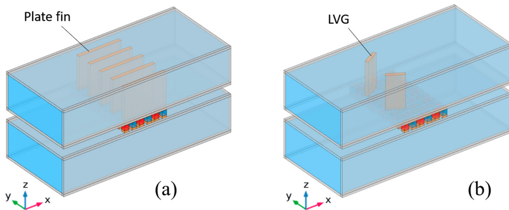
Figure 2. Schematic diagram of the TEG installed in (a) a heat exchanger with flat plate fins and (b) a heat exchanger with LVG.
