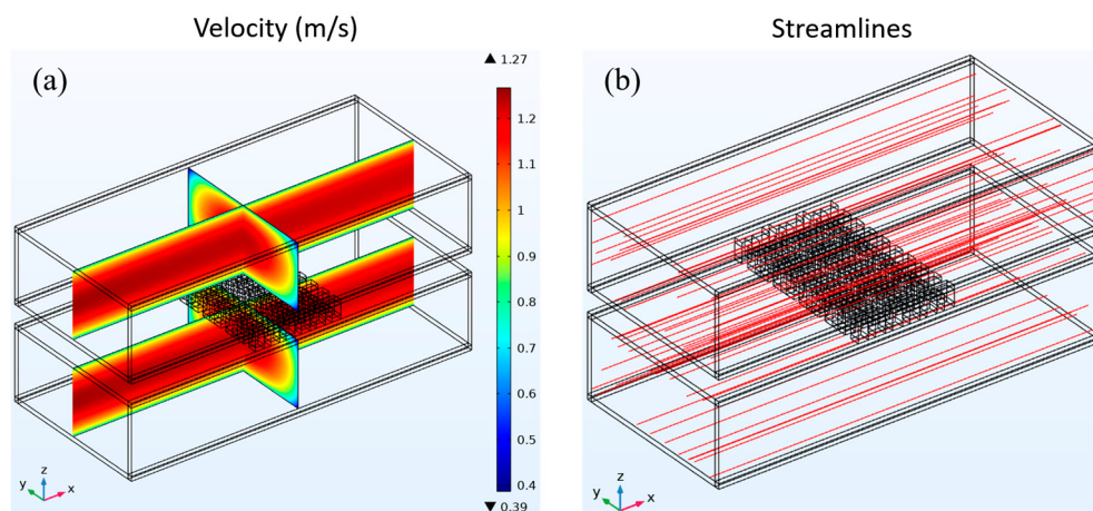
Figure 4. (a) Fluid velocity distribution and (b) streamline distribution in a cavity-type heat exchanger.
