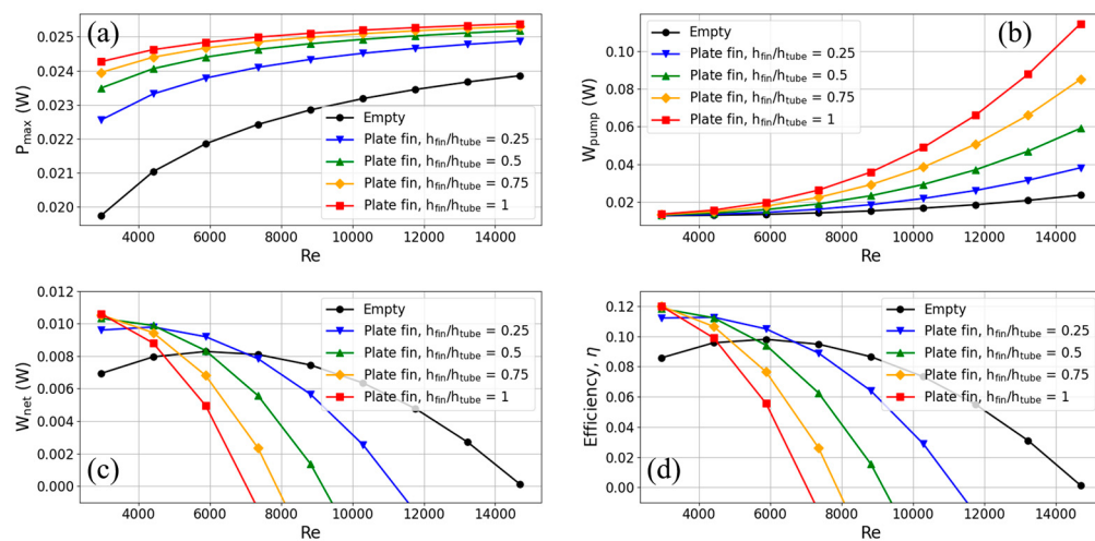
Figure 10. Trends of (a) maximum output power, (b) pump power, (c) net output power, and (d) thermoelectric conversion efficiency with Reynolds number for TEG installed in a heat exchanger with flat plate fins.
