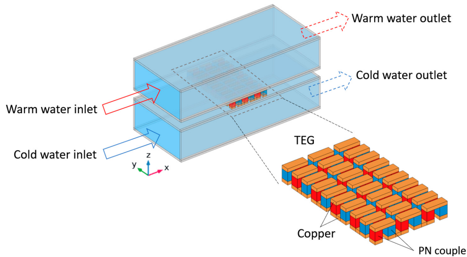
Figure 1. Schematic diagram of the TEG installed in a cavity-type heat exchanger.
