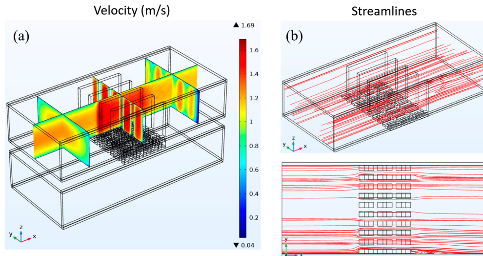
Figure 5. (a) Fluid velocity distribution and (b) streamline distribution in a heat exchanger with flat plate fins.
