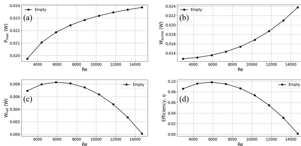
Figure 9. Trends of (a) maximum output power, (b) pump power, (c) net output power, and (d) thermoelectric conversion efficiency with Reynolds number for TEG installed in a cavity-type heat exchanger.
