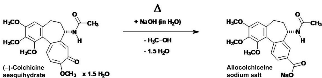
Scheme 3. The possible side product in the synthesis of compound 2 , the allocolchicine (syn. colchinoic acid, colchicinoic acid, colchicic acid) monosodium salt, originating from hydrolytic ring C contraction by a benzylic-type rearrangement.
