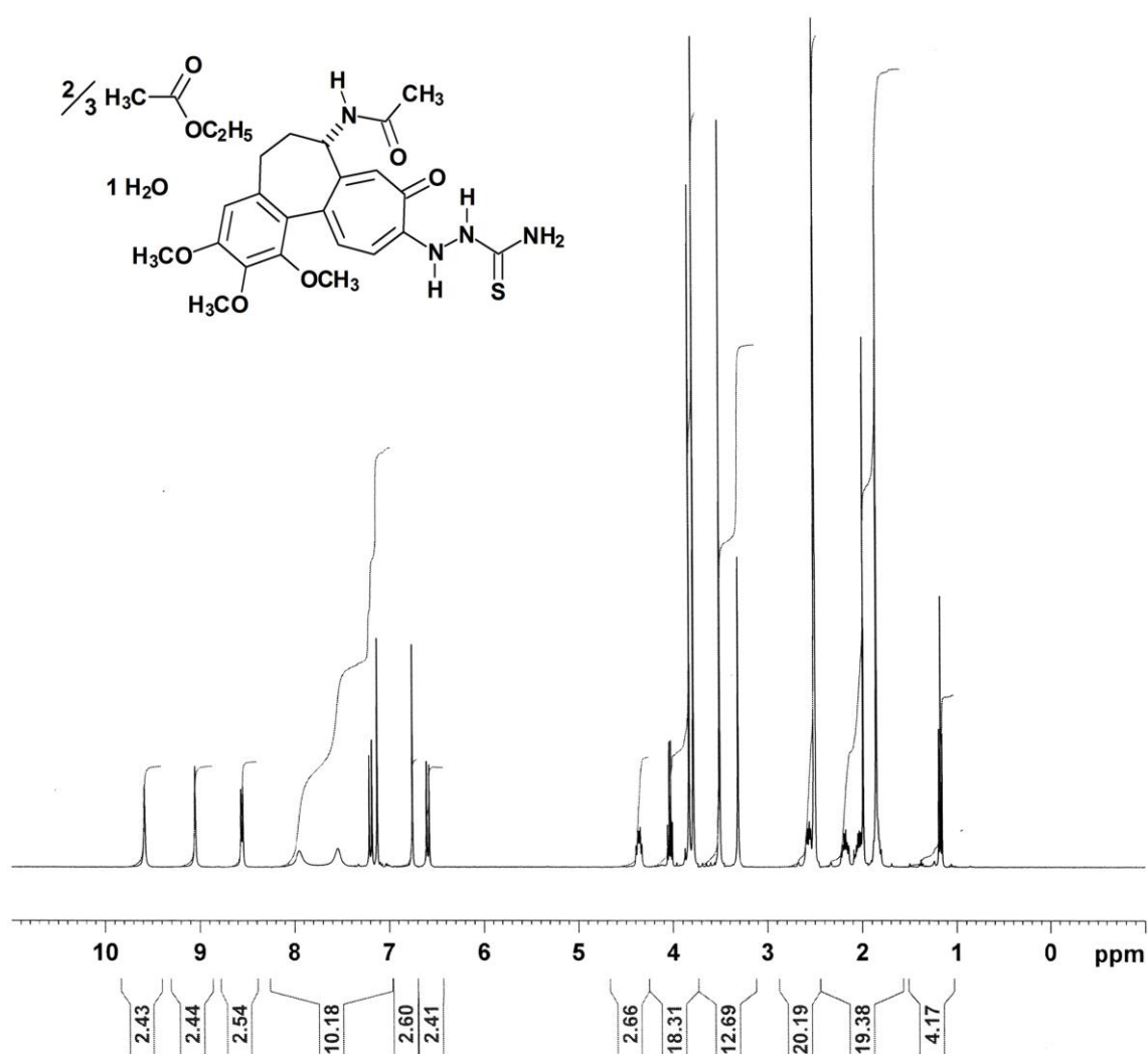
Figure 5. The 400.13 MHz ^1\text{H} -NMR spectrum (in \text{DMSO}-d_6 ) [ \text{DMSO}-d_6 quintet at \delta 2.50 ppm, ^2J_{\text{gem}}(^1\text{H}-^1\text{H}) = +1.9 Hz; water at \delta 3.32 ppm] of the colchic(in)oid 10-(2-carbamothioylhydrazinyl)-10-
