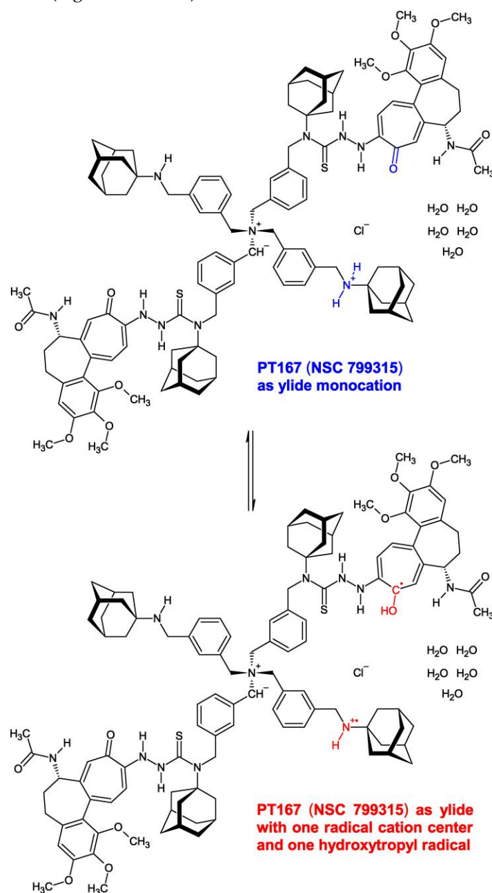
Figure 14. The electron transfer in compound 3 yielding a partially paramagnetic molecular species. The colchic(in)oid part of the molecule picks up one electron from the ylide monocation yielding a
