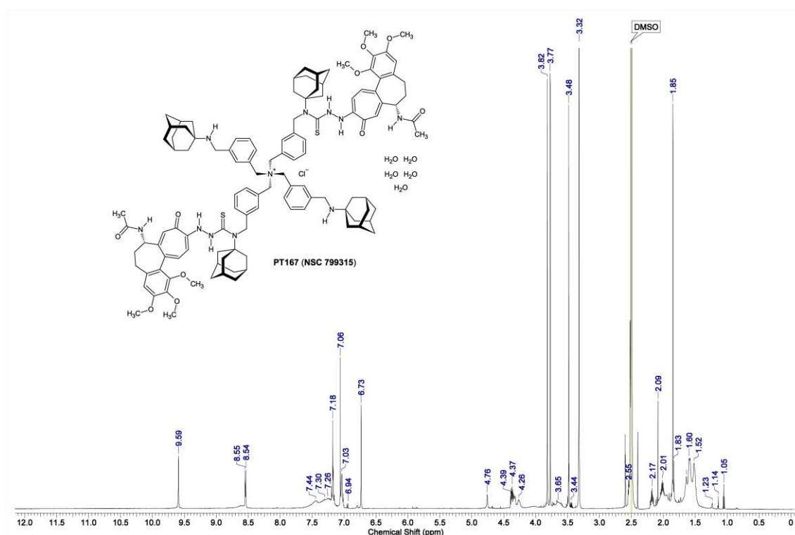
Figure 10. The organic chemical structure formula of compound 3 [PT167 (NSC 799315)] = C_{116}H_{142}N_{11}O_{10}S_2^+ \times Cl^- \times 5 H_2O = C_{116}H_{152}ClN_{11}O_{15}S_2 ( M = 2040.10 g/mol). The compound 3 contains one chloride anion ( Cl^- ) and five water of crystallization ( \times 5 H_2O ).
