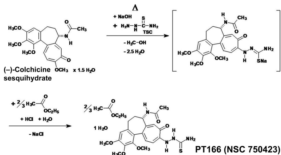
Scheme 2. The synthesis of the modified colchic(in)oid 10-(2-carbamothioylhydrazinyl)-10-demethoxycolchicine monohydrate \times \frac{2}{3} (ethyl acetate) (compound 2 , PT166, NSC 750423) by NaOH-catalysed amidation (amino-de-alkoxylation) of the vinylogous (tropolonic) carboxylic acid methyl ester (–)-colchicine. Methanol was split off by thiosemicarbazide (TSC) from (–)-colchicine during short refluxing. Subsequently, the product compound 2 was liberated from a monosodium salt intermediate by acidification with hydrochloric acid and extraction with ethyl acetate. The term colchic(in)oid is now well accepted and documented in literature [36].
