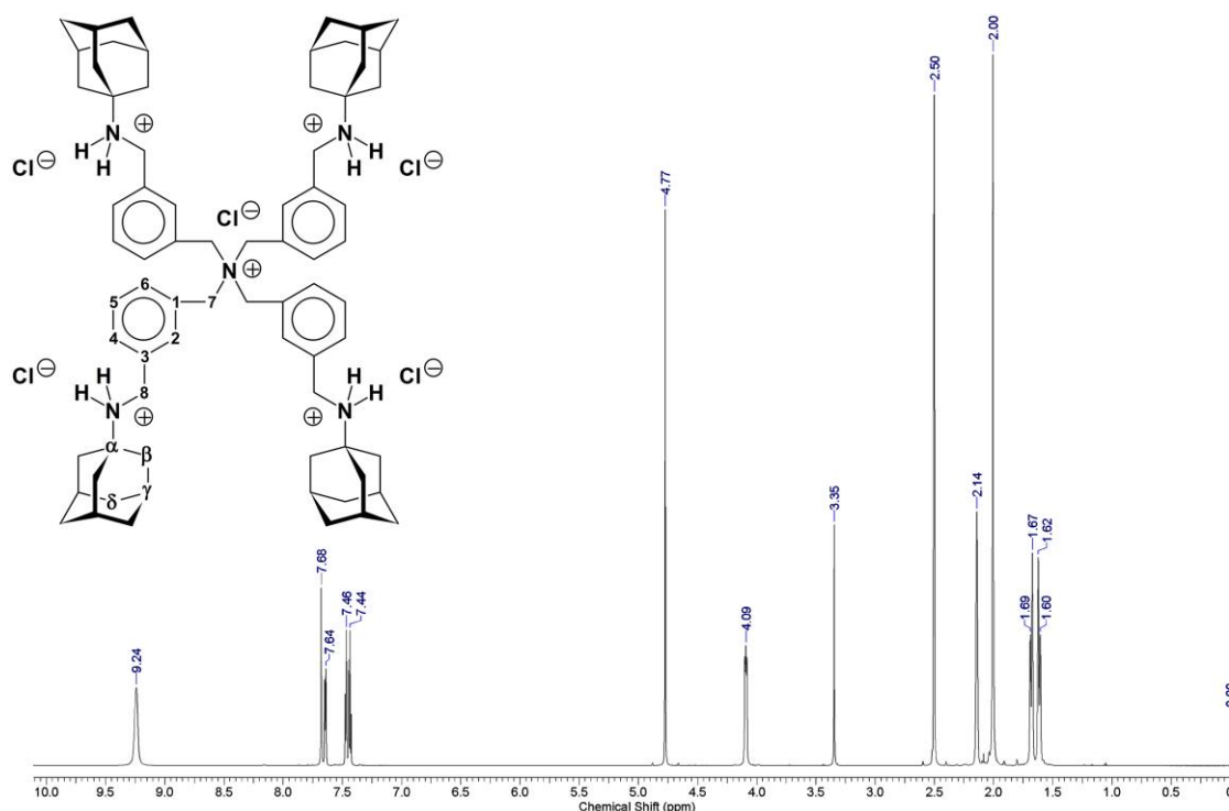
Figure 3. The 700.43 MHz ^1\text{H} -NMR spectrum (in \text{DMSO-}d_6 ) of the pure polyammonium polycation tetrakis{3-[(tricyclo[3.3.1.1. 3,7 ] decan-1-ammonio)methyl]benzyl}ammonium pentachloride = pure (salt-free) compound 1 [PT162 (NSC 796018)] [ \text{DMSO-}d_5 quintet at \delta 2.50 ppm, ^2J_{\text{gem}}(^2\text{H-}^1\text{H}) = +1.9 Hz; water at \delta 3.35 ppm].
