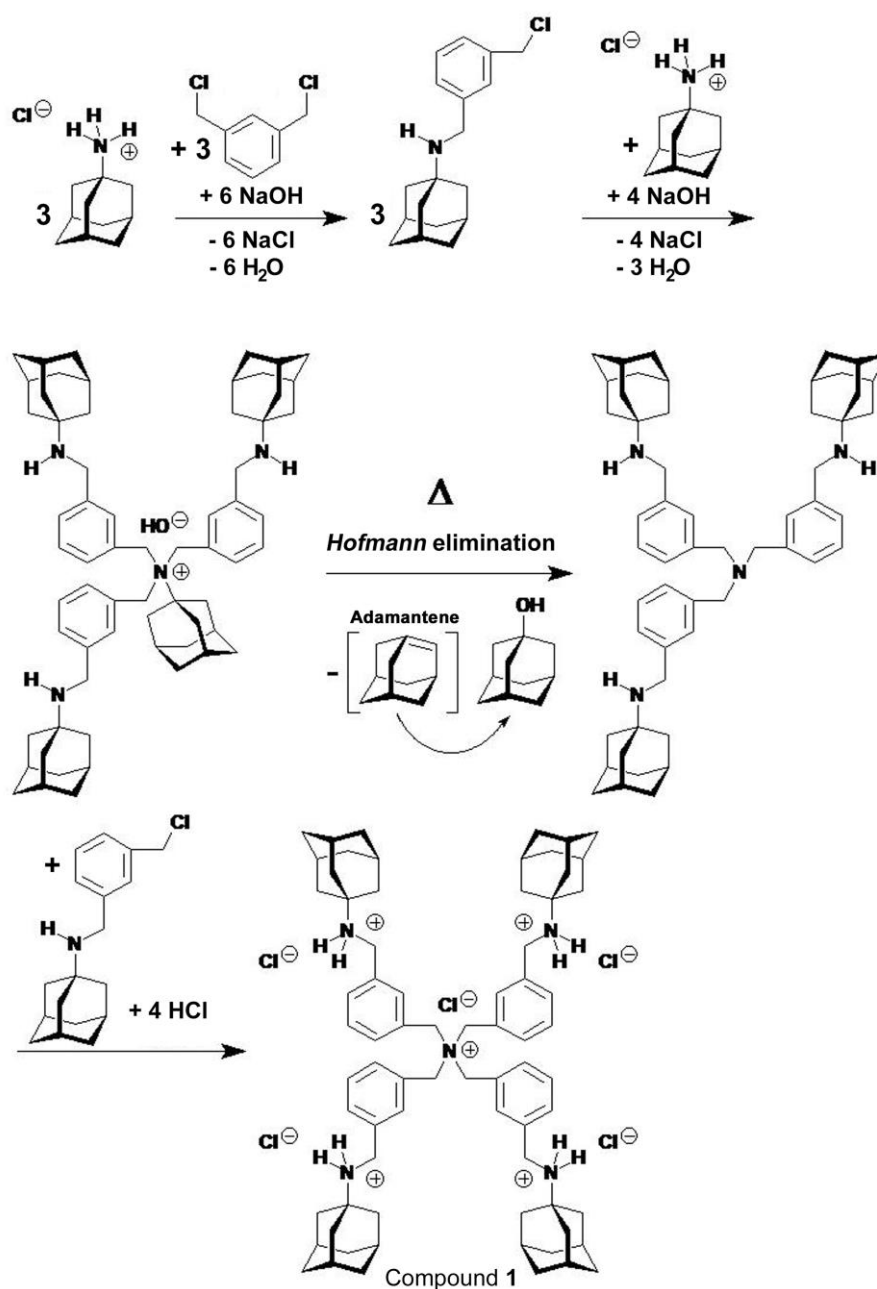
Scheme 1. The synthesis of the polyammonium polycation compound 1 from 1-aminoadamantane \times HCl and 1,3-bis(chloromethyl)benzene. The intermediate N -[3-(chloromethyl)benzyl]-1-adamantanamine reacted with amantadine \times HCl under influence of NaOH to N,N,N -tris[3-[(tricyclo[3.3.1.1 3,7 ]decan-1-ylamino)methyl]benzyl]-1-adamantanammonium hydroxide, which in
