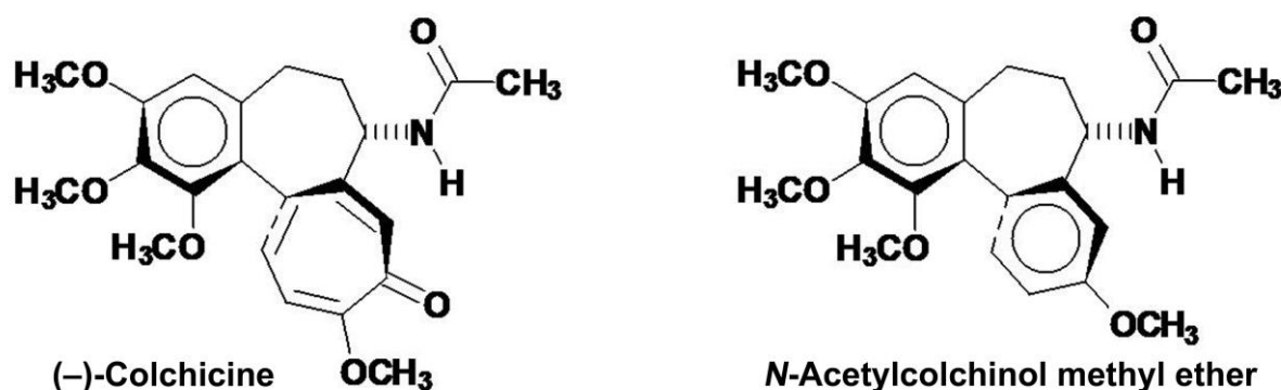
Figure 6. The atropisomerism of natural (–)-colchicine and its degradation product N -acetylcolchinol methyl ether. Both exhibit the (aS,7S)-absolute configuration, as was proved by Brossi et al. [62,63].
