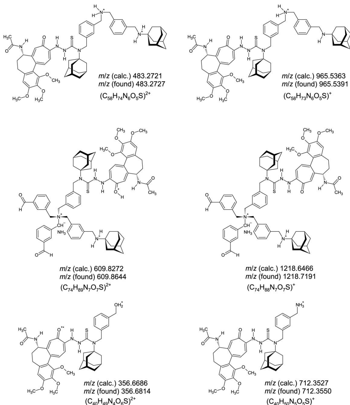
Figure 16. The six structure-proofing fragment cations (left, dications; right, monocations) in the electrospray ionization (ESI) time-of-flight (ToF) mass spectrometric investigation of compound 3 after storing the substance over six years at +0–4 °C in the refrigerator. The m/z 483.2727 (100%) (generated from ylide dication), m/z 965.5391 (80.9%) (generated from ylide dication), m/z 609.8644 (31.0%) (generated from ylide monocation), m/z 1218.7191 (5.0%) (generated from ylide monocation), m/z 356.6814 (19.1%) (generated from ammonium monocation), and m/z 712.3550 (100%) (generated from ammonium monocation) are the major, structure-proofing fragments of compound 3 .
