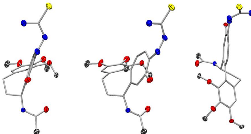
Figure 9. The helical axis atropisomerism view of one independent, isolated molecule of compound 2 as found in the single crystal. Compound 2 , the colchic(in)oid N -[(aS,7S)-10-(2-carbamothioylhydrazinyl)-1,2,3-trimethoxy-9-oxo-5,6,7,9-tetrahydrobenzo[ a ]heptalen-7-yl]acetamide, is helical stereogenic and shows the [ M(inus) ]-helicity. Priority rules [64,65] show the helical axis turn in ( S ).
