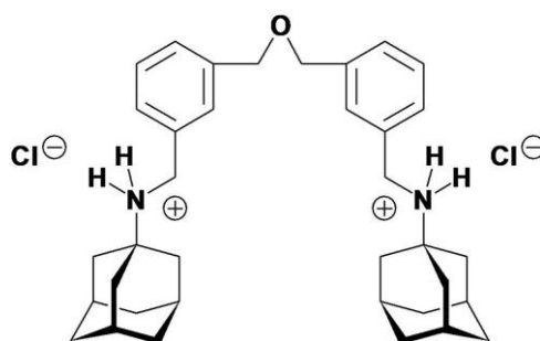
Figure 2. The structure of the dibenzyl ether derivative di{3-[(tricyclo[3.3.1.1 3,7 ]decan-1-ammonio)methyl]benzyl}ether dichloride. This hypothetical structure was considered as alternative reaction product in the synthesis of compound 1 .
