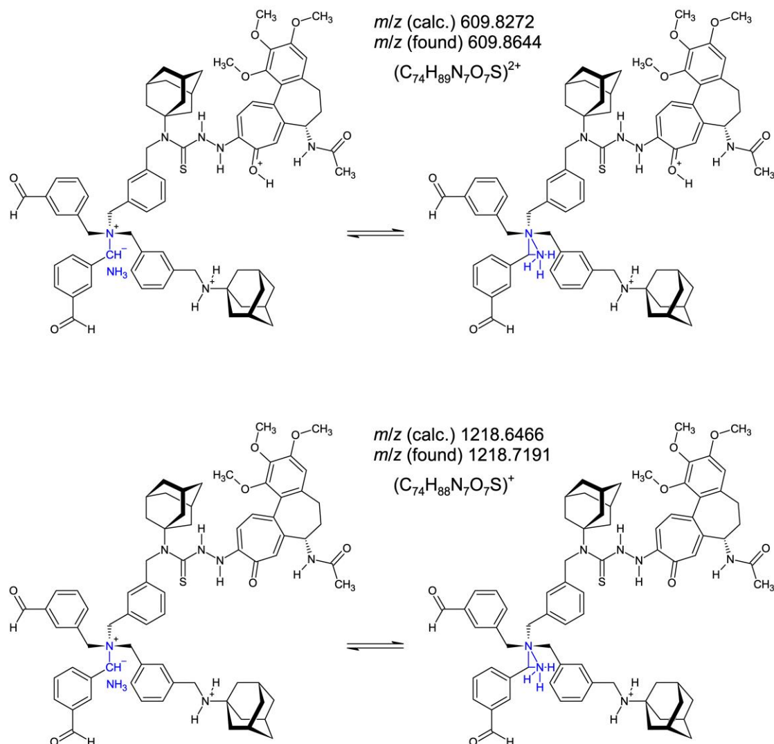
Figure 17. The two cations (C_{74}H_{89}N_7O_7S)^{2+} m/z 609.8644 (31.0%) [generated from of compound 3 ylide monocation] and (C_{74}H_{88}N_7O_7S)^{+} m/z 1218.7191 (5.0%) [generated from of compound 3 ylide monocation] (see Figure 16) are to be formulated as ammonia ( NH_3 )-stabilized [73,74] nitrogen ylides [75] (left, in blue) being in equilibrium with a mass spectrometric enabled species characterized by twice pentavalent nitrogen [76–78] (right, in blue).
