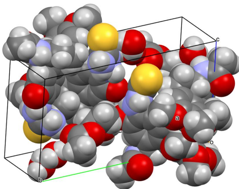
Figure 8. Crystal packing in the monoclinic (space group P2_1 ) unit cell ( Z = 2 ) of compound 2 crystallized as hydrate (ethyl acetate) solvate ( 2 \text{ C}_{22}\text{H}_{26}\text{N}_4\text{O}_5\text{S} \times 3 \text{ H}_2\text{O} \times \text{C}_4\text{H}_8\text{O}_2 ) \text{C}_{48}\text{H}_{66}\text{N}_8\text{O}_{15}\text{S}_2 ( M = 1059.21 \text{ g/mol} ). Unit cell dimensions ( a , b , c are indicated from the origin o ): a = 9.1886(5) \text{ \AA} , b = 20.9047(10) \text{ \AA} , c = 13.9841(7) \text{ \AA} , \alpha = 90.00^\circ , \beta = 106.153(2)^\circ , \gamma = 90.00^\circ , V = 2580.1(2) \text{ \AA}^3 .
