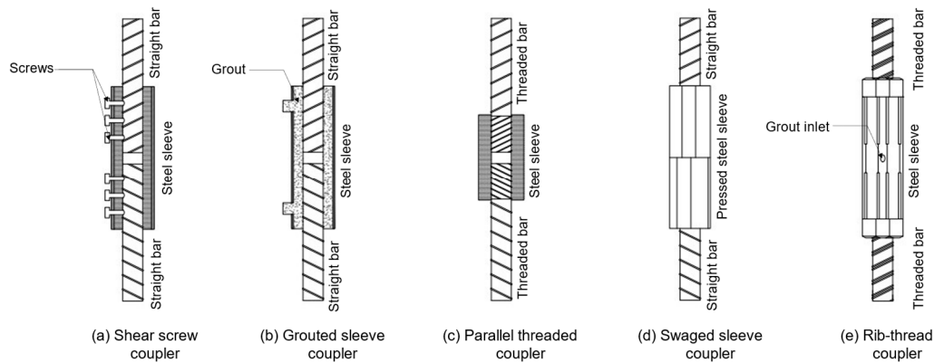
Figure 1. Market-ready mechanical couplers.
