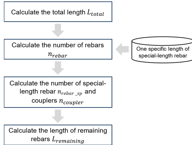
Figure 6. Steps taken in the 3 rd module of the algorithm.
