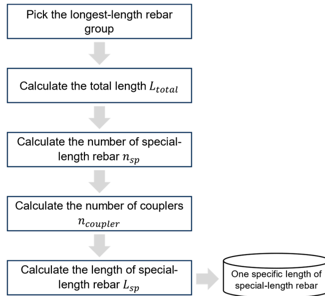
Figure 4. Steps taken in the 2 nd module of the algorithm.
