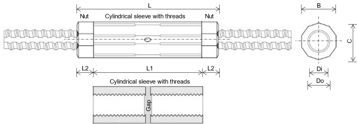
Figure A1. Details of a rib thread coupler [40].
