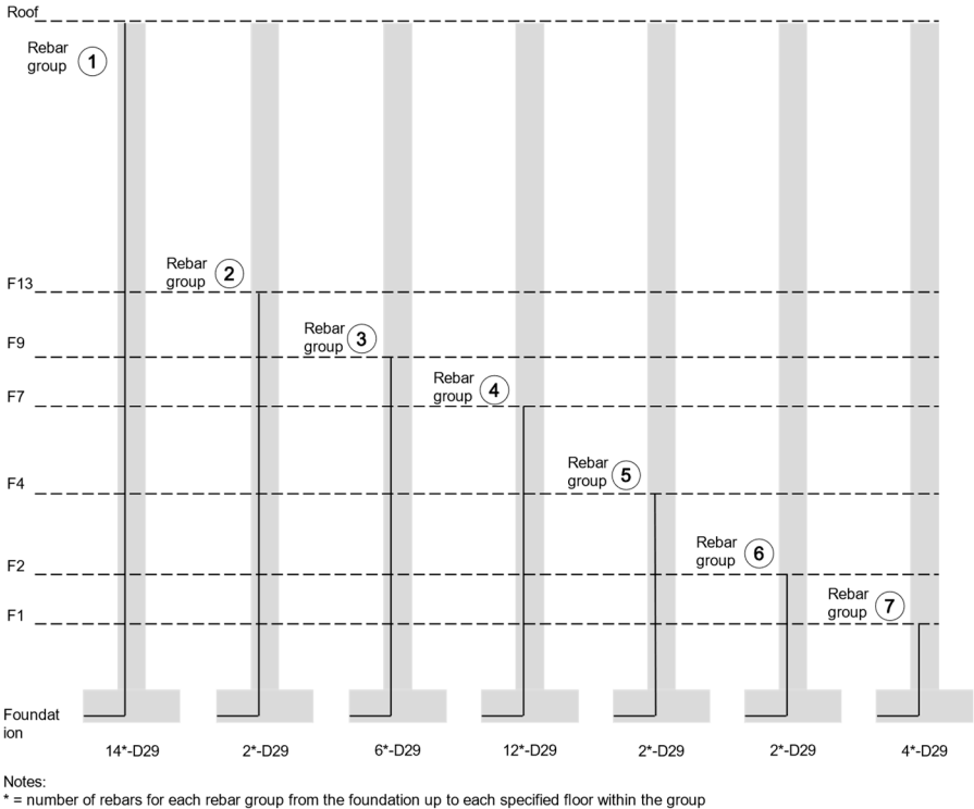
Figure 7. Rebar groups with similar lengths (adapted from [9]).
