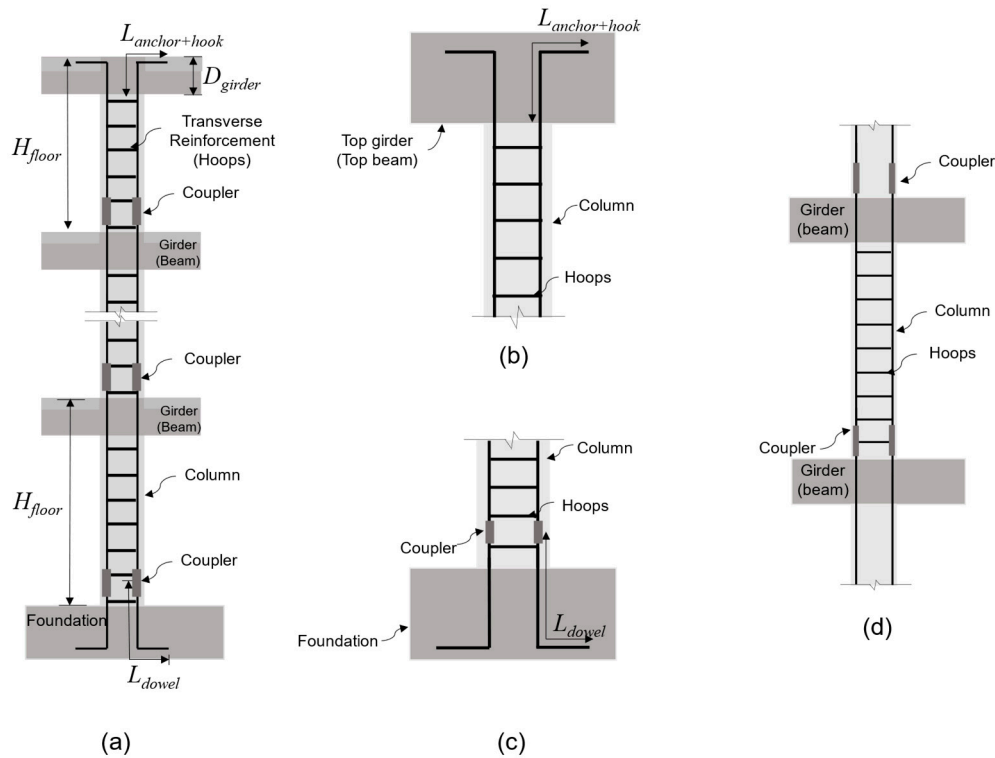
Figure 2. (a) Common column rebar arrangement with couplers; (b) detail of top-anchored rebar; (c) detail of foundation–column connection; (d) detail of couplers between floors (modified from [9]).
