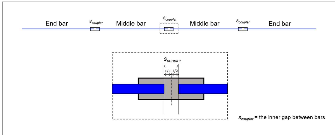
Figure 5. Illustration of coupler's inner gap.
