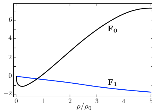
Figure 12. Landau Fermi liquid parameters derived from the quasiparticle properties that are based on the median of the data-inferred baryon chemical potential \mu (see Fig.3).
