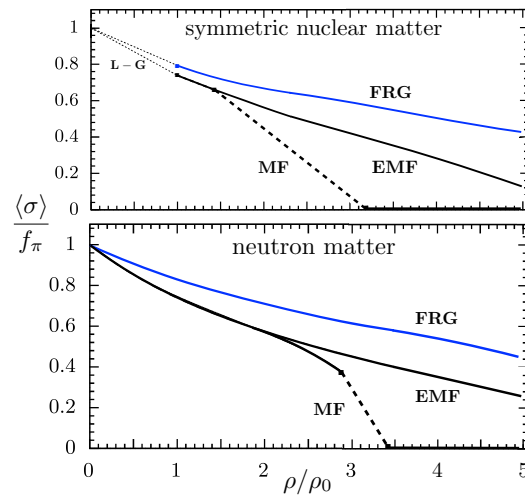
Figure 10. Chiral order parameters in symmetric nuclear matter and neutron matter at temperature T = 0 as function of baryon density in units of nuclear ground state equilibrium density, \rho_0 = 0.16 \text{ fm}^{-3} . Dotted lines: liquid-gas phase transition (L-G) in symmetric nuclear matter. Dashed lines: first-order chiral phase transitions emerging from the mean-field (MF) approximation of a relativistic chiral nucleon-meson (ChNM) field-theoretical model. Solid lines show results of extended mean-field calculations (EMF, with inclusion of fermionic vacuum fluctuations), and functional renormalization group calculations (FRG), based on the same ChNM model. Figures adapted from Refs. [70,71].
