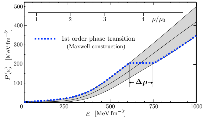
Figure 8. Illustration of the constraint on the maximum width of a Maxwell-constructed coexistence region for a first-order phase transition within the 68% credible band of P(\varepsilon) (see Figure 2) following ref. [27].
