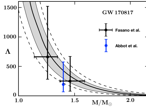
Figure 6. Posterior credible bands [27] of the tidal deformability as a function of neutron star mass, at 68% level (grey band) and 95% level (dashed lines), compared to values [12,35] deduced from the merger event GW170817.
