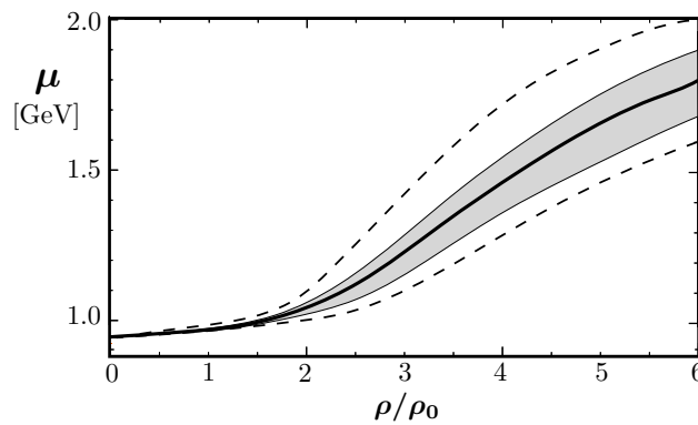
Figure 3. Baryon chemical potential \mu(\rho) in neutron star matter, normalized at \mu(\rho = 0) = 939 \text{ MeV} . Shown are posterior credible bands [27] at 68% level (grey band) and 95% level (dashed lines). 2.
