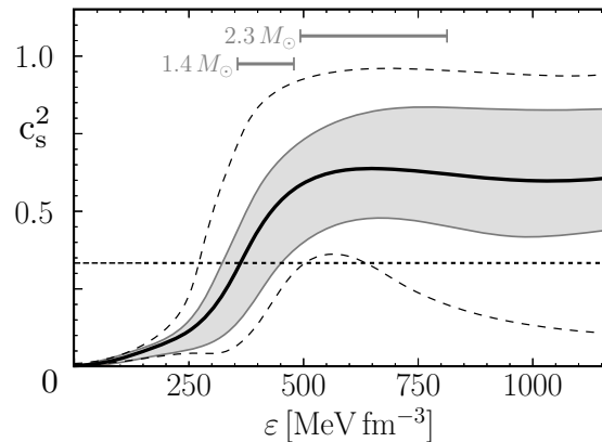
Figure 1. Squared speed of sound [27] as function of energy density inferred from the empirical data set listed in Section 2.1. Median (solid curve) and posterior credible bands at levels of 68% (grey band) and 95% (dashed curves) are displayed. Intervals are indicated for 68% ranges of central energy densities in the cores of 1.4 and 2.3 M_{\odot} neutron stars.
