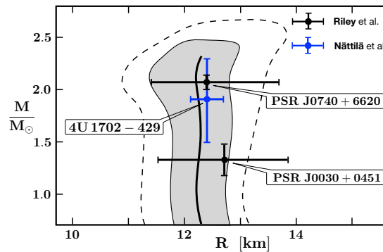
Figure 5. Posterior credible bands [27] of the mass-radius relation at 68% level (grey band) and 95% level (dashed line), compared to the NICER data analysis by Riley et al. of PSR J0030+0451 and PSR J0740+6620 [7,9]. In addition the 68% mass-radius credible interval of the thermonuclear burster 4U 1702-429 (blue) is displayed [37] (which was not included in the Bayesian analysis).
