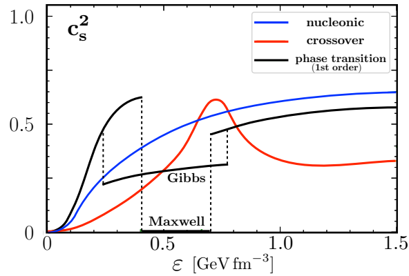
Figure 7. Characteristic behaviours of the squared sound velocity in the presence of a phase transition or a crossover.
