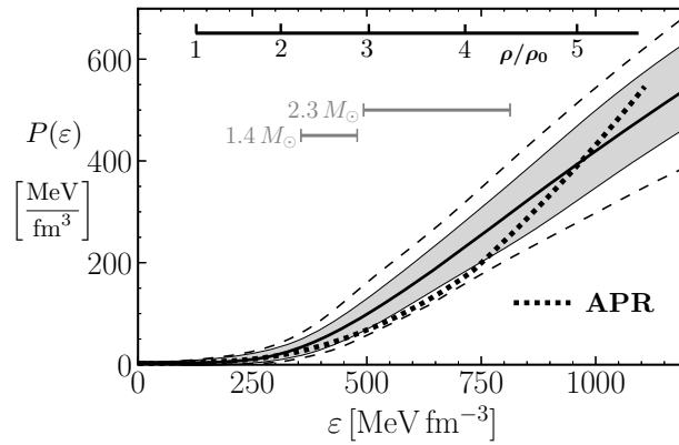
Figure 2. Equation of state P(\varepsilon) [27] deduced from the inferred sound velocity based on the empirical data set listed in Section 2.1. Median, 68% and 95% posterior credible bands are displayed as in Figure 1. The APR EoS [36] (dotted line) is shown for comparison. Also shown for orientation is the baryon density scale, \rho/\rho_0 (in units of the equilibrium density of nuclear matter \rho_0 = 0.16 \text{ fm}^{-3} ), computed for the median of P(\varepsilon) .
