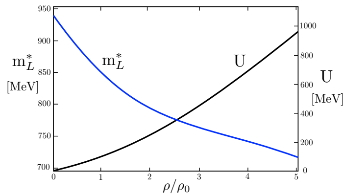
Figure 11. Landau effective mass m_L^*(\rho) = \sqrt{p_F^2 + m^2(\rho)} and potential U(\rho) of quasiparticles representing the median of the posterior distribution of the baryon chemical potential \mu(\rho) (see Figure 3).
