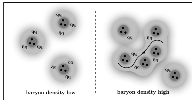
Figure 9. Sketch of low- and high-density baryonic matter. Baryons (e.g. nucleons) are viewed as valence quark cores surrounded by clouds of quark-antiquark pairs (e.g. chiral meson clouds). At densities \rho \gtrsim 2 - 3\rho_0 percolation of quark-antiquark pairs over larger distances starts as indicated. Valence quark cores begin to touch and overlap at baryon densities \rho \gtrsim 5\rho_0 .
