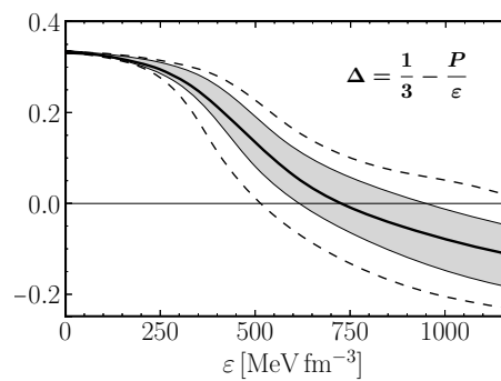
Figure 4. Median and credible bands [27] of the trace anomaly measure, \Delta = \frac{1}{3} - \frac{P}{\varepsilon} , at 68% level (grey band) and 95% level (dashed lines).
