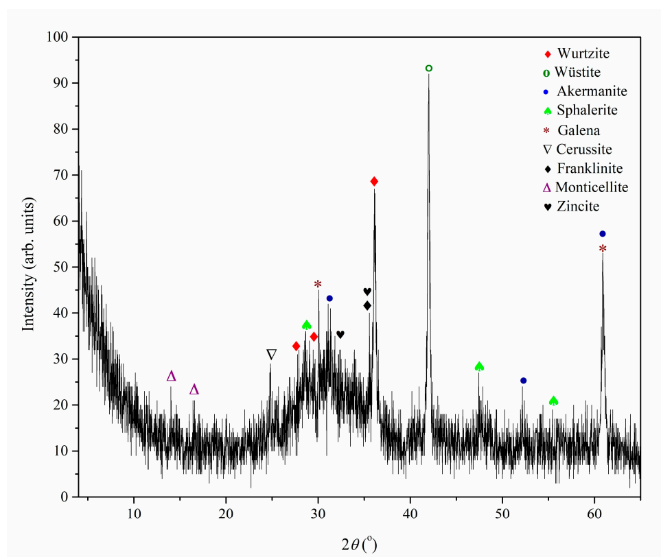
Figure 5. XRD diffractogram of Pb-Zn slag.
