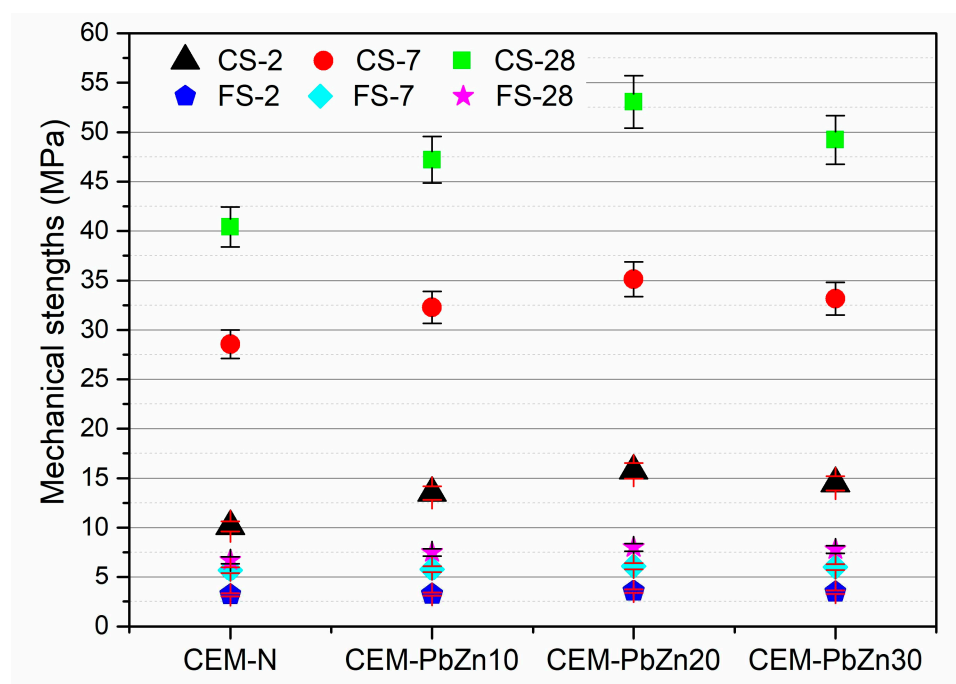
Figure 9. Mechanical strengths of mortar samples.
