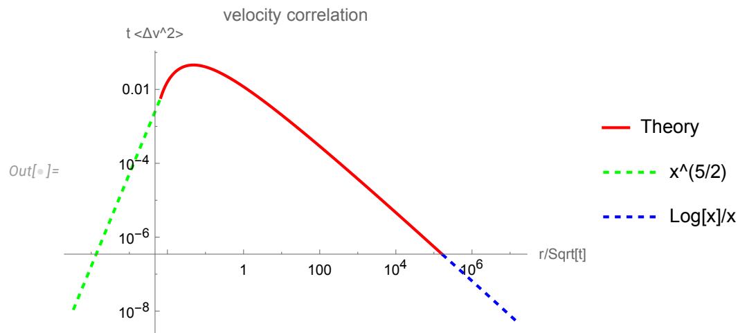
Figure 23. The universal function (265) as a function of x = |\vec{r} - \vec{r}'| / \sqrt{\bar{v}t} . The turnover and subsequent decay are caused by subleading terms in the power expansion starting with x^{5/2} . The next terms involve quantum oscillations manifesting as a turnover from power growth to power decay. Asymptotic decay at large x is \log x/x as it follows from the table (267) of the decay indexes. Thus, the correlation decreases both at large times and at large distances.
