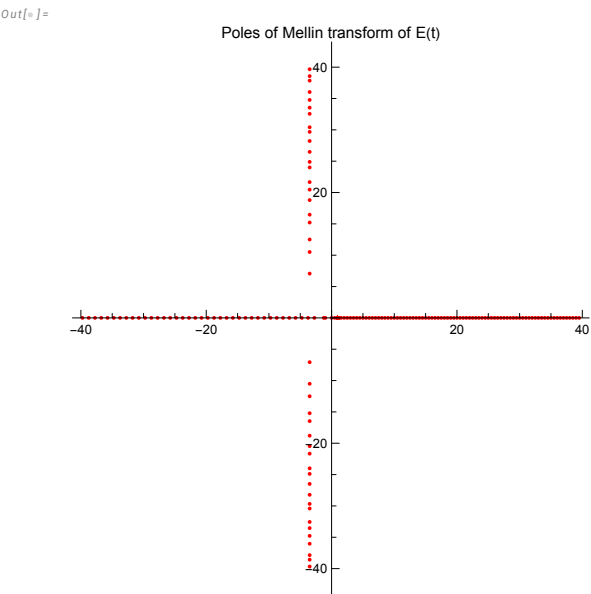
Figure 21. Complex poles of the Mellin transform e(q) of E(t) in (262) defining the spectrum of critical indexes of remaining energy as a function of time.
