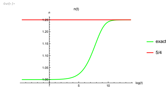
Figure 16. The effective index n(t) = -\frac{t\mathcal{E}(t)}{E(t)} compared with asymptotic value n(\infty) = 5/4 .
