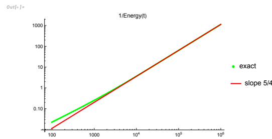
Figure 3. Green curve is the inverse energy 1/E(t) as a function of time. It slowly approaches from above its asymptotic law 1/E(t) \propto t^{5/4} shown in red.
