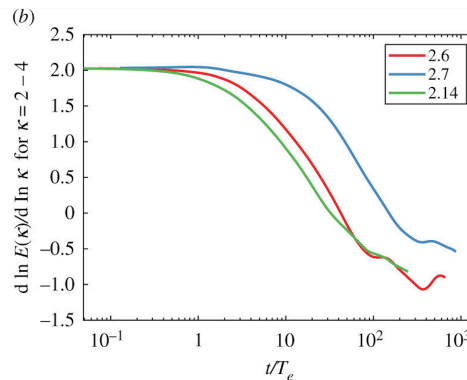
Figure 7. The DNS plot of spectral index \mu(t) = k\partial_k \log E(k, t) as a function of \log t at fixed values of k . The curve goes from \mu = 2 to \mu \approx -1 , which partly overlaps with our theoretical curve in Figure 6. Larger dataset with higher Reynolds numbers is needed for a quantitative match with our theory.
