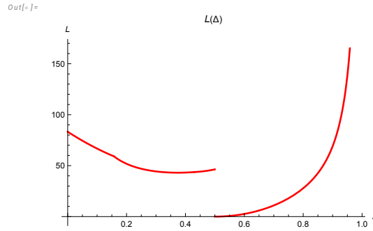
Figure 14. Log plot of L(\Delta) = A_c(r_0(\Delta), \Delta) .
