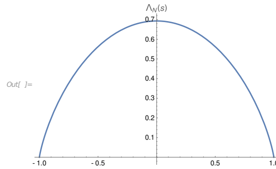
Figure 8. The plot of the function \Lambda(s) . As required, it is positive, takes a maximal value \log(2) at s = 0 , and vanishes at both ends s = \pm 1 of the physical region.
