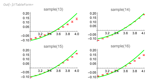
Figure 19. The log plots for the DNS data (red dots) for dimensionless spectrum moments \langle w(p,t) \rangle \pm err , compared with our theory (green line).
