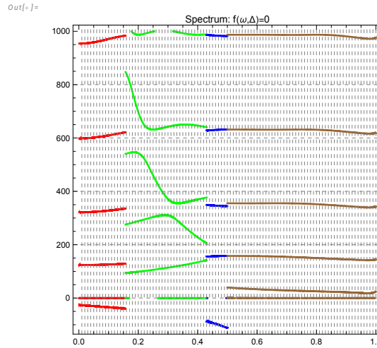
Figure 15. The first levels of the spectrum satisfying equation f(\omega, \Delta) = 0 . The colored lines correspond to four phases. Red: 0 < \Delta < \Delta_1 , Green: \Delta_1 < \Delta < \Delta_2 , Blue: \Delta_2 < \Delta < 1/2 , Brown: 1/2 < \Delta < 1 . The green zone is left as stable, and others are eliminated because r_0(\Delta) < 0 in these zones. Naturally, we eliminate the zero-mode \epsilon_0 = 0 corresponding to translational invariance of the effective Action.
