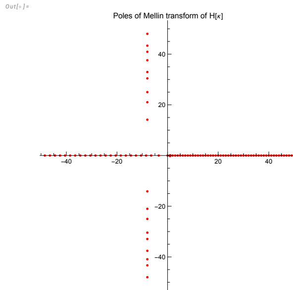
Figure 20. Complex poles of the Mellin transform h(p) of H(\kappa) in (256) defining the critical indexes of the energy spectrum as a function of \kappa = |\vec{k}|\sqrt{\nu t} .
