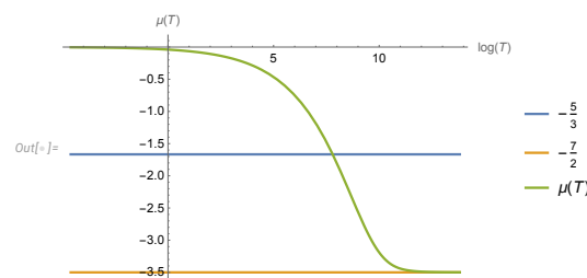
Figure 6. The theoretical plot of effective spectral index \mu(T) = k \partial_k \log E(k, t) as a function of T = k^2 \nu t . It starts at 0 and goes down to the limit -7/2 . The DNS plot Figure 7 starts higher, at \mu = 2 , then goes down and stops at approximately -1 for accessible decay time t . The part from -0.5 to -1 qualitatively matches our curve, but clearly, more data at higher Reynolds numbers is required to verify this prediction of our theory.
