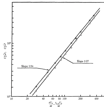
Figure 2. The experimental data [1] for decaying turbulence behind the oscillating grid. The two lines correspond to log-log plots of 1/v_{\perp}^2, 1/v_{\parallel}^2 for the flow behind the grid. The total inverse kinetic energy iK = 2/(v_{\perp}^2 + v_{\parallel}^2) , would have the the mean slope (1.24 + 1.27)/2 \approx 1.255 \pm 0.02 in agreement with our prediction n(\infty) = \frac{5}{4} . This plot was shown by K.R.Sreenivasan at the ICTS in Dec'23 in Bangalore, India [5] as the most reliable experimental data. Other measurements and simulations, at different conditions reviewed in [2], provide mismatching data influenced by initial and boundary conditions. The only large-scale DNS [2] covering three time decades yields a close value of 1.27.
