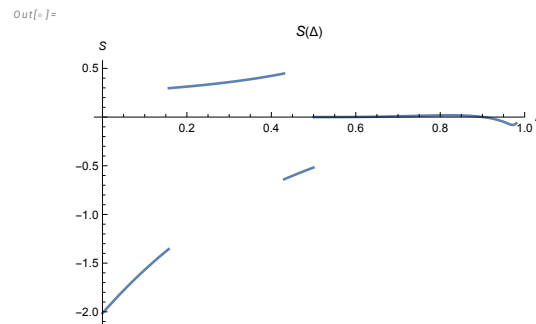
Figure 11. Plot of S(\Delta) .
