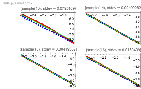
Figure 17. The log-log plots of the DNS data for L(t), E(t) compared with our theory with fitted scales a, b . The thick red line corresponds to the DNS data, the green line is our theory, and the blue dashed line is the asymptotic line with the slope -\frac{5}{2} .
