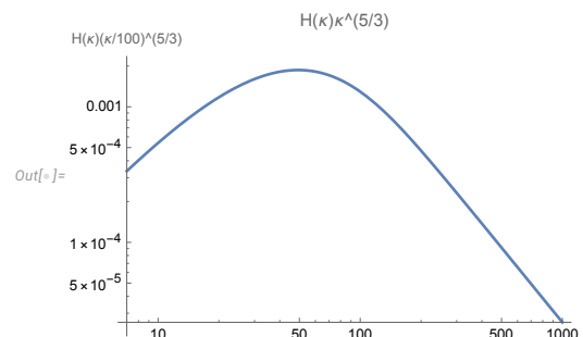
Figure 5. Log-log plot of the universal function H(k)k^{5/3} . It starts growing, reaches the maximum, then turns down, asymptotically decaying as k^{-11/6} . This qualitatively matches the DNS plot at Figure 4. A larger DNS data at higher Reynolds numbers would be required to verify our theory with more precision.
