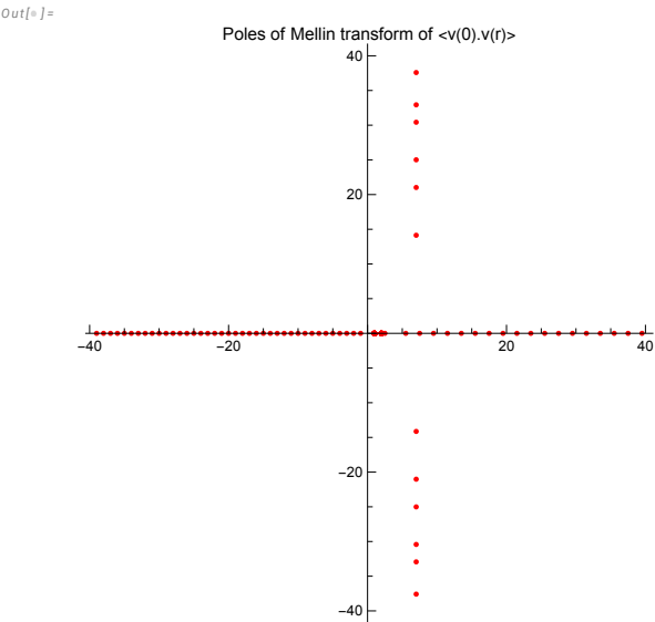
Figure 22. The spectrum of (complex) indexes of the power expansion of the velocity correlation function. The poles in the right semiplane determine the small-distance expansion of the correlation function \vec{v}(0) \cdot \vec{v}(r) \sim \sum_n O_n |\vec{r}|^{p_n} .
