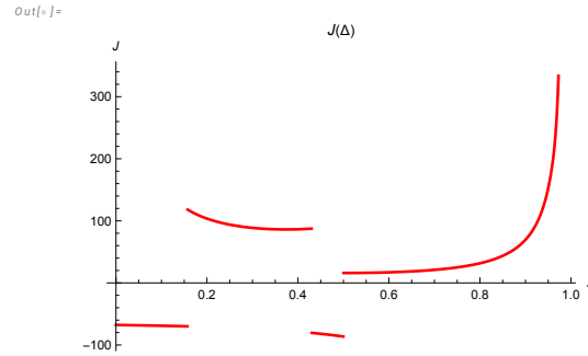
Figure 13. Plot of universal function J(\Delta) . the four curves correspond to four phases (solutions for r_0(\Delta) ).
