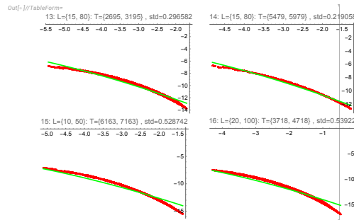
Figure 18. The log-log plot of the mid-range of the DNS data [2] for energy spectrum E(k,t)\sqrt{t} = F(k\sqrt{t}) at mid-range of decay times, fitted by our theory (green line) with variable scales of the energy and wavevectors
