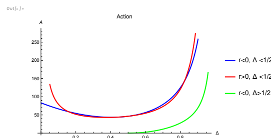
Figure 12. Plot of A_c(r_0(\Delta), \Delta) for the three real solutions of the equation g(r, \Delta) = 0 . At \Delta = \Delta_1 and \Delta = \Delta_2 , the action curves intersect; at \Delta = 1/2 , there is a gap between the lowest action ( = 0 ) and the lowest of the other two. So, there are second-order phase transitions at \Delta_1, \Delta_2 and the first-order phase transition at \Delta = 1/2 .
