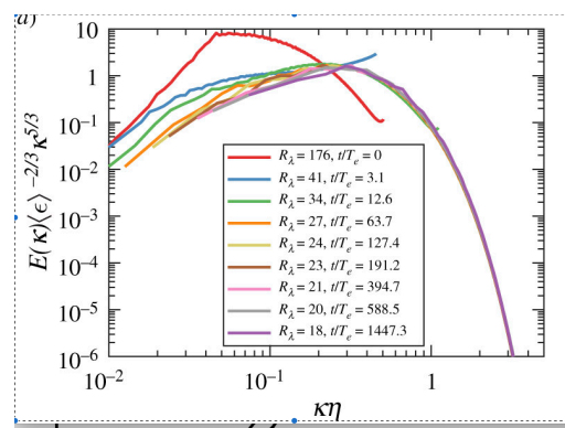
Figure 4. The log-log plot of deviation from K41 energy spectrum in decaying turbulence, taken from [2] with permission of the author. The observed curve approximately matches our theoretical curve in Figure ???. The K41 spectrum would correspond to a horizontal line, a total mismatch.
