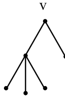
Figure 1. The tree T which is used in the following example.
