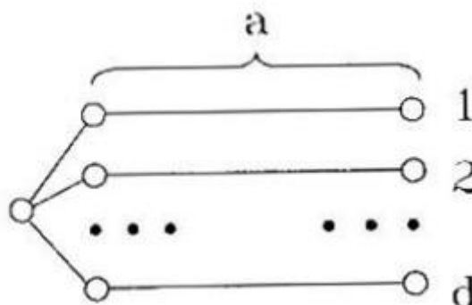
Figure 4. The tree H (Subdivisions of star graph).
