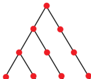
Figure 3. The tree S for n=4 .
