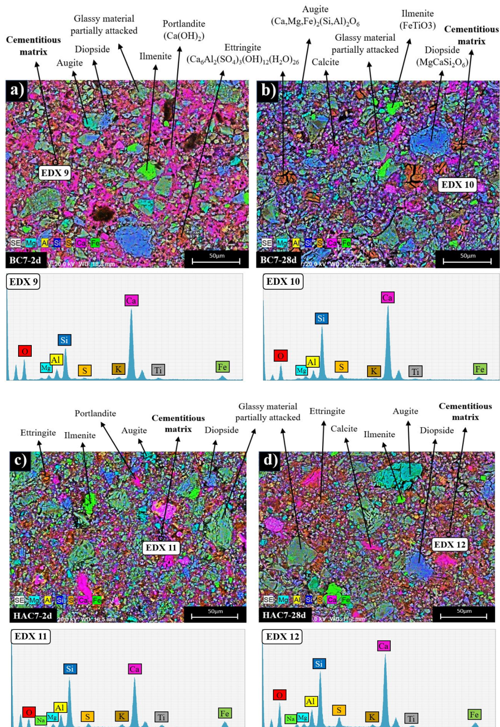
Figure 10. BSEM micrography of (a) BC-7 after 2 days of curing (x500), (b) BC-7 after 28 days of curing (x500), (c) HAC-7 after 2 days of curing, (d) HAC-7 after 28 days of curing (x500).
