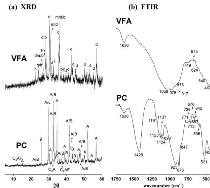
Figure 3. (a) XRD patterns and (b) FTIR spectra of PC and VFA. Legend: d: diopside ( \text{MgCaSi}_2\text{O}_6 ) (COD 9004319); a: augite ( (\text{Ca,Mg,Fe})_2(\text{Si,Al})_2\text{O}_6 ) (COD 9006247); q: cristobalita ( \text{SiO}_2 ) (COD 9001578); m: magnetite ( \text{Fe}_2\text{O}_3 ) (COD 9006247); b: bytownita ( (\text{Ca,Na})(\text{Si,Al})_4\text{O}_8 ) (COD 9011200); i: ilmenita ( \text{FeTiO}_3 ) (COD 9000910); py: pyroxene ( \text{Fe}_{0.44}\text{Mg}_{0.56}\text{SiO}_3 ) (COD 9001577); A: alita ( 3\text{CaO}\cdot\text{SiO}_2 ) (COD 1540705); B: belita ( 2\text{CaO}\cdot\text{SiO}_2 ) (COD 9012793); C 3 A: aluminato tricálcico ( 3\text{CaO}\cdot\text{Al}_2\text{O}_3 ) (COD 9014359); C 4 AF: ferritos ( 4\text{CaO}\cdot\text{Al}_2\text{O}_3\cdot\text{Fe}_2\text{O}_3 ) (COD 9015955); g: anhidrite ( \text{CaSO}_4 ) (COD 5000040); c: calcite ( \text{CaCO}_3 ) (COD 9016022).
