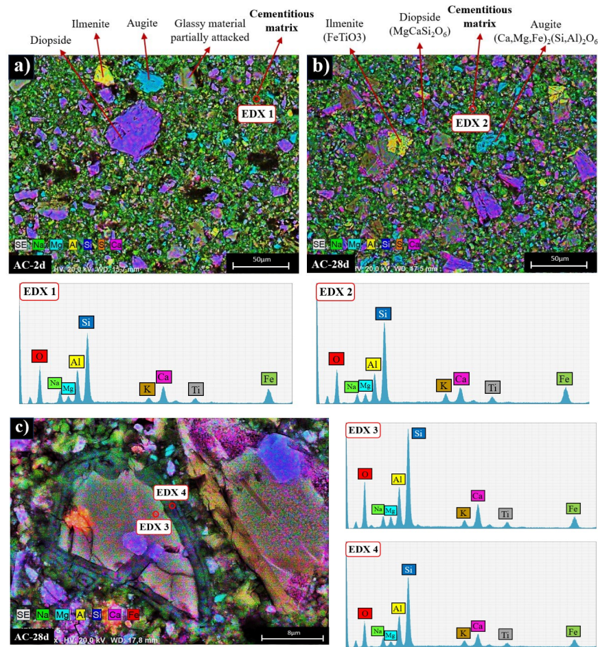
Figure 8. BSEM micrography of (a) AC after 2 days of curing (x500), (b) AC after 28 days of curing (x500), (c) partially attacked VFA particle in AC 28d (x3000).
