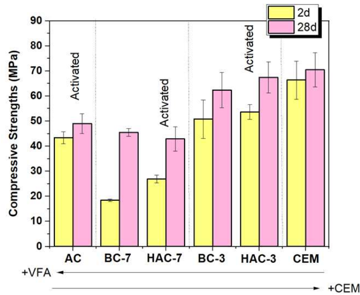
Figure 4. Compressive strengths (MPa) for the all pastes CEM, BC, HAC and AC cements.
