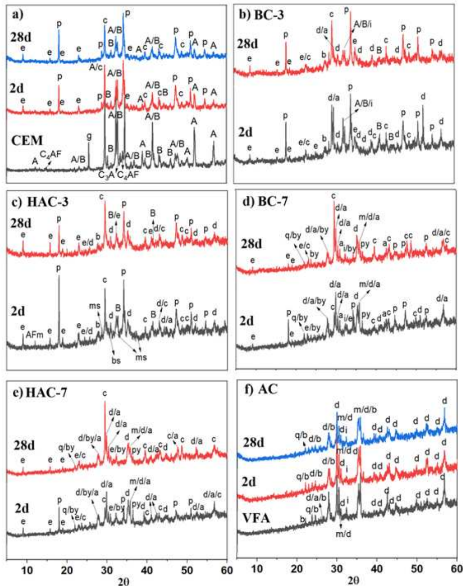
Figure 5. XRD patterns of (a) CEM, (b) BC-3, (c) HAC-3, (d) BC-7, (e) HAC-7, (f) AC, after 2 and 28 days of curing. Legend: d: diopside ( \text{MgCaSi}_2\text{O}_6 ); a: augite ( (\text{Ca,Mg,Fe})_2(\text{Si,Al})_2\text{O}_6 ); q: cristobalite ( \text{SiO}_2 ); b: bytownite ( ((\text{Ca,Na})(\text{Si,Al})_4\text{O}_8) ); i: ilmenite ( \text{FeTiO}_3 ); A: alite ( 3\text{CaO}\cdot\text{SiO}_2 ); B: belite ( 2\text{CaO}\cdot\text{SiO}_2 ); \text{C}_3\text{A} : tricalcium aluminate; e: ettringite ( \text{Ca}_6\text{Al}_2(\text{SO}_4)_3(\text{OH})_{12}(\text{H}_2\text{O})_{26} ) (COD 9015084); p: portlandite ( \text{Ca}(\text{OH})_2 ) (COD 1008780); c: calcite ( \text{CaCO}_3 ); AFm: ( (3\text{CaO}\cdot\text{Al}_2\text{O}_3\cdot\text{CaSO}_4\cdot 12\text{H}_2\text{O}) ) (COD 9013423), bs: basanite ( \text{Ca}_3\text{H}_3.6\text{O}_{13.8}\text{S}_3 ) (COD 9012211), ms: magnesium silicate ( \text{MgSiO}_3 ) (COD 9016052).
