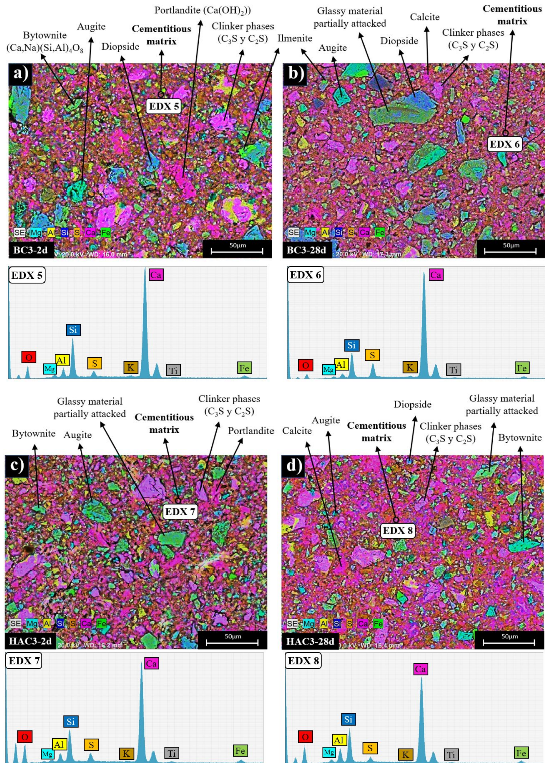
Figure 9. BSEM micrography of (a) BC-3 after 2 days of curing (x500), (b) BC-3 after 28 days of curing (x500), (c) HAC-3 after 2 days of curing, (d) HAC-3 after 28 days of curing (x500).
