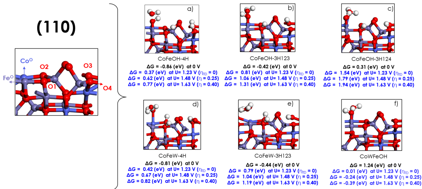
Figure S6. Off-stoichiometric coverage patterns on CoFe 2 O 4 (110) with (a-e) excess hydrogens on lattice oxygens, and (f) with missing hydrogen. Free energies referenced to the resting states in Figure S5 (m). Energetics with respect to applied potentials ( U = 1.23 V , 1.48 V and 1.63 V) has been reported each converged structure. Oxygen, hydrogen, iron, and cobalt atoms are colored red, white, violet, and indigo blue, respectively.
