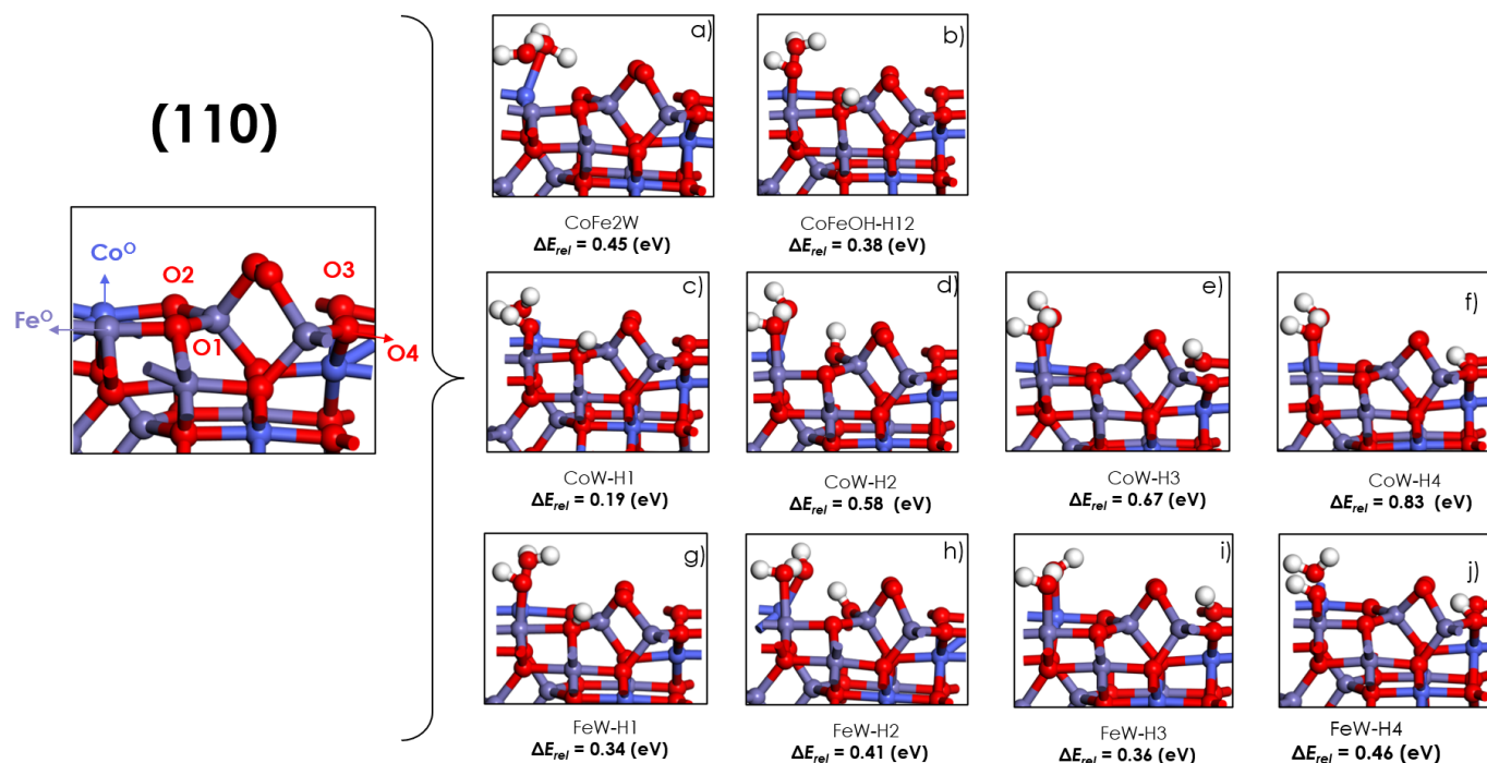
Figure S4. Dissociated water Coverage patterns on CoFe 2 O 4 (110). Oxygen, hydrogen, iron, and cobalt atoms are colored red, white, violet, and indigo blue, respectively.
