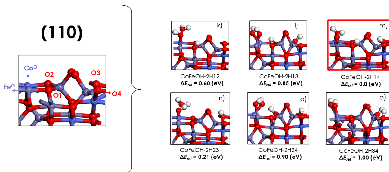
Figure S5. Dissociated water Coverage patterns on CoFe 2 O 4 (110). Oxygen, hydrogen, iron, and cobalt atoms are colored red, white, violet, and indigo blue, respectively.
