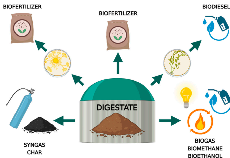
Figure 2. Application of the digestate produced in an agricultural biogas plant.
