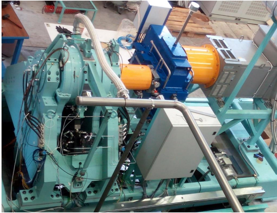
Figure 6. Photograph of experimental apparatus for testing full scale pad journal bearings.
