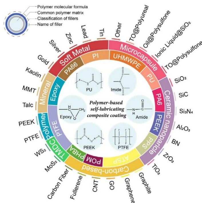
Figure 4. Common matrices and fillers of polymer composite coating. From [29].
