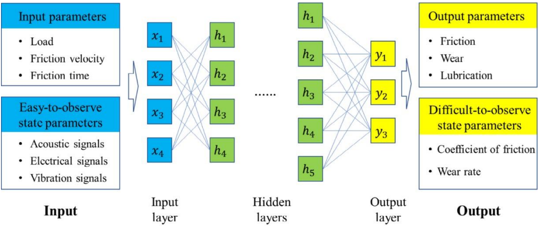
Figure 10. Application of ANN methods in tribology research. From [57].
