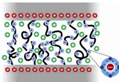
Figure 5. Illustrating schematically the origin of the lubrication by charged brushes. From [36].
