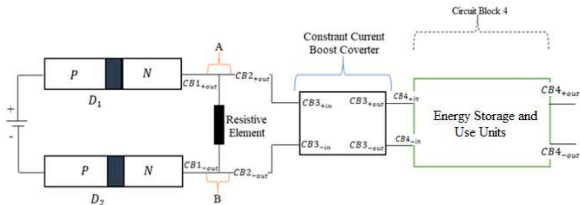
Figure 4. Circuit Block 4 Configuration-Energy Storage and Potential Recharging System (Circuit Block 4 serves as a crucial interface in the energy conservation process, capturing output power from Circuit Block 3 and overseeing its efficient utilization).
