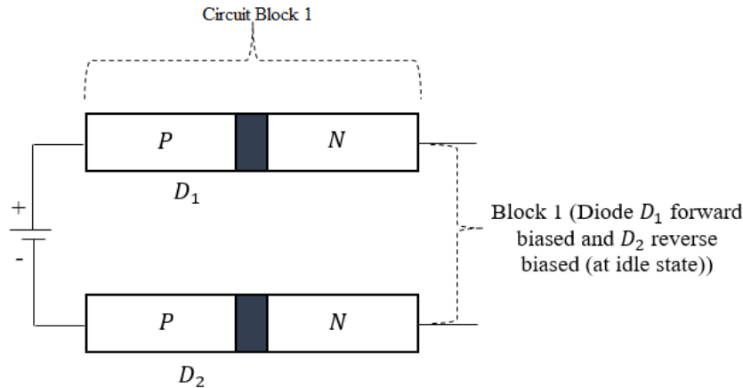
Figure 1. Operational Principle of Circuit Block 1-Diode Configuration. (The diodes ( D_1 and D_2 ) are configured in parallel with the specific arrangement to prevent undesired backflow of short circuit current from Circuit Block 2. As the short circuit current attempts to flow in reverse, the diodes transition to a reverse-biased mode, widening the depletion region and increasing resistance, acting as a barrier to the reverse flow. The block diagram illustrates the parallel connection of diodes).
