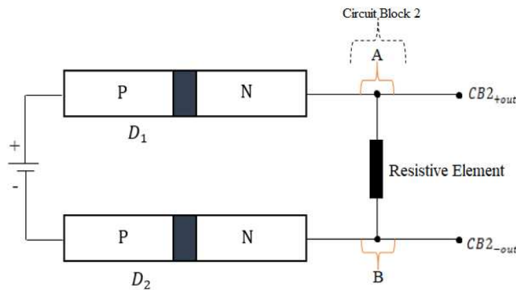
Figure 2. Circuit Block 2-Short Circuit Power Harnessing. (Circuit Block 2 illustrates the innovative approach to energy conservation and utilization).
