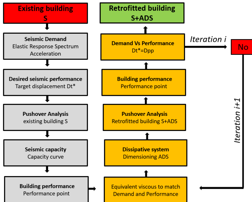
Figure 5. Design Procedure of Additional Dissipative Structures (ADS): Flow-chart.
