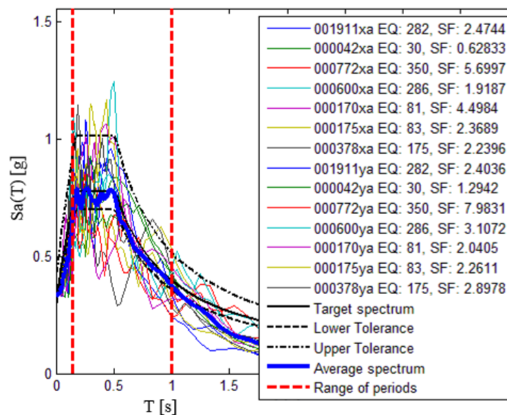
Figure 11. REXEL data selection: selected record response spectrum.
