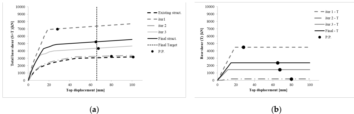
Figure 8. Variation of global response S+ADS (cumulative base shear-top displacement) and contribution of the dissipative towers T (towers base shear-top displacement).
