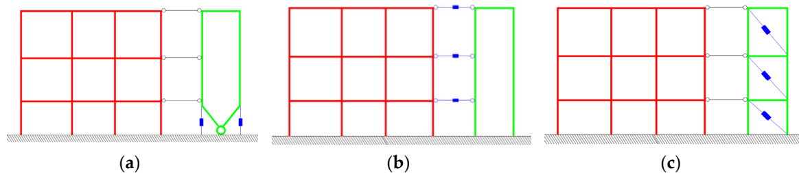
Figure 2. Possible configurations of dissipative devices of the ADS: (a) at the hinge of a tower, (b) at each connection between S and contrast structure, (c) as dissipative braces inside framing system.
