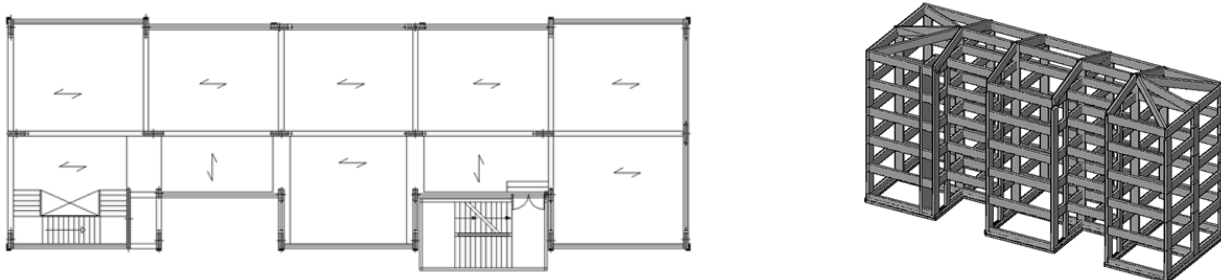
Figure 6. Planar and 3D view of the existing building.
